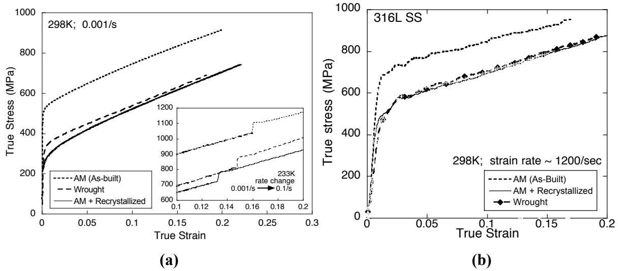
Fig. 3. Compressive a) quasi-static and b) dynamic SHPB, true stress-true strain responses of 316L SS in the AM-as-built condition, AM + recrystallization heat-treatment, and annealed wrought 316L SS.
