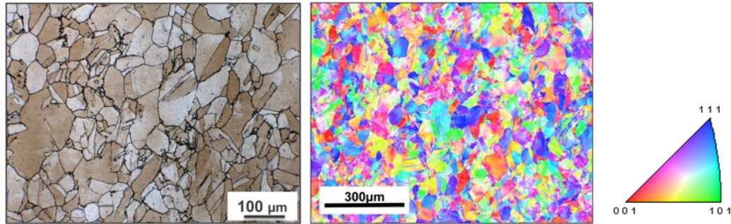
Figure 7 : Optical metallography and EBSD map of wrought 304L SS.
