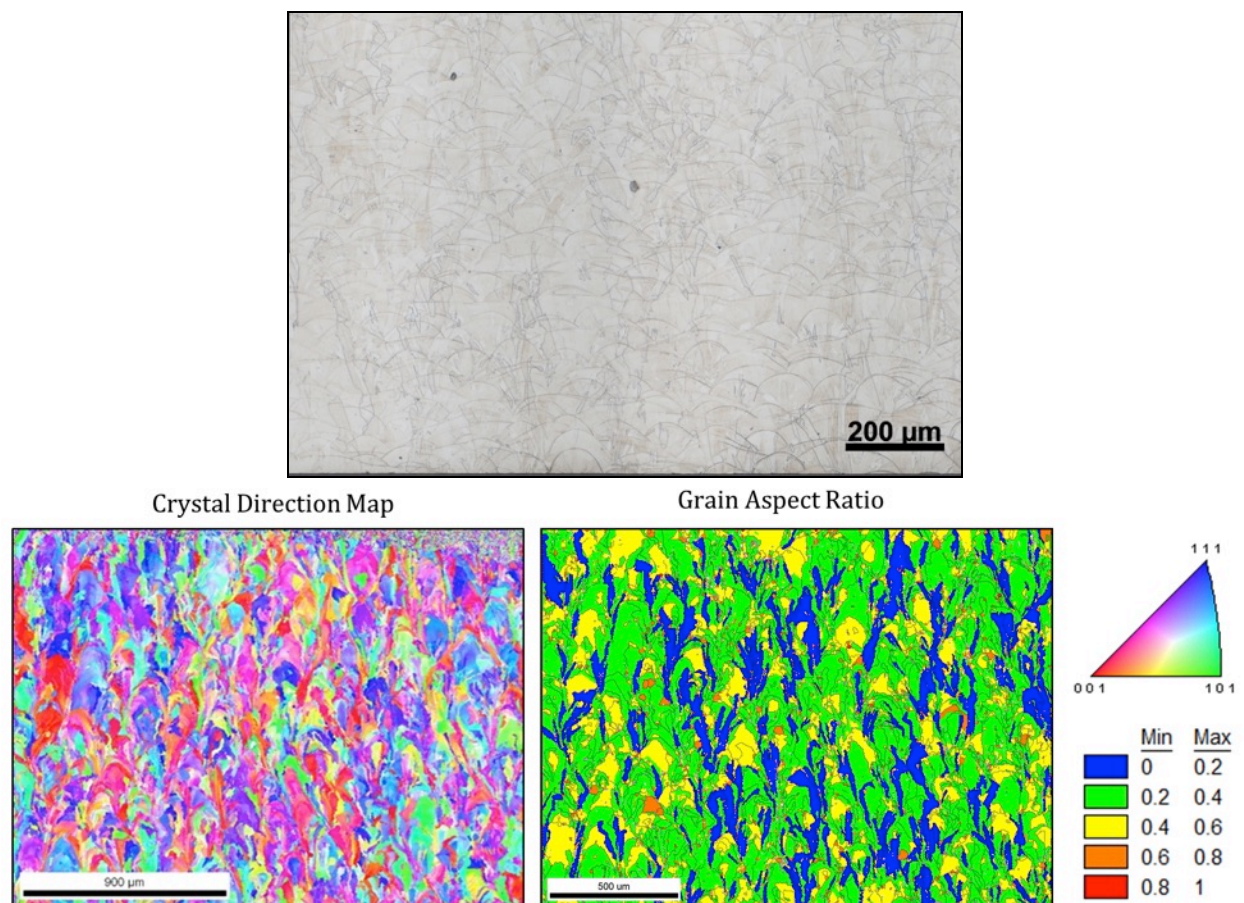
Figure 6 : Optical metallography and EBSD scan of 304L SS microstructure produced on the EOS machine using the pedigreed ADET (low sulfur) powder.
