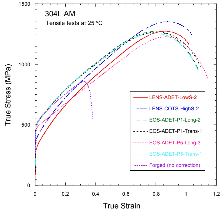
Figure 9 : Tensile stress-strain response of the LENS and EOS – AM 304L SS materials produced with the ADET (low sulfur) and COTS(high sulfur) powders compared to that of forged wrought 304L SS
