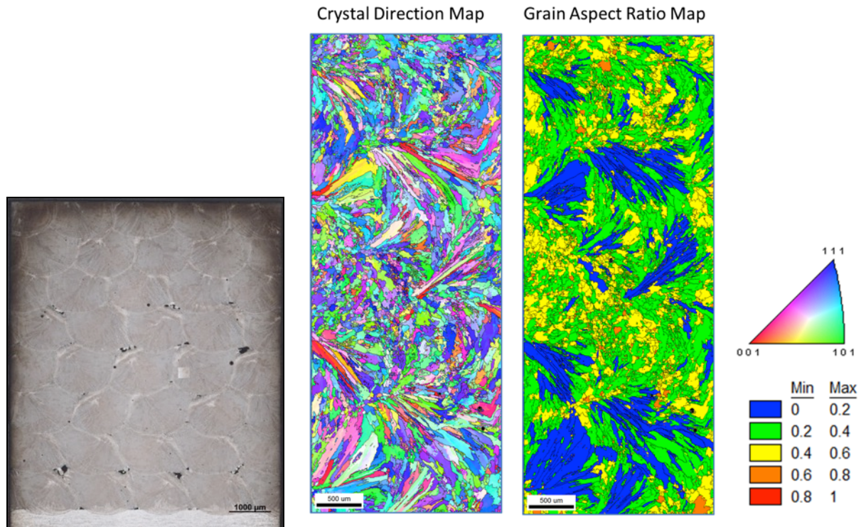
Figure 4 : Optical metallography and EBSD scan of 304L SS microstructure produced using a LENS additive process using the pedigreed ADET (low sulfur) powder.
