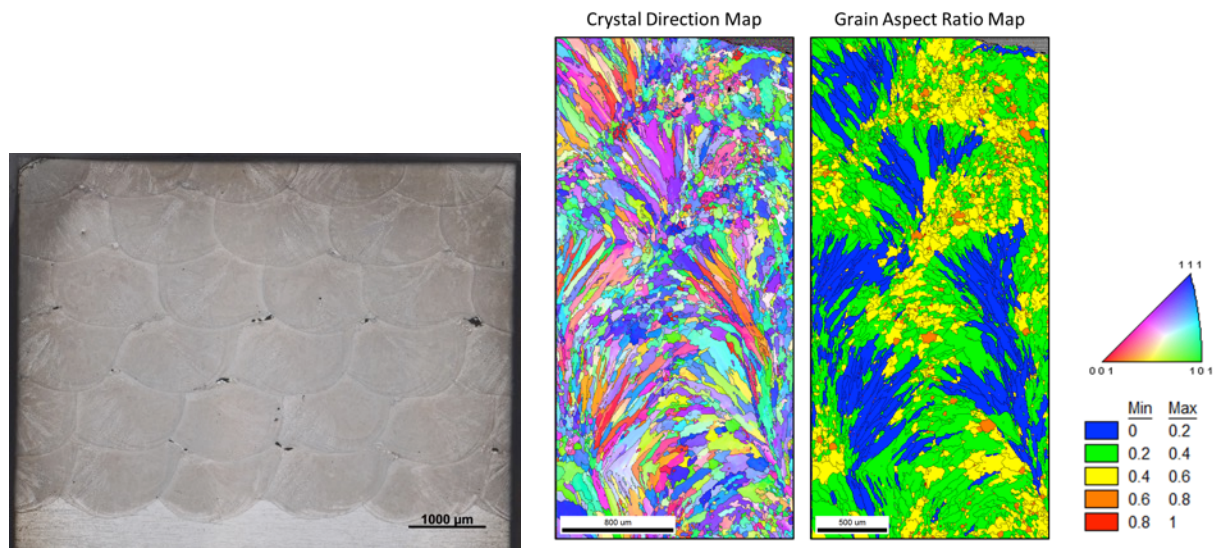
Figure 5 : Optical metallography and EBSD scan of 304L SS microstructure produced on the LENS machine using the COTS (high sulfur) powder.
