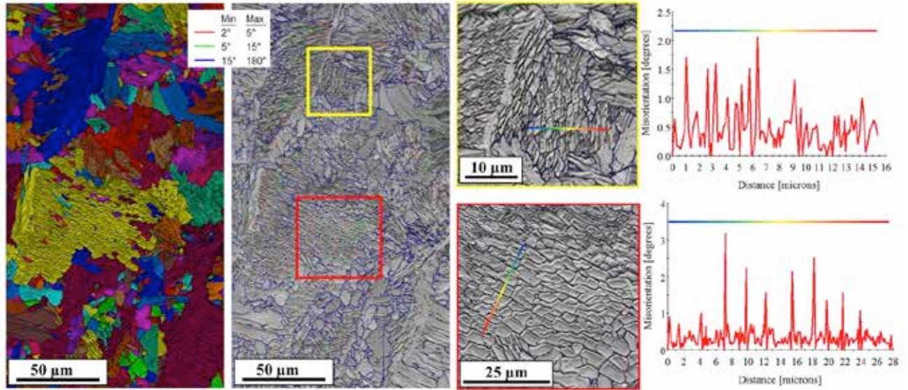
Fig. 4. 316L AM microstructure showing unique grain color map (left), boundary type maps (center), and misorientations along rainbow-colored lines showing dendritic spacing.
