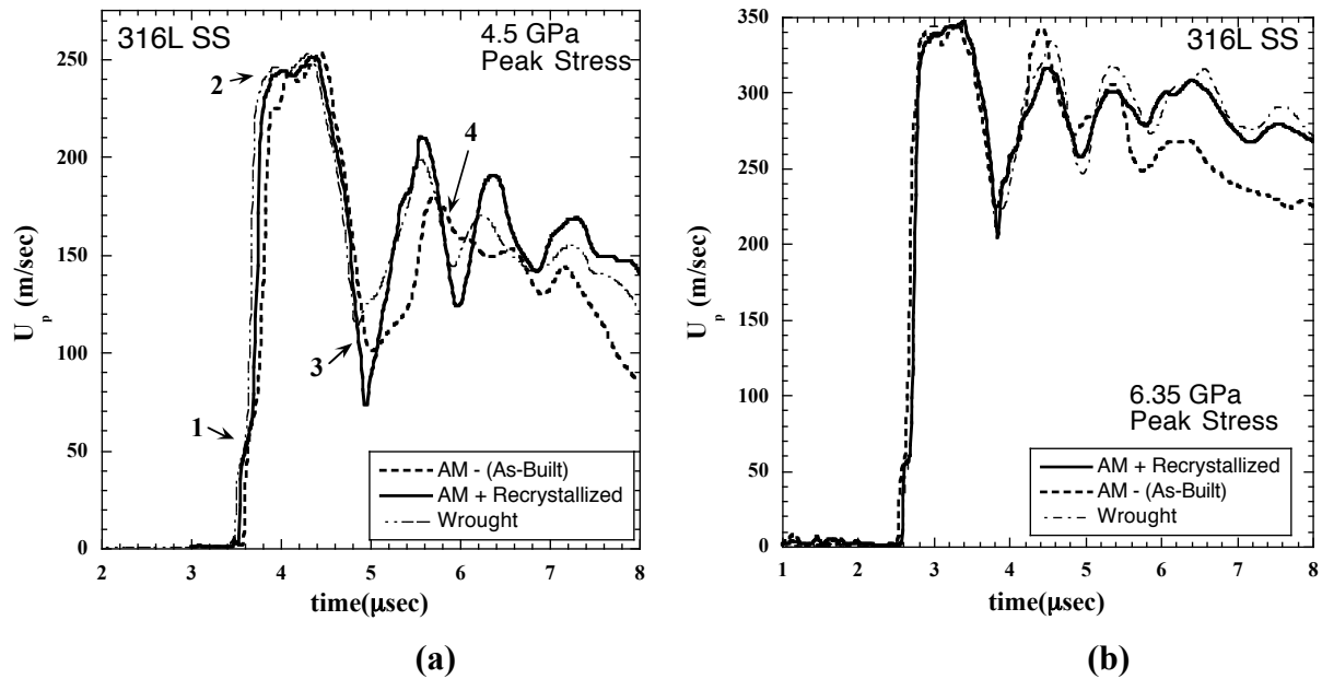
Fig. 5. PDV wave profiles (particle velocity versus time plots) for the three 316L SS materials impacted at peak stresses of a) 4.5 and b) 6.35 GPa.
