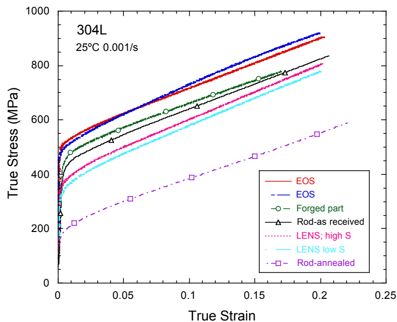
Figure 8 : Compressive stress-strain response of the LENS and EOS – AM 304L SS materials compared to that of forged wrought and Annealed wrought rod stock 304L SS
