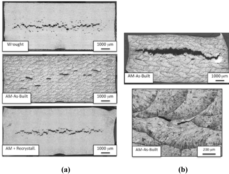
Fig. 6. Macroscopic optical metallography 316L SS in the AM-as-built condition, AM + Rx, and annealed wrought 316L SS following a) peak shock stress loading to 4.5 GPa causing incipient damage, and b) shock loading to peak stress of 6.35 GPa resulted in nearly full spall in the AM-As-Built sample and full sample fracture (complete spall) in AM-As-Built and AM+Recrystallization (details in Figure 7b).
