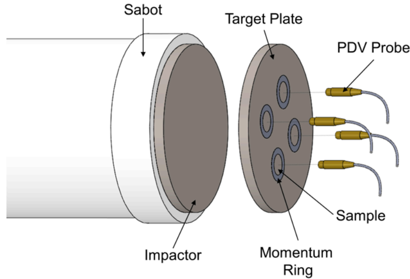
Figure 10. Experimental configuration used to produce incipient damage or complete spall in the four 304L SS samples simultaneously. Wrought 304L SS impactors were accelerated in an 80 mm gas gun and impacted onto the target to produce the peak shock stress studied. PDV probes were positioned to view the center of each sample to provide free-surface velocimetry data from each of the four samples in each spallation experiment.
