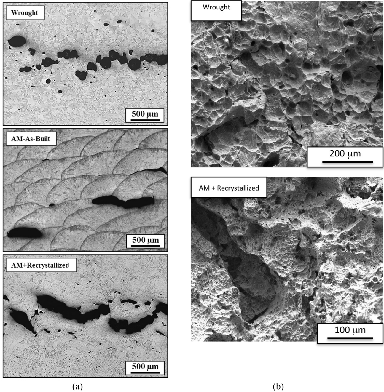
Fig. 7. (a) Higher magnification optical micrographs of damage evolution in incipiently spalled 316L SS in the AM-as-built condition, AM+Rx, and annealed wrought 316L SS following 4.5 GPa spall test, and (b) Scanning-Electron Micrographs of ductile fractures in wrought and AM + recrystallized conditions following spallation loading to 6.35 GPa.
