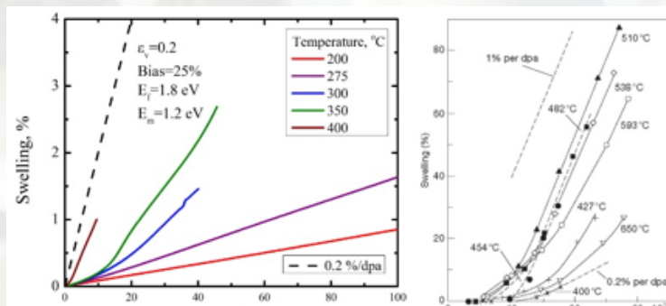
Figure 6: Modeled swelling (left) in 20% cold worked 316 stainless steel as a function of dose taking into account concurrent nucleation of vacancy and interstitial type loops, and experimental data (right) from the EBR-II fast reactor [data from Garner and Gelles].
