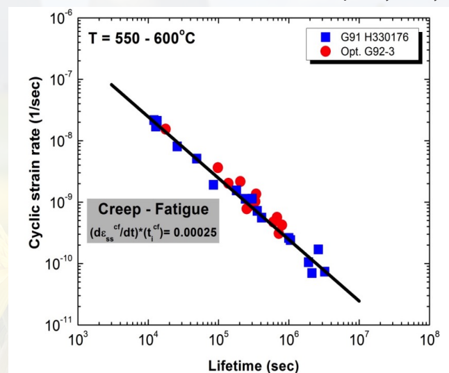
Figure 1: A new creep-fatigue correlation for Grade 91 and optimized Grade 92 steels
