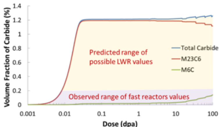
Figure 7: The evolution of total carbide ( M_{23}C_6 + M_6C ) volume fraction under LWR conditions (275 °C and 7 \times 10^{-8} dpa/s).
