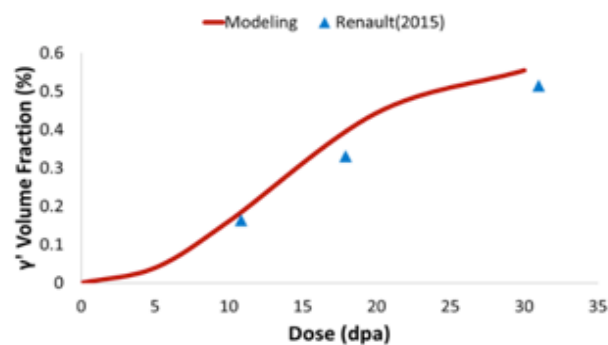
Figure 8: Comparison of modeled \gamma' development to experimental data in cold worked 316 stainless (390°C at 9.4 \times 10^{-7} dpa/s).
