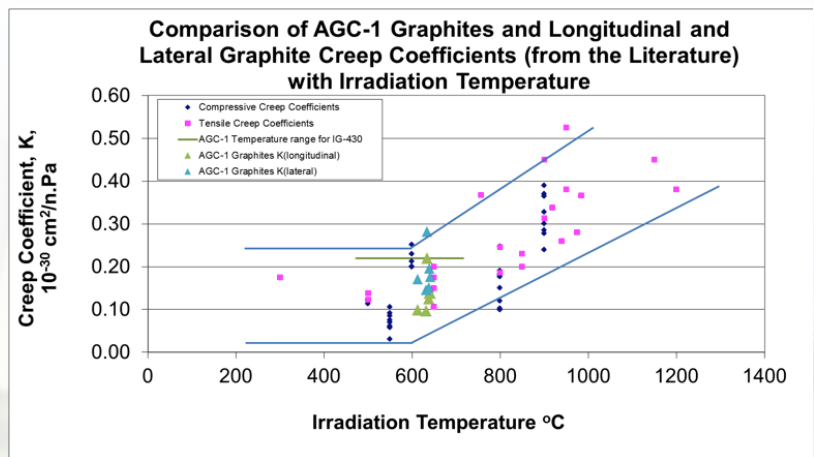
Figure 3: Irradiation Creep measured in AGC-1 Graphites compared to creep measurements in the literature.
