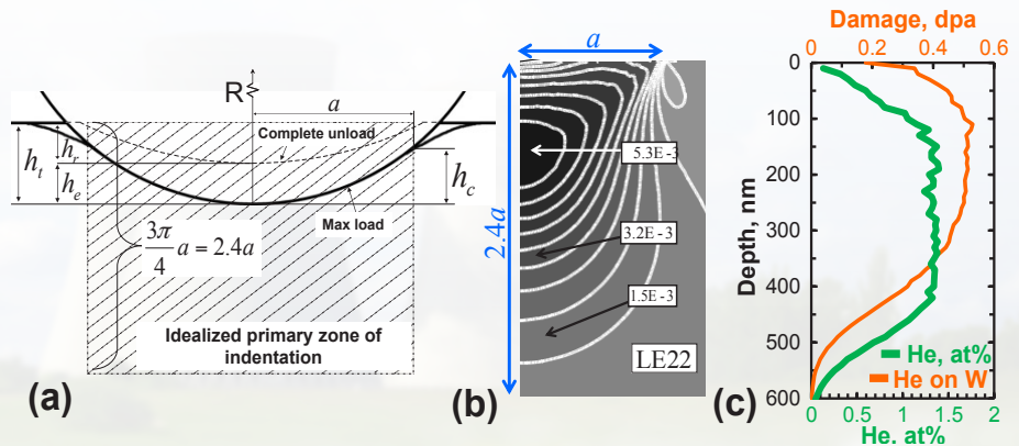
Figure 4: (a) Schematic of spherical indentation showing the idealized primary zone of indentation. (b) Logarithmic strain field (along the indentation direction) for a spherical indenter in the indentation zone ( \sim 2.4a , where a is the contact radius) close to the indentation yield. Both the contact radius a , and hence the volume probed by indentation, can be controlled with a proper choice of indenter radii. This approach is thus ideally suited for measuring any mechanical changes in the modified material surface layers, such as probing the (c) damage caused by He irradiation on a tungsten sample.
