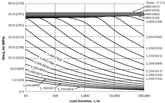
Figure 2 : Time dependent allowable design stresses for Alloy 617 from the draft code case.
