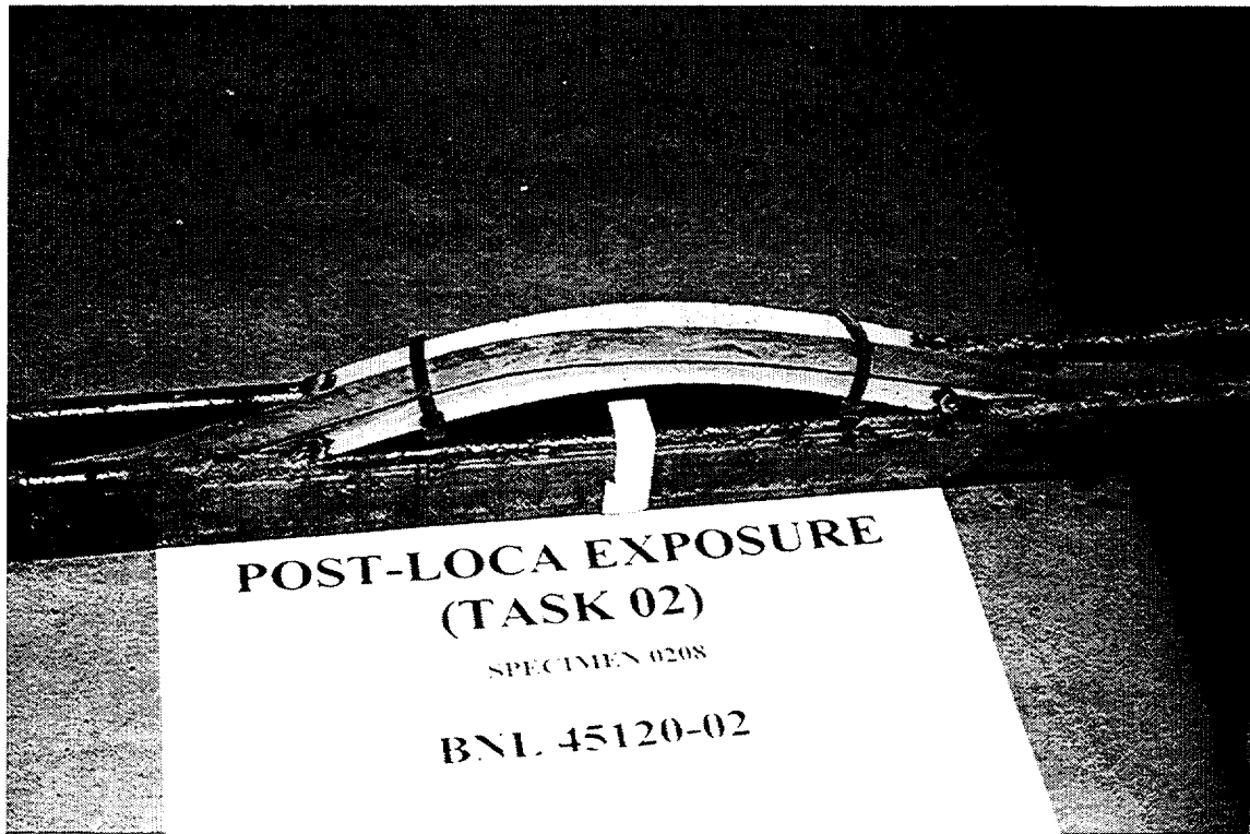
Figure 3.15 Post-LOCA condition of AIW specimen 0208 from Group 2.3 (naturally aged 24 years)
