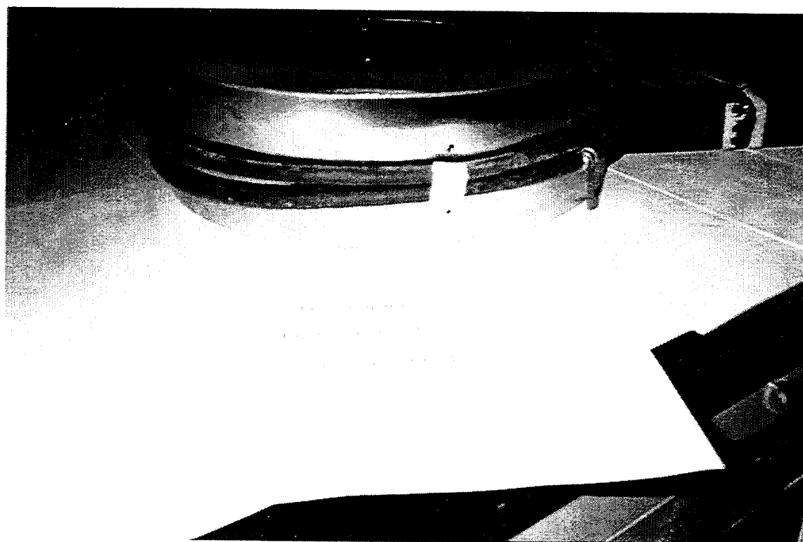
Figure 3.34 AIW specimen 0611 from Group 6.2 (pre-aged to 60 years) after accelerated service aging
