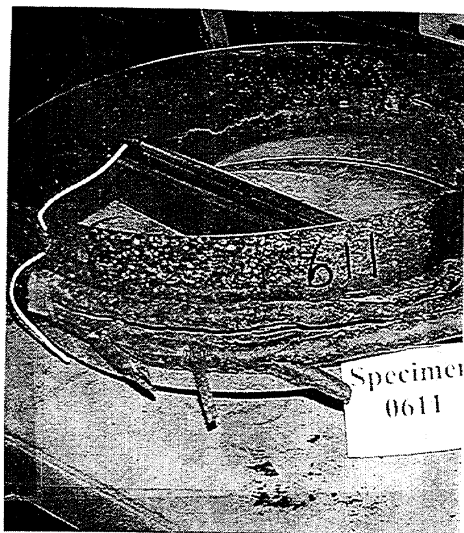
Figure 3.40 Post-LOCA condition of AIW specimen 0611 from Group 6.2 (pre-aged to 60 years)
