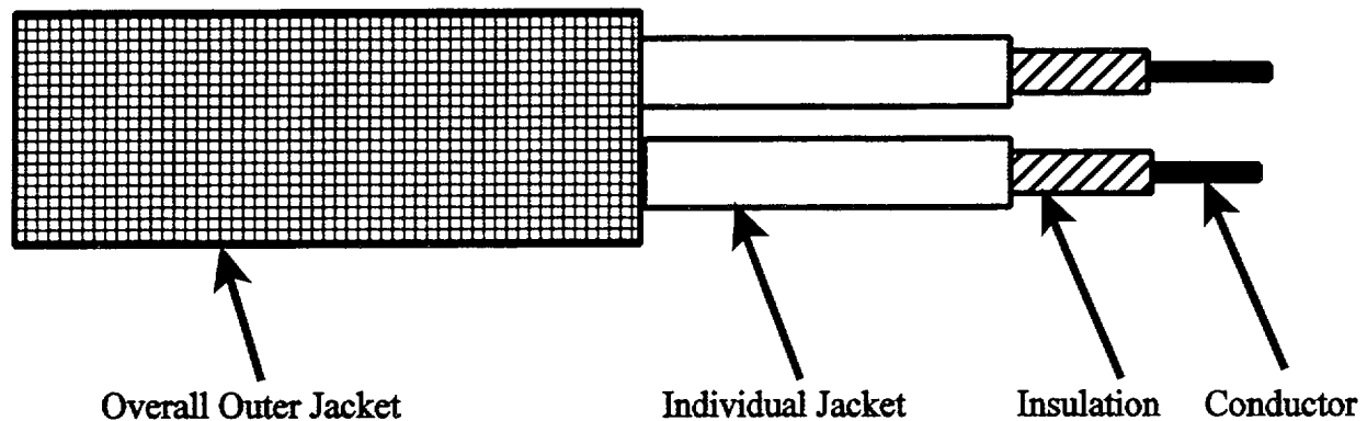
Figure 3.10 Typical sub-components of EPR/Hypalon® cables
