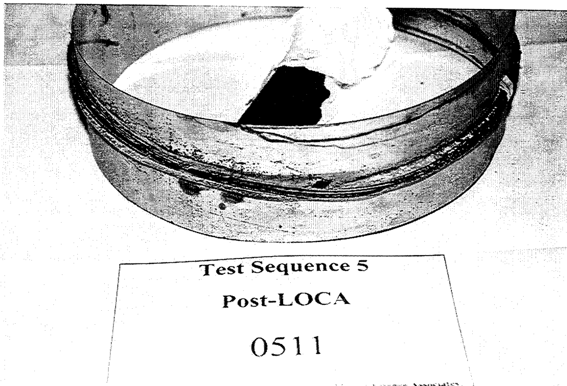
Figure 3.31 Post-LOCA condition of Okonite specimen 0511 in Group 5.3 (pre-aged to 40 years)
