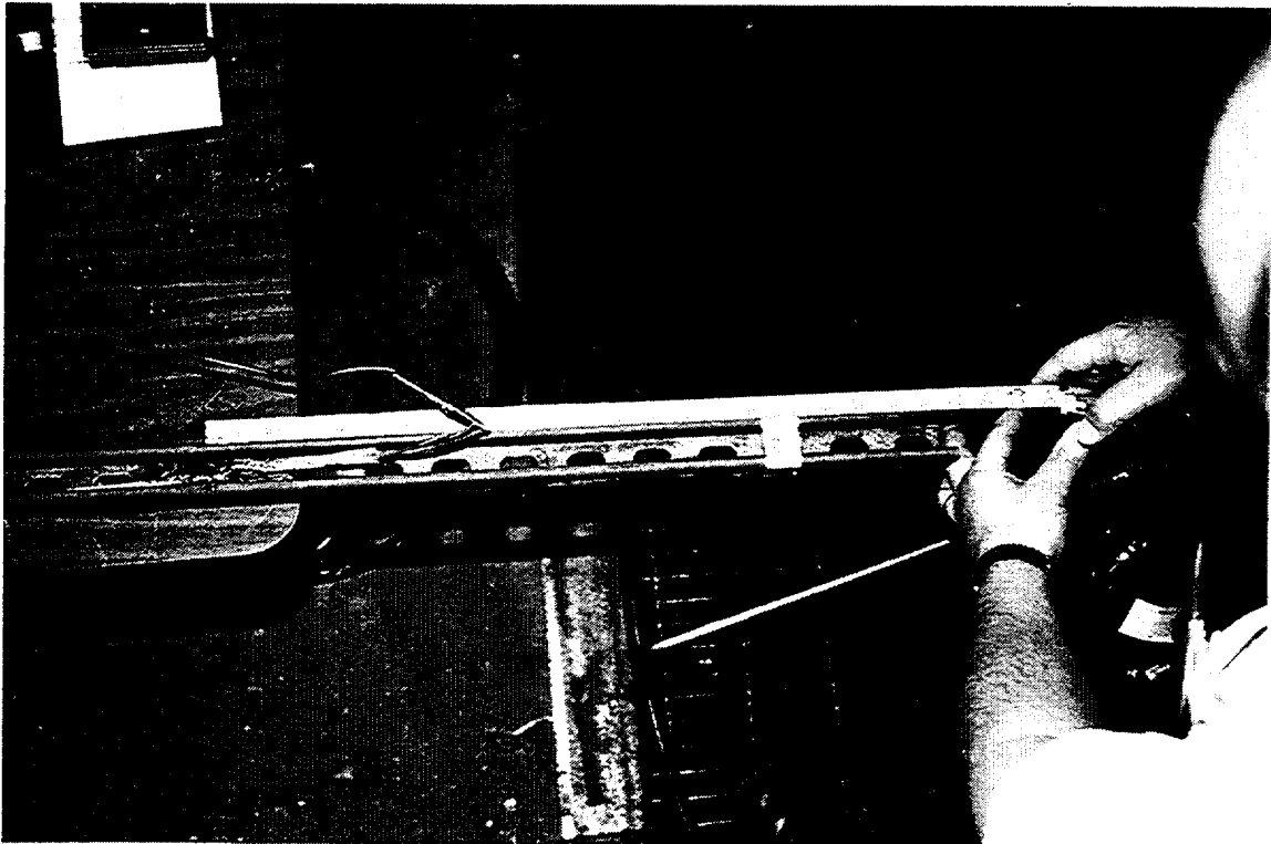
Figure 3.18 Specimen 0313 fault location near outboard cable tie
