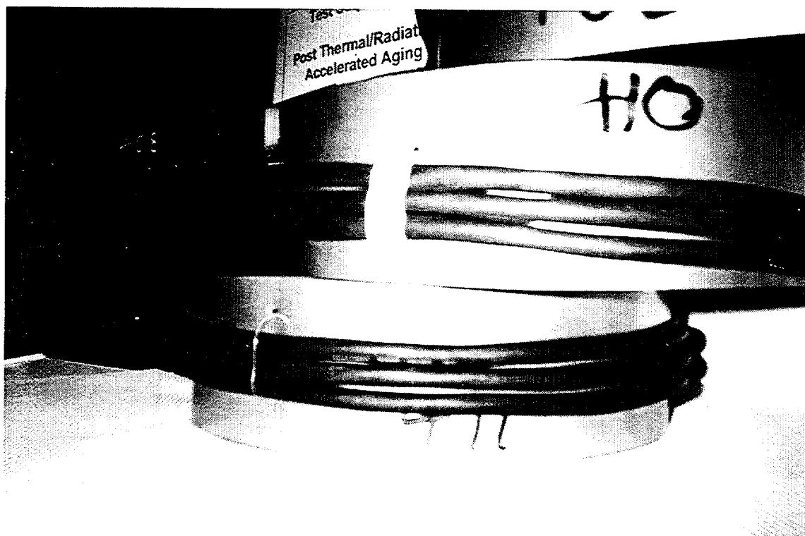
Figure 3.20 Anaconda multiconductor specimens 0410 and 0411 from Group 4.3 (pre-aged to 40 years) after accelerated service aging
