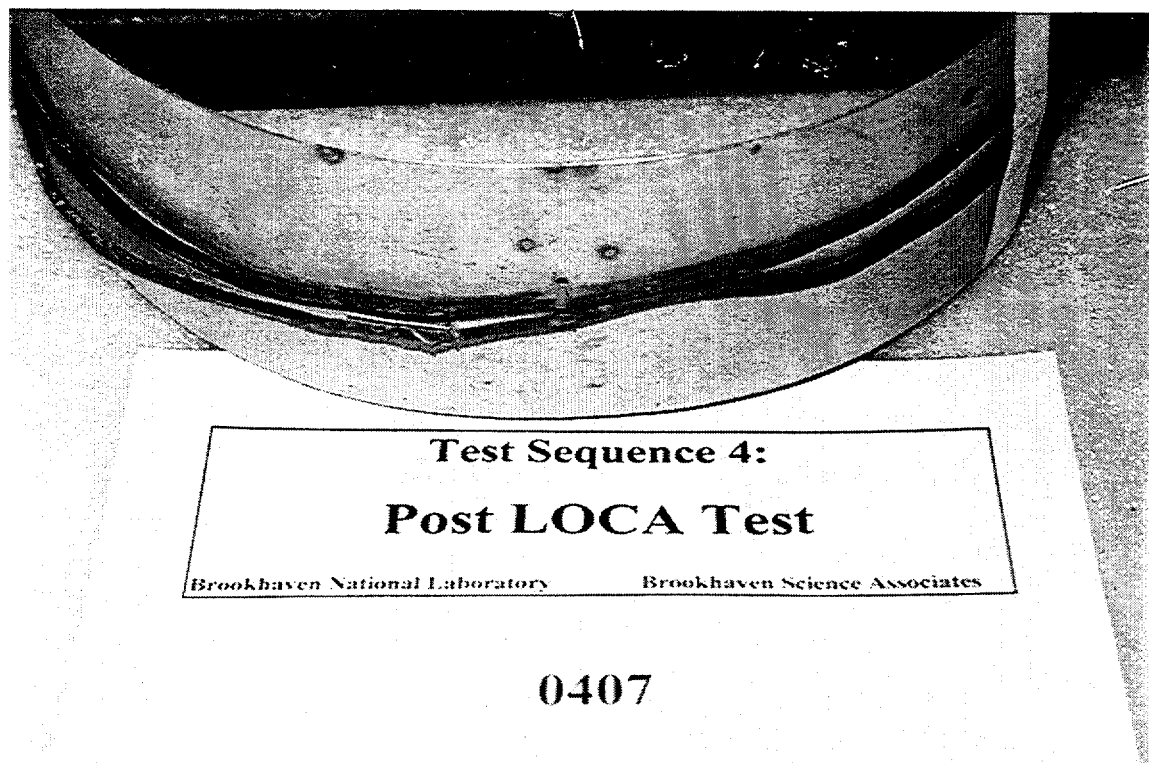
Figure 3.26 Post-LOCA condition of Anaconda single conductor specimen 0407 from Group 4.3 (pre-aged to 40 years)
