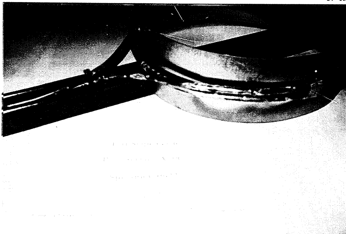
Figure 3.35 Rockbestos specimen 0622 from Group 6.2 (pre-aged to 60 years) after accelerated service aging
