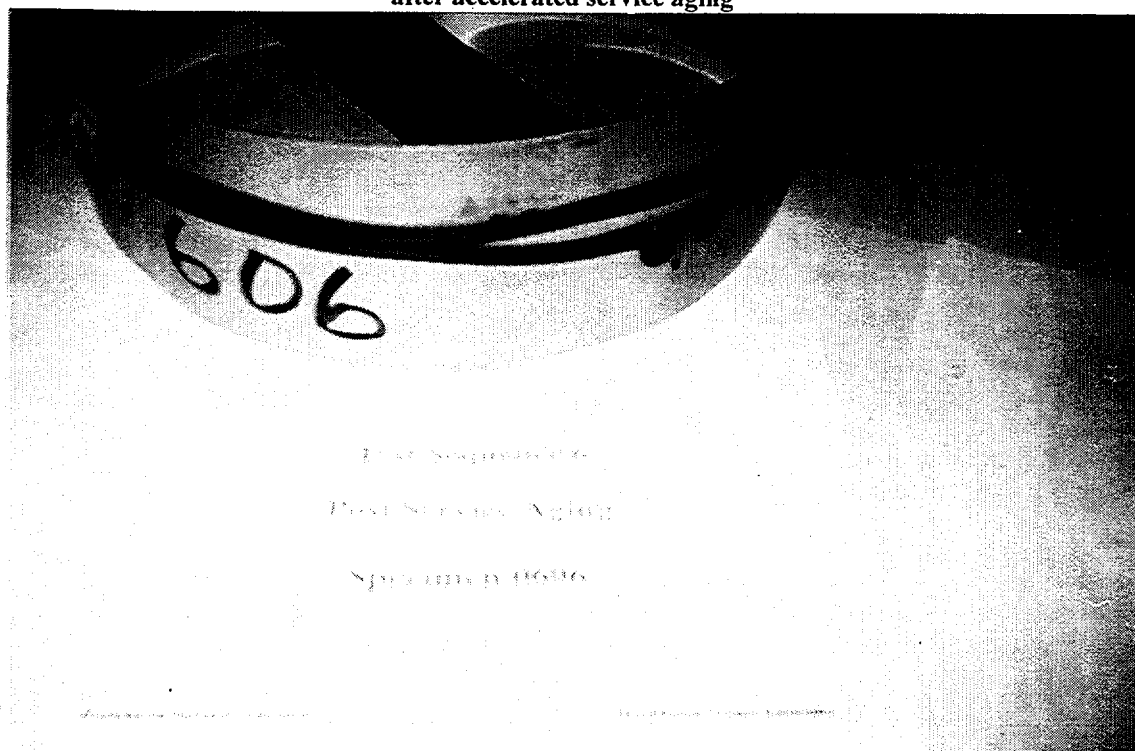
Figure 3.36 Okonite specimen 0606 from Group 6.2 (pre-aged to 60 years) after accelerated service aging
