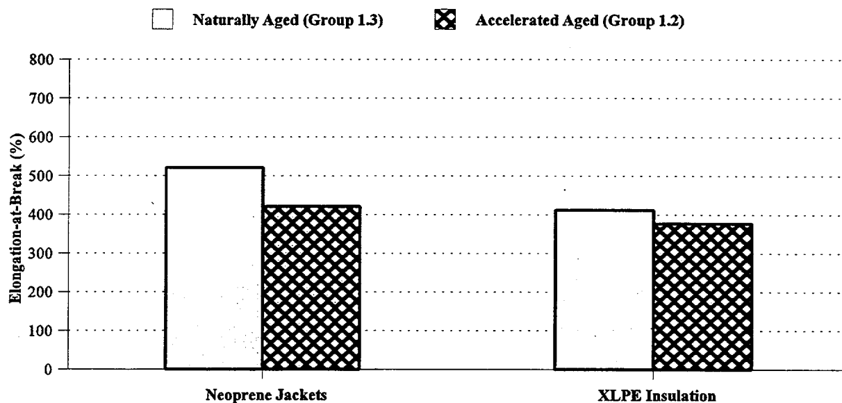
Figure 4.1 EAB values for naturally aged and accelerated aged Neoprene®/XLPE specimens from Test Sequence 1
