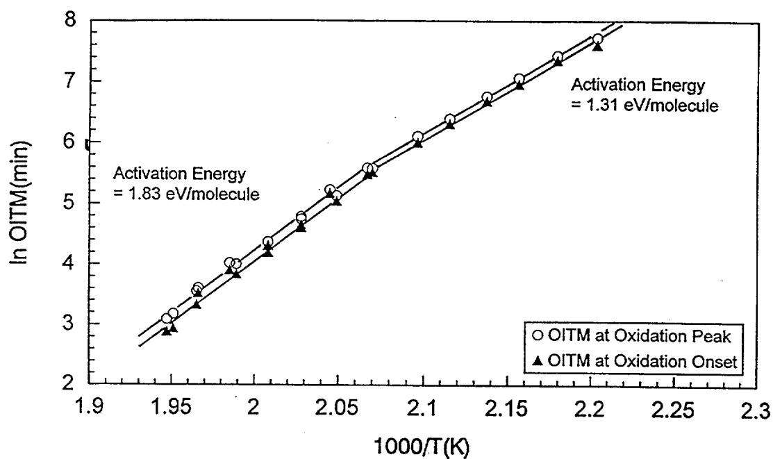
Figure 3.44 Arrhenius plot for white XLPE insulation
