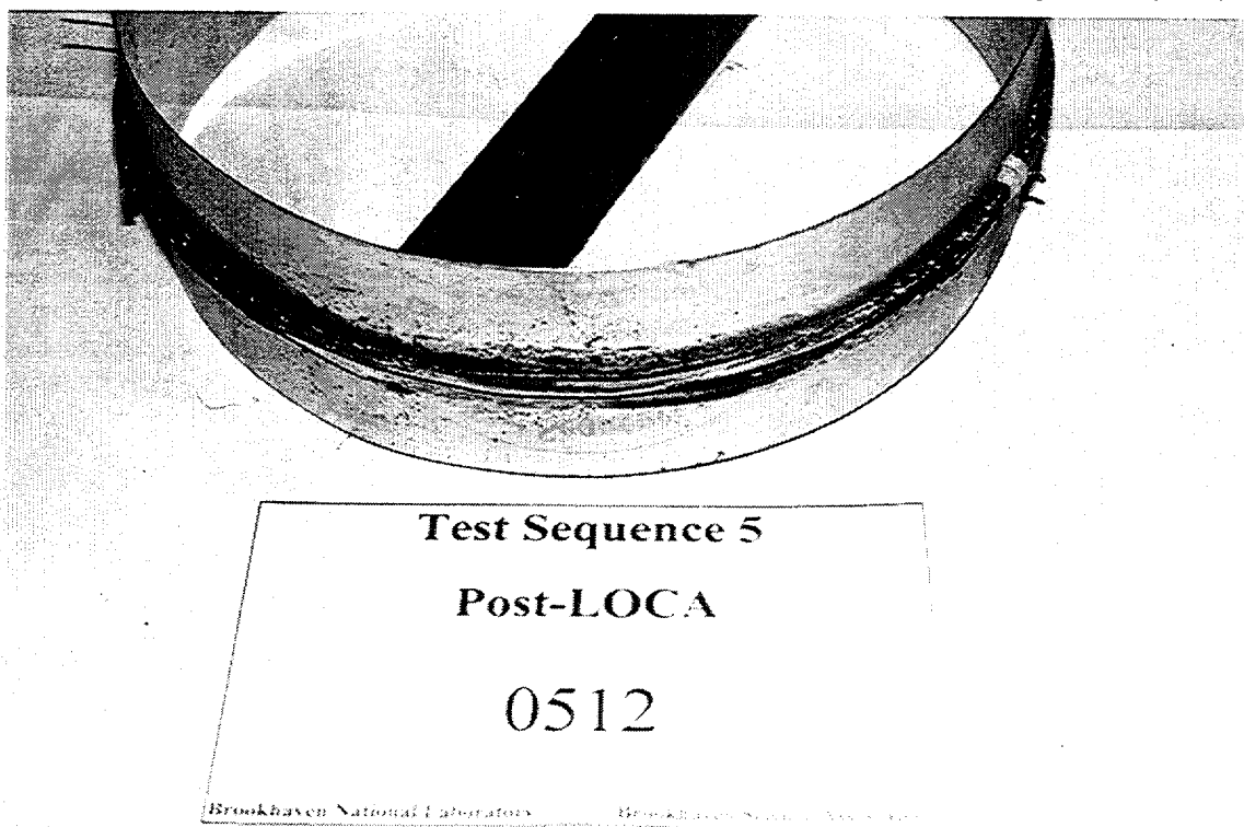
Figure 3.32 Post-LOCA condition of Okonite specimen 0512 in Group 5.3 (pre-aged to 40 years)
