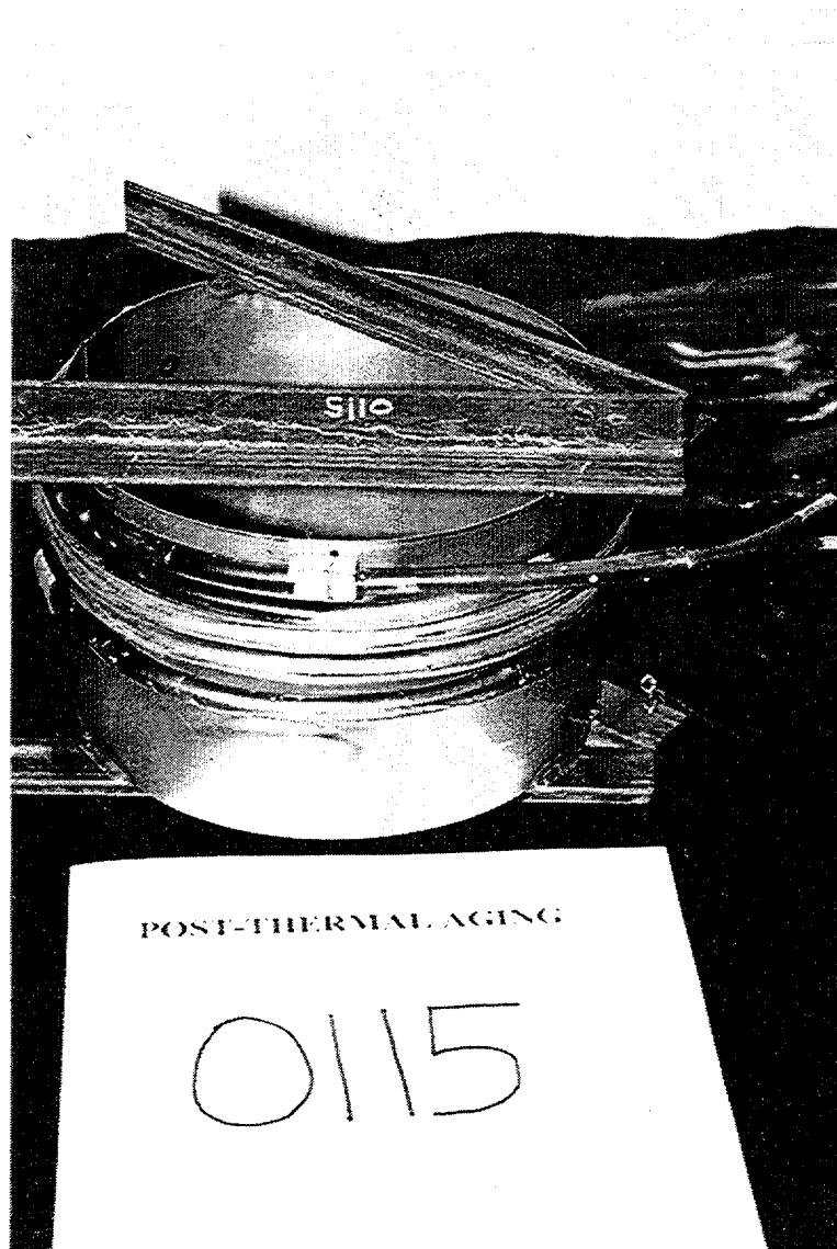
Figure 3.1 Rockbestos specimen 0115 from Group 1.4 (pre-aged to 20 years) after accelerated thermal aging
