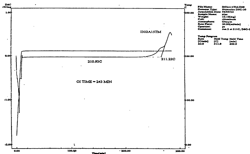
Figure 3.43 Typical DSC Thermogram for XLPE Insulation Oxidized in Oxygen at 410°F (210°C)
