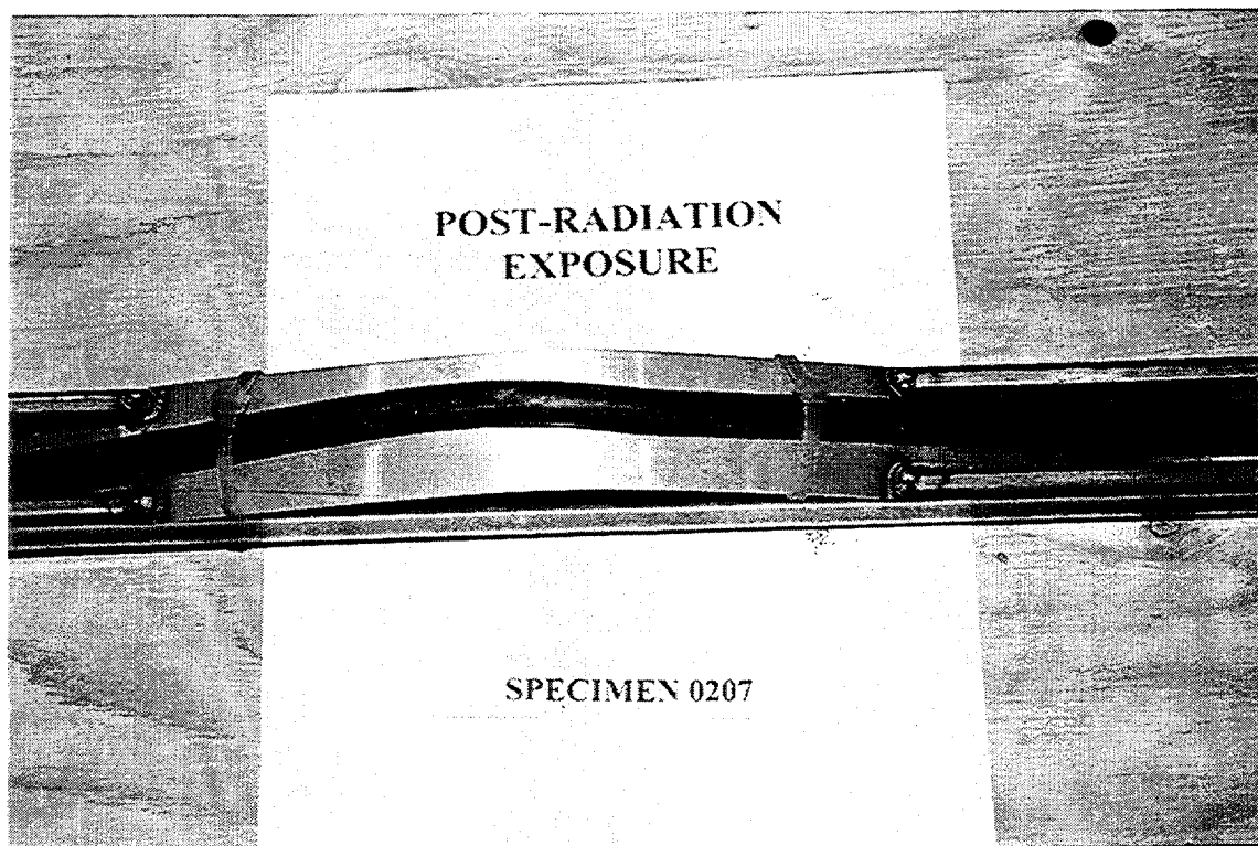
Figure 3.11 AIW specimen 0207 from Group 2.3 (naturally aged 24 years) after LOCA radiation
