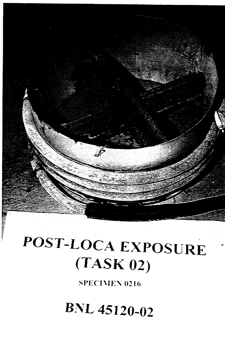
Figure 3.16 Post-LOCA condition of AIW specimen 0216 from Group 2.4 (pre-aged to 20 years)
