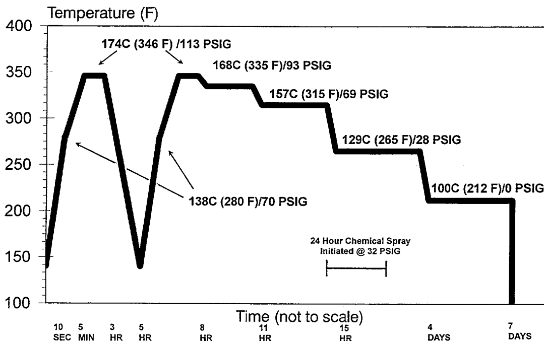
Figure 3.3 Test chamber temperature/pressure profile used in LOCA Tests 1, 3, 4, 5 and 6 (Note: LOCA Tests 4, 5 and 6 were 10 days in duration)
