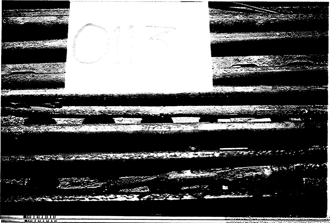
Figure 3.4 Post-LOCA condition of Rockbestos specimen 0113 from Group 1.4 (pre-aged to 20 years)
