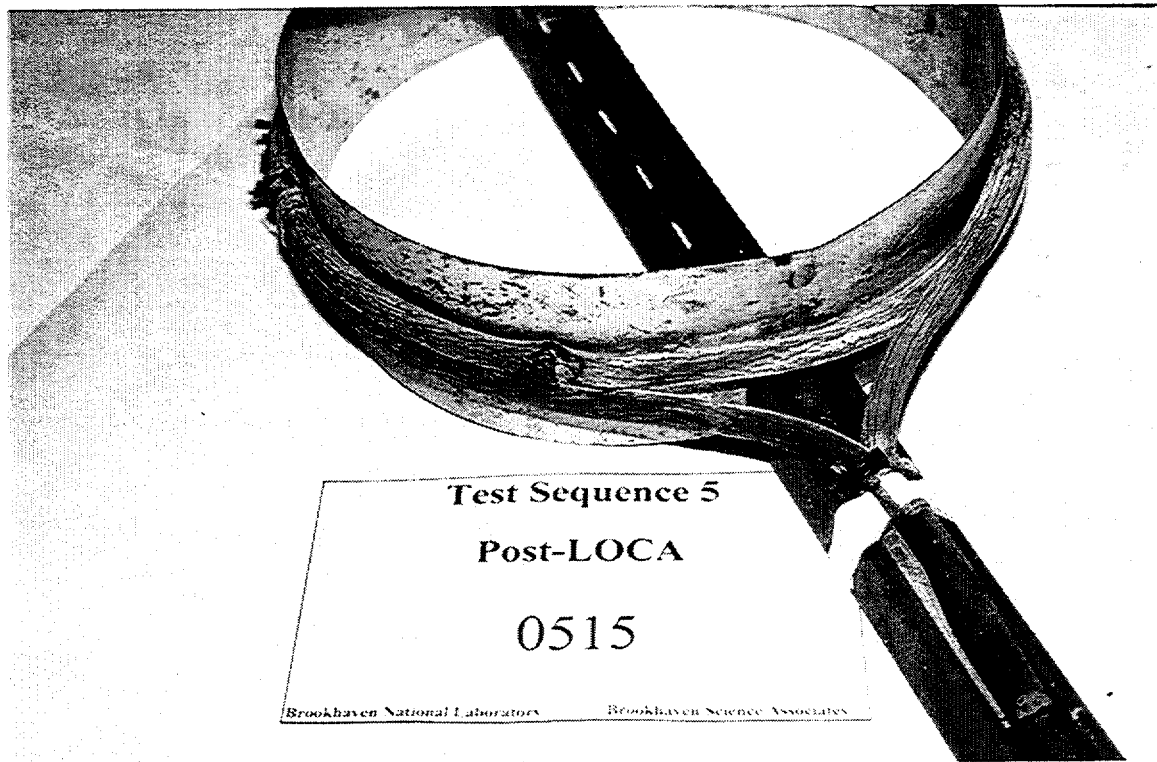
Figure 3.29 Post-LOCA condition of Anaconda specimen 0515 from Group 5.3 (pre-aged to 40 years)
