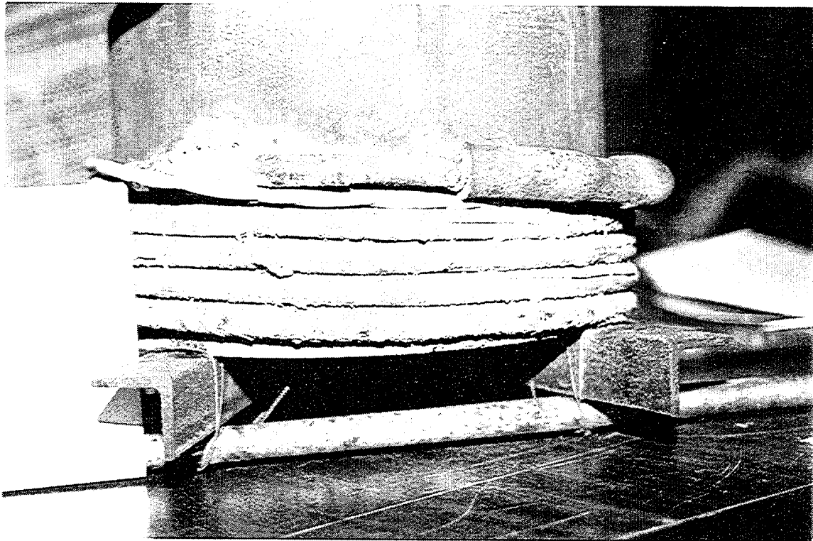
Figure 3.5 Post-LOCA condition of Rockbestos specimen 0115 from Group 1.4 (pre-aged to 20 years)
