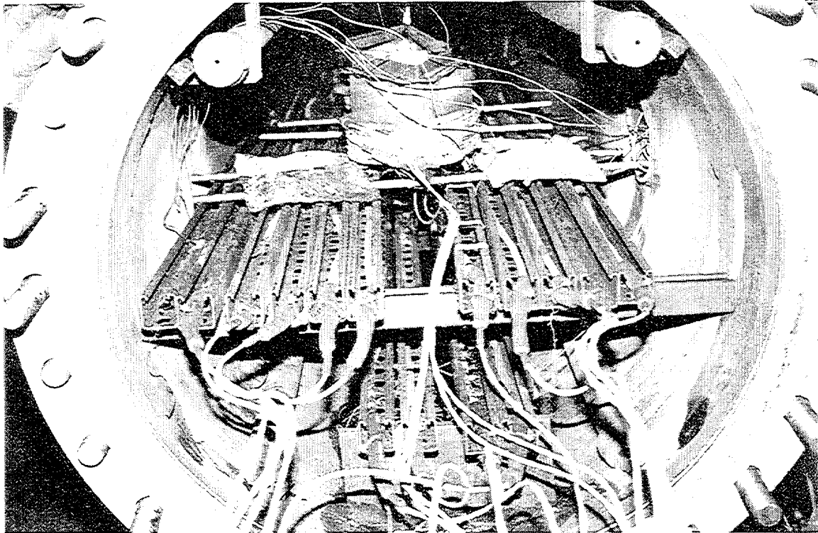
Figure 3.6 Rockbestos specimens in LOCA chamber after steam/chemical spray exposure
