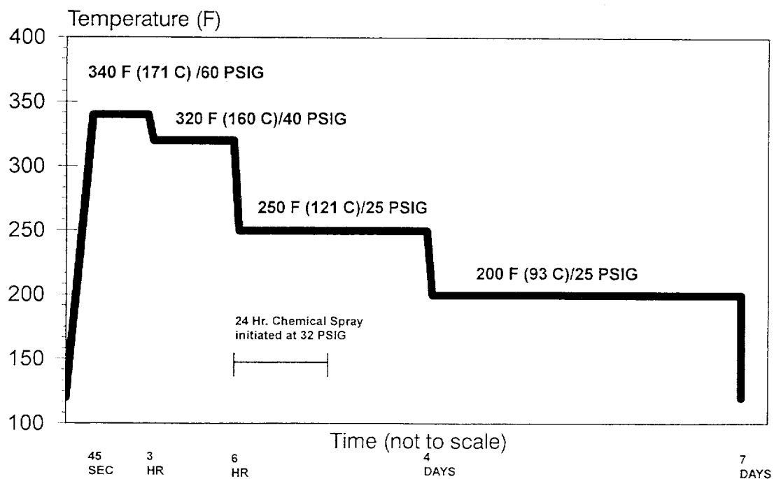
Figure 3.13 Test chamber temperature/pressure profile used in LOCA Test 2
