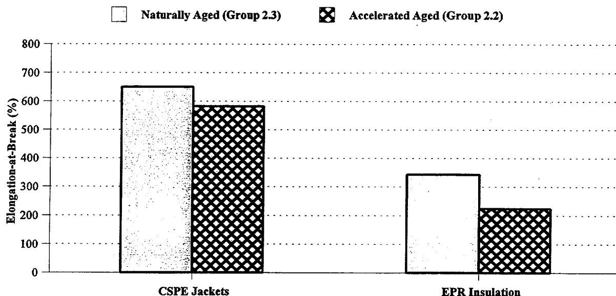
Figure 4.3 EAB values for naturally aged and accelerated aging CSPE/EPR specimens from Test Sequence 2
