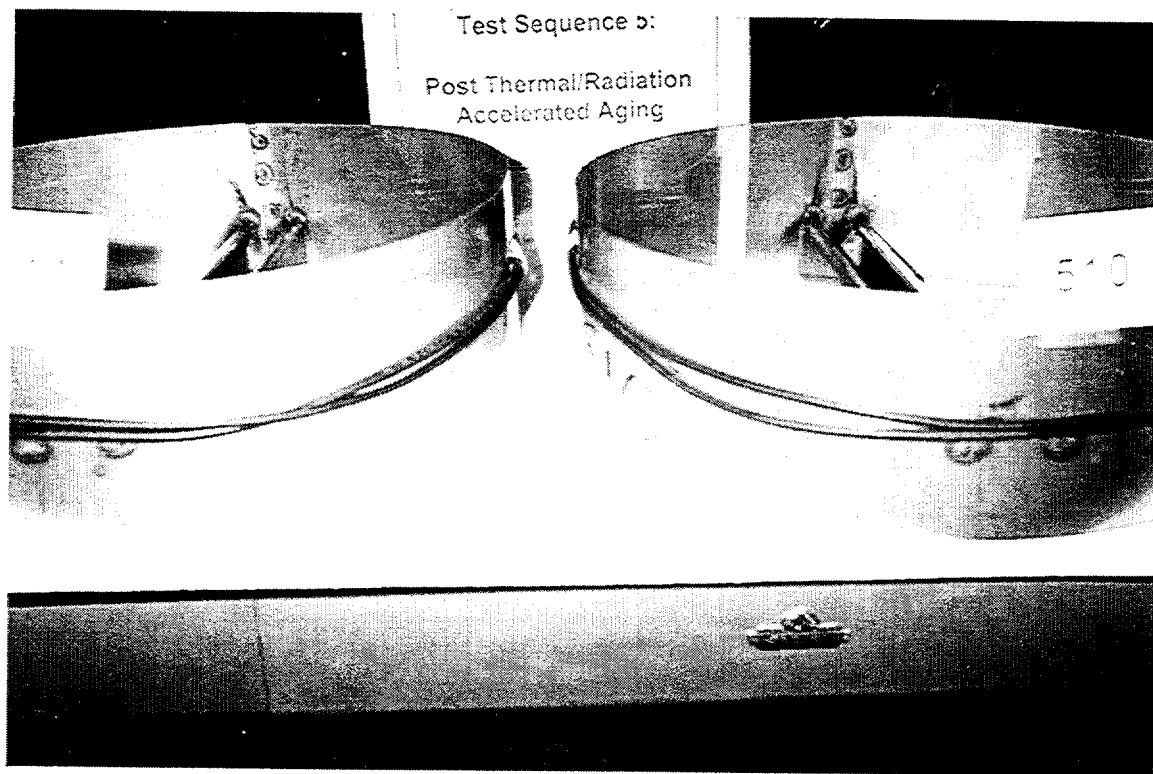
Figure 3.27 Okonite specimens 0510 and 0511 from Group 5.3 (pre-aged to 40 years) after accelerated service aging
