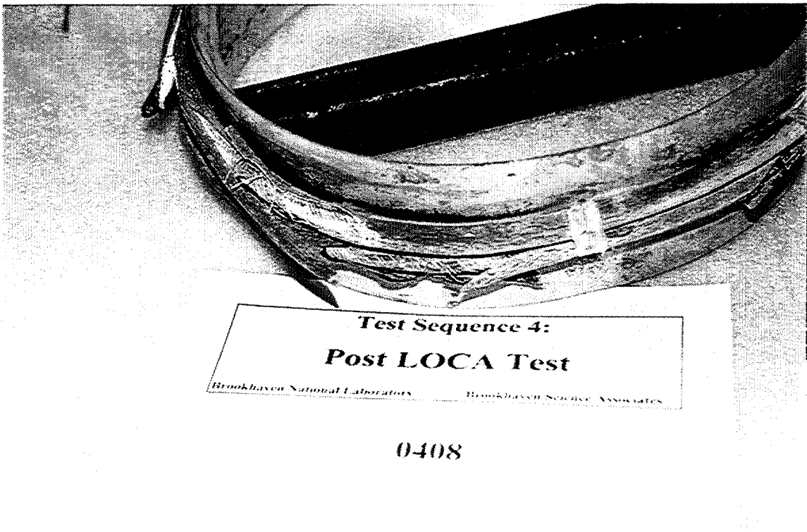
Figure 3.25 Post-LOCA condition of Anaconda multiconductor specimen 0408 from Group 4.3 (pre-aged to 40 years)
