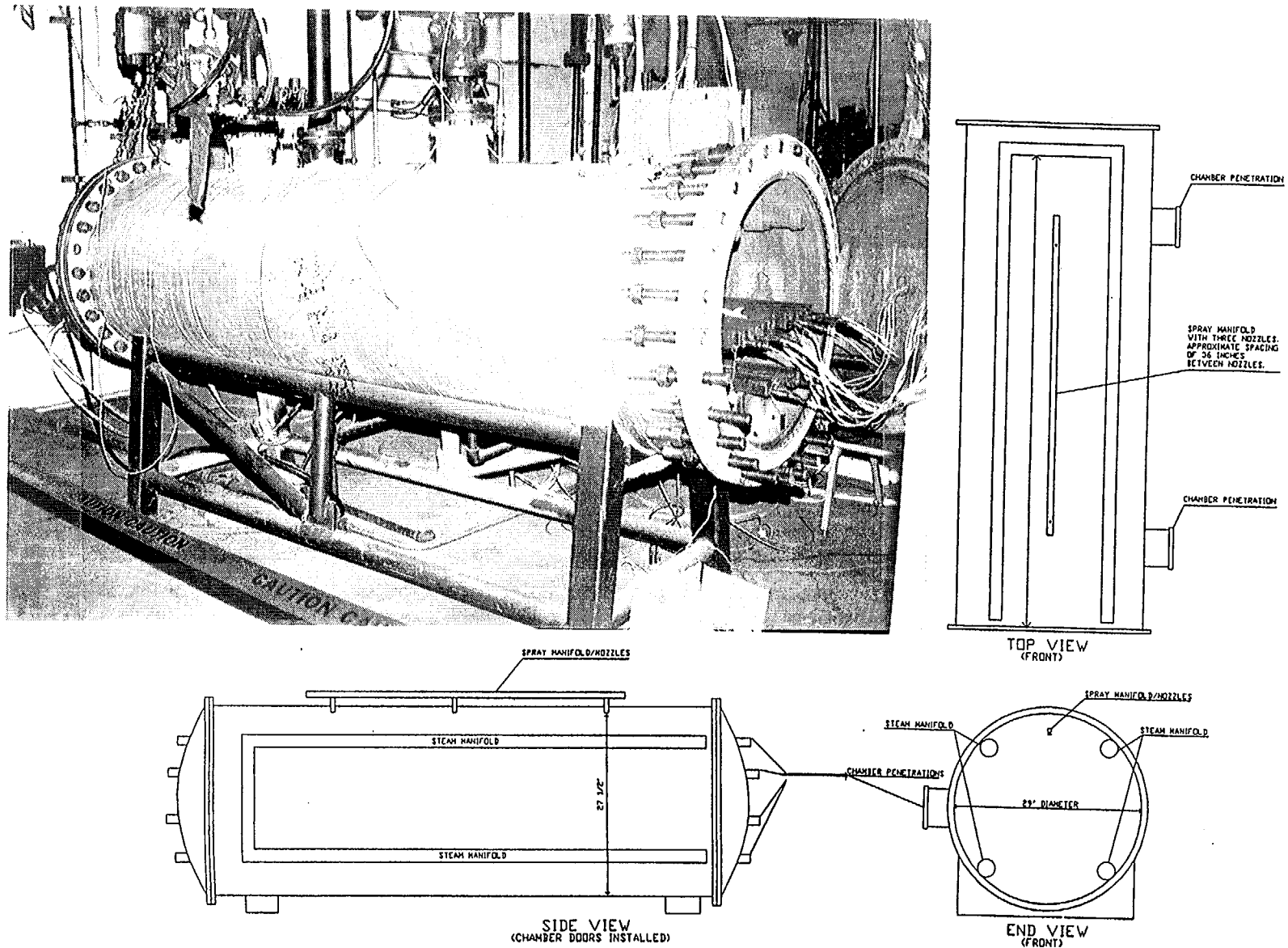
Figure 2.9 Photograph and diagram of the LOCA test chamber at Wyle Laboratories used for Tests 1, 2 and 3
