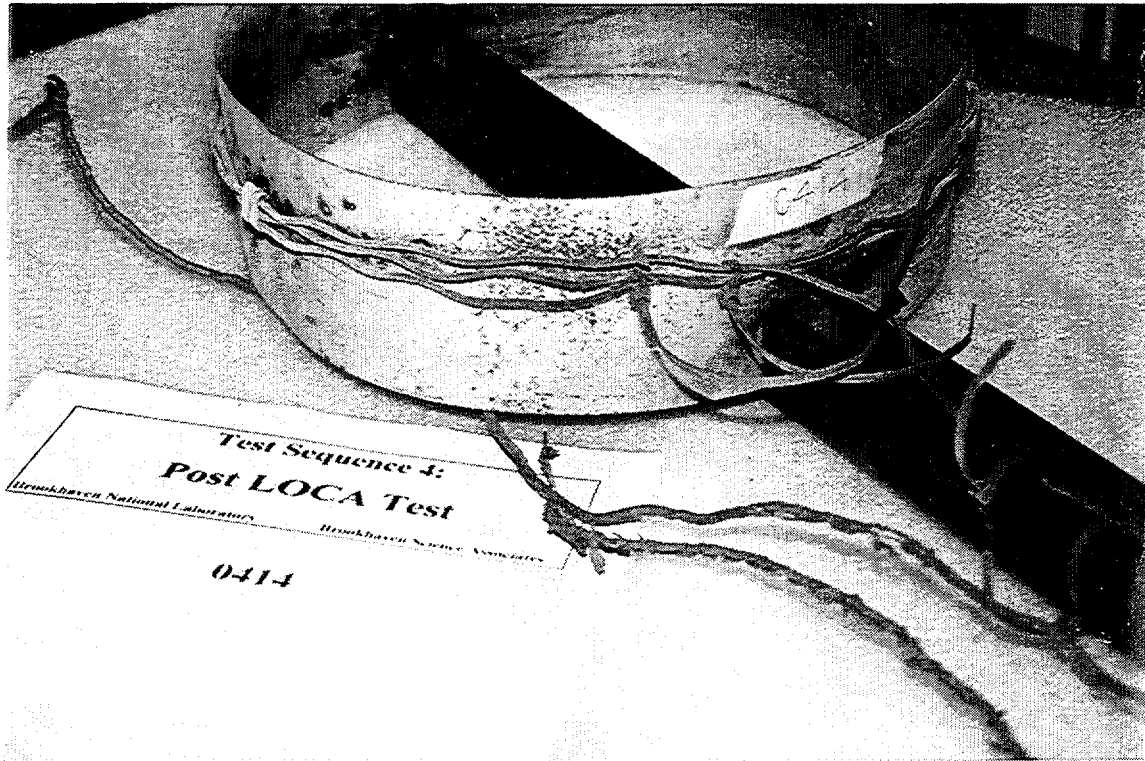
Figure 3.24 Post-LOCA condition of Samuel Moore single conductor specimen 0414 from Group 4.3
