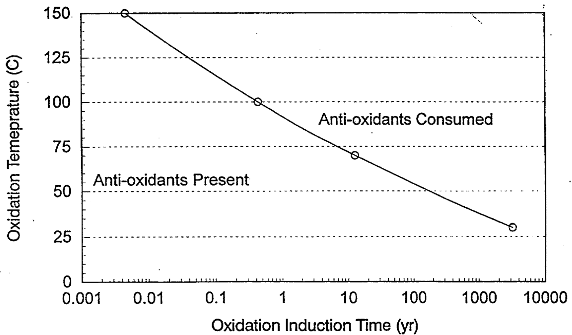
Figure 3.47 Estimated times for depletion of antioxidants in EPR as a function of aging temperature in an air environment
