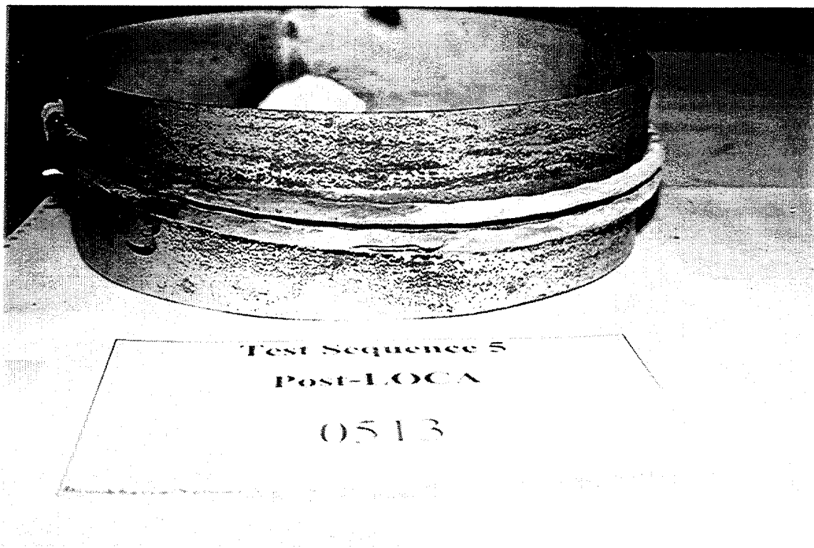
Figure 3.28 Post-LOCA condition of Samuel Moore specimen 0513 from Group 5.3 (pre-aged to 40 years)
