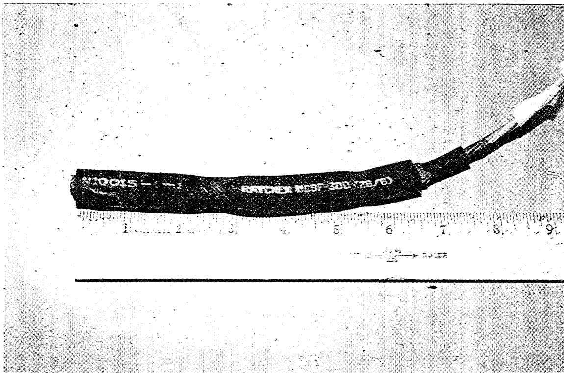
Figure 3.7 Raychem® splice as installed on specimen 0112
