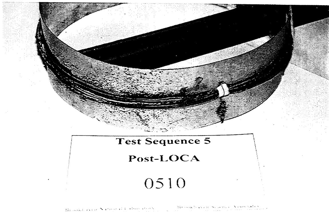
Figure 3.30 Post-LOCA condition of Okonite specimen 0510 in Group 5.3 (pre-aged to 40 years)
