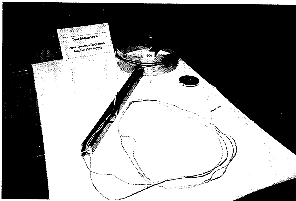
Figure 3.19 Anaconda single conductor specimen 0409 from Group 4.3 (pre-aged to 40 years) after accelerated service aging
