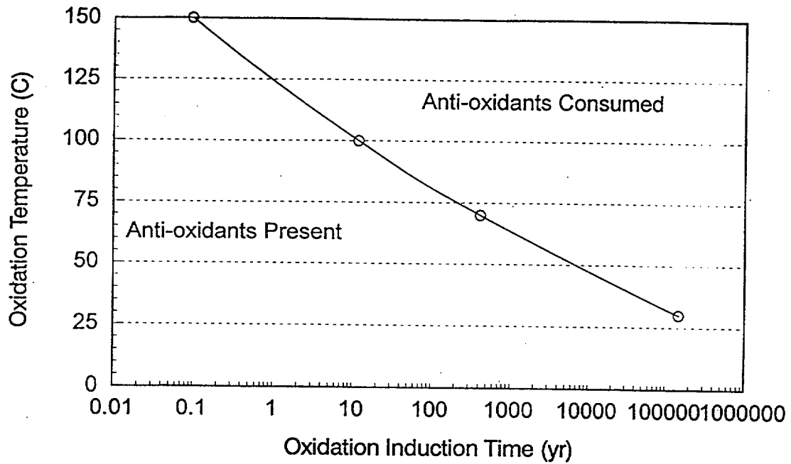
Figure 3.46 Estimated times for depletion of antioxidants in XLPE as a function of aging temperature in an air environment
