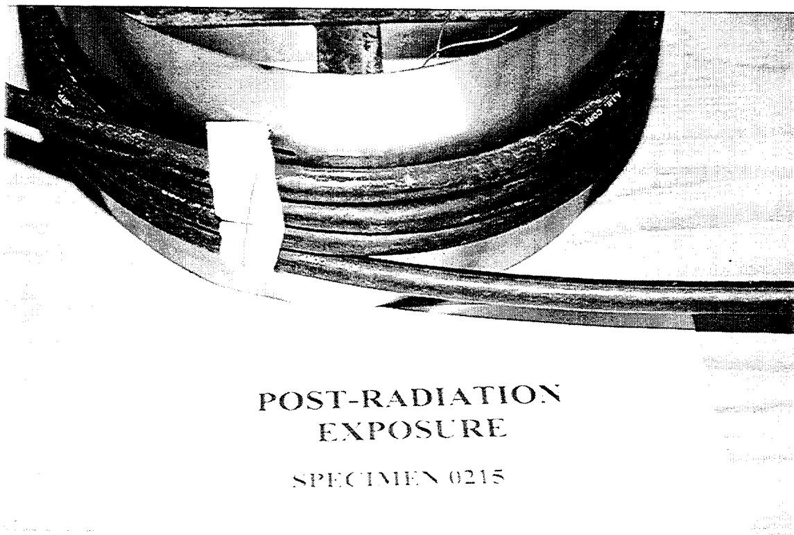
Figure 3.12 AIW specimen 0215 from Group 2.4 (pre-aged to 20 years) after service aging plus LOCA radiation
