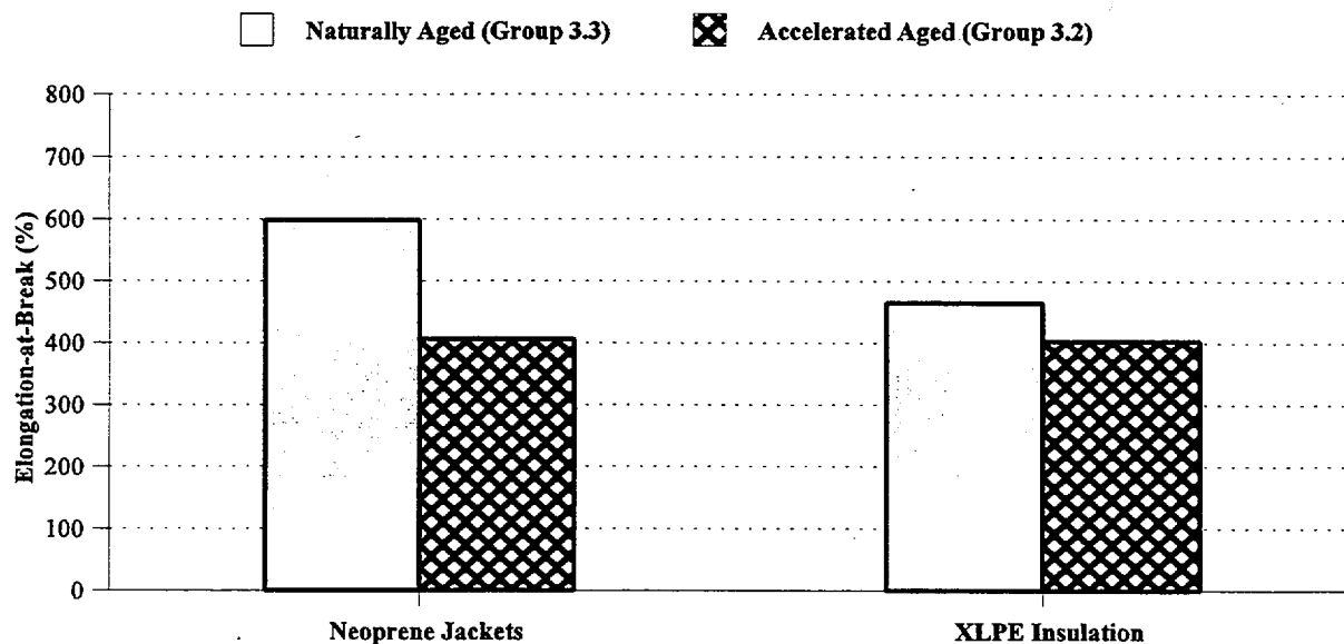
Figure 4.2 EAB values for naturally aged and accelerated aged Neoprene®/XLPE specimens from Test Sequence 3
