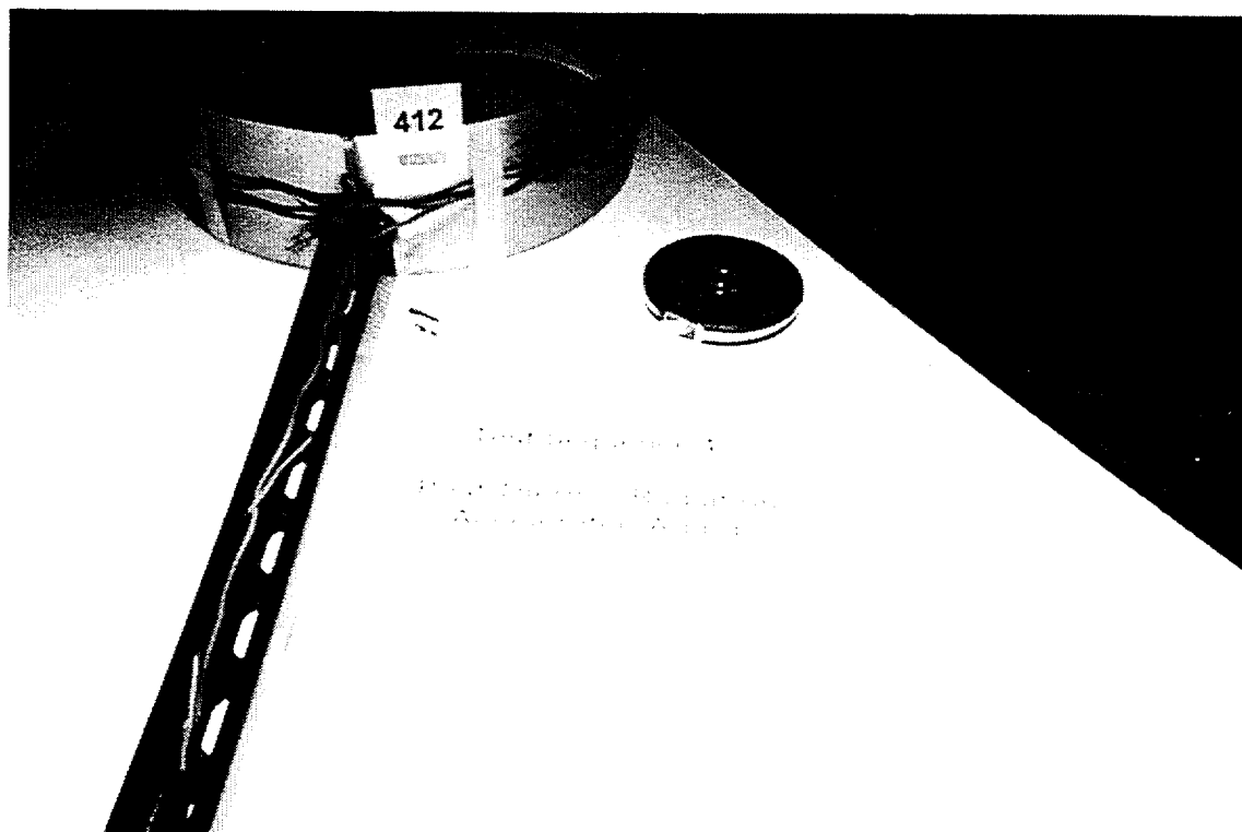
Figure 3.21 Samuel Moore single conductor specimen 0412 from Group 4.3 (pre-aged to 40 years) after accelerated service aging
