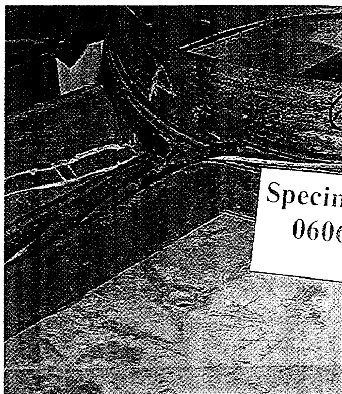
Figure 3.38 Post-LOCA condition of Okonite specimen 0606 from Group 6.2 (pre-aged to 60 years)
