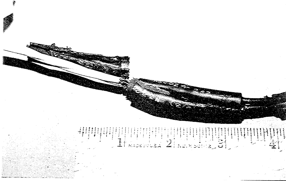
Figure 3.9 Raychem® splice with test lead shim removed
