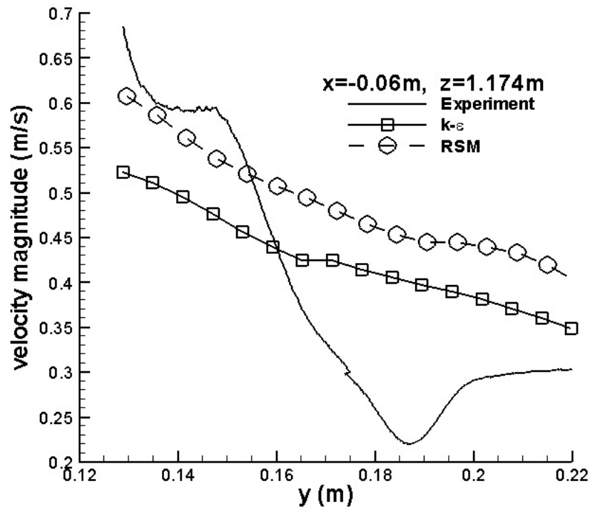
Fig. 35. Comparison between experimental and predicted velocity magnitude at x = -0.06\text{m}, z = 1.174\text{m} .
