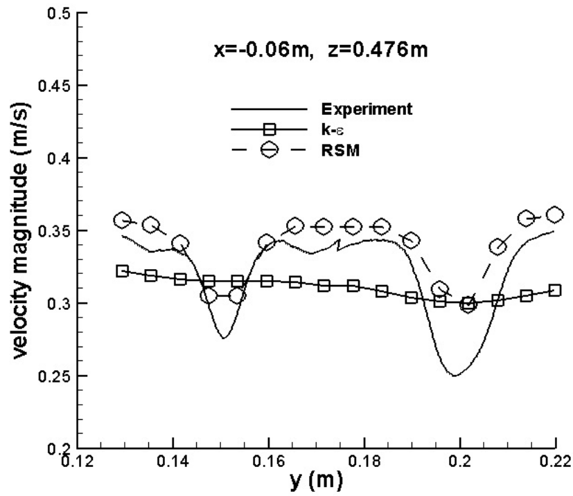
Fig. 33. Comparison between experimental and predicted velocity magnitude at x = -0.06\text{m}, z = 0.476\text{m} .
