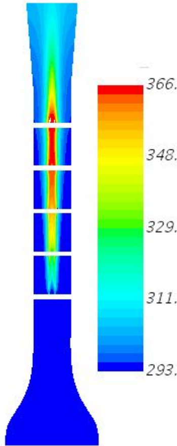
Fig. 42. Temperature contours for the RSM model on a y - z plane at x = 0 .
