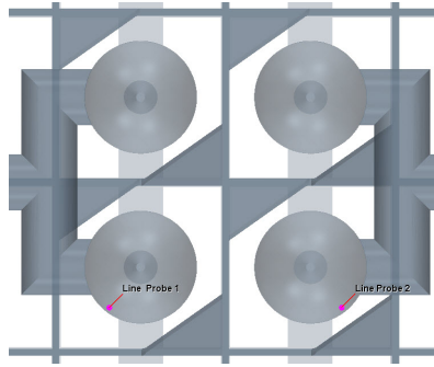
Fig. 25. Top view ( x - y plane) showing line plot locations on rod 1 and rod 2, denoted as Line Probe 1 and Line Probe 2, respectively, and swirler vane locations.
