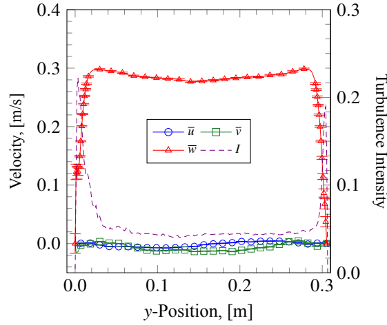
Fig. 20. Inlet velocity profile at the test section centerline ( x = 0 m) for the Natural700 case. The location of the profile is shown as a dashed line in Fig. 19. The velocity used for calculating turbulence intensity was \bar{w}_{\text{bulk}} = 0.2584 m/s.
