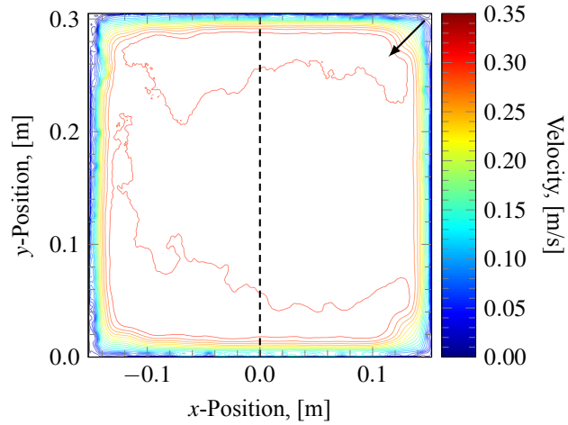
Fig. 19. Contour plot of the test section inflow measurement for the Natural700 case. The first contour level begins at 0 m/s and the increment is 0.0175 m/s. The arrow indicates increasing contour levels and the dashed line represents the location of the line profile in Fig. 20.
