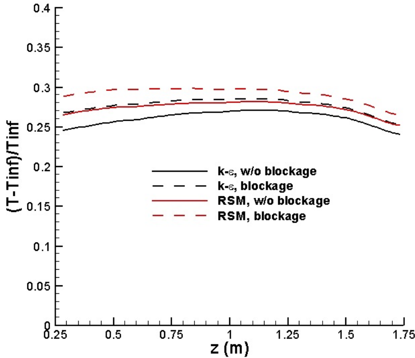
Fig. 26. Influence of inlet pressure losses on computed temperatures for rod 1.
