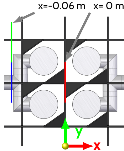
Fig. 9. Locations in the xy -directions of the PIV field of views for SRQ data acquisition. The coordinate system is shown for directional reference only and does not correspond to the actual location of the origin. The blue and green windows are centered at y = 0.152 m and y = 0.197 m, respectively. The red field of view is centered at y = 0.152 m on the x = 0 plane.
