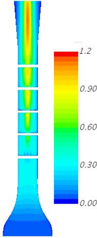
Fig. 39. Contours of velocity magnitude for the model on a y - z plane at x = 0 .
