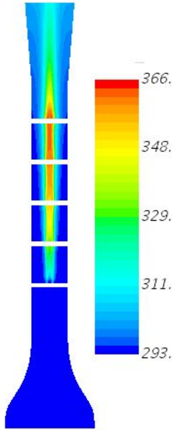
Fig. 41. Temperature contours for the model on a y - z plane at x = 0 .
