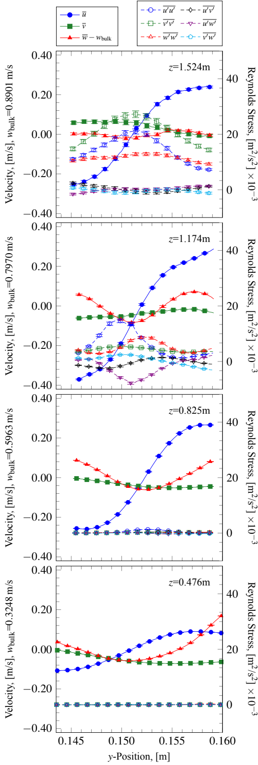
Fig. 21. Velocity profile along y -direction for x = 0 m at four z -positions indicated on each plot for the Natural700 case.
