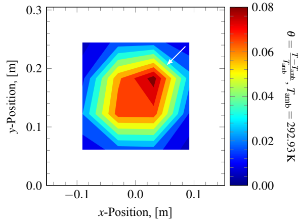
Fig. 16. Outlet fluid temperatures at z = 2 m for the Natural700 case. The contour scale begins at \theta = 0 and has an increment of 0.008. The arrow indicates the direction of increasing temperature. The TCs were arranged in a 4 \times 4 square grid and were evenly spaced across the test section outlet (61 mm apart in the x and y directions). TC uncertainty in terms of \theta was approximately \pm 0.0047 .
