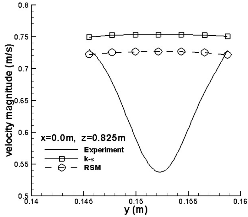
Fig. 30. Comparison between experimental and predicted velocity magnitude at x = 0.0\text{m} , z = 0.825\text{m} .
