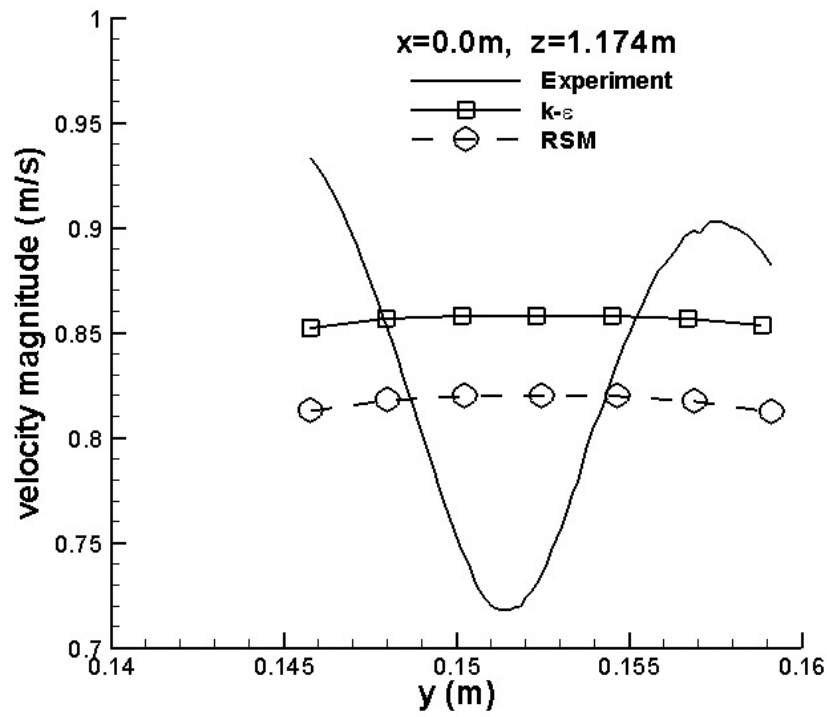
Fig. 31. Comparison between experimental and predicted velocity magnitude at x = 0.0\text{m} , z = 1.147\text{m} .
