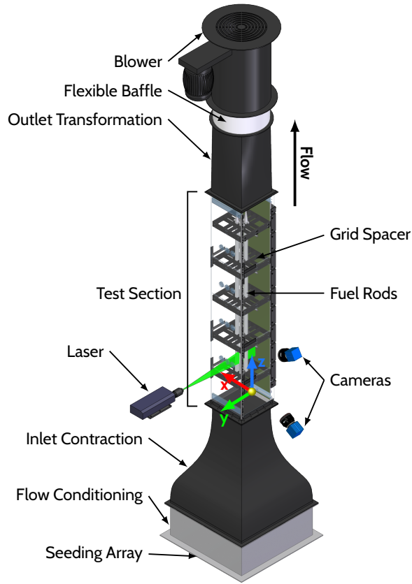
Fig. 3. A schematic of the wind tunnel showing the major components used in this study.
