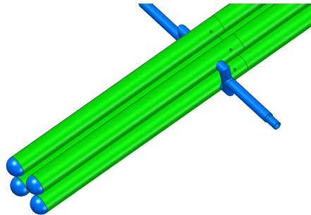
Fig. 4. Surface treatment of the leading edge of the fuel rod assembly. Blue surfaces represent polished aluminum and green surfaces represent nickel plating.
