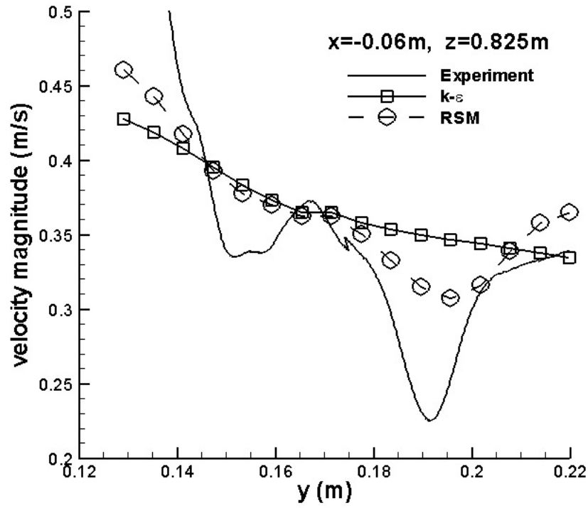
Fig. 34. Comparison between experimental and predicted velocity magnitude at x = -0.06\text{m}, z = 0.825\text{m} .
