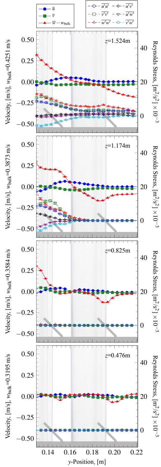
Fig. 22. Velocity profile along y -direction for x = -0.06 m at four z -positions indicated on each plot for the Natural700 case. The relative locations of the swirl elements in the y -position (not to scale in z ) are shown in the background of each figure.
