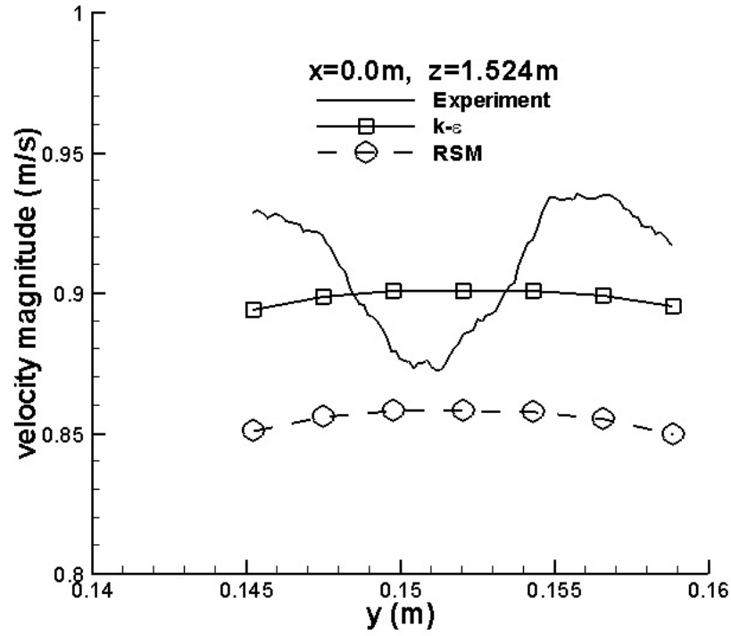
Fig. 32. Comparison between experimental and predicted velocity magnitude at x = 0.0\text{m}, z = 1.524\text{m} .
