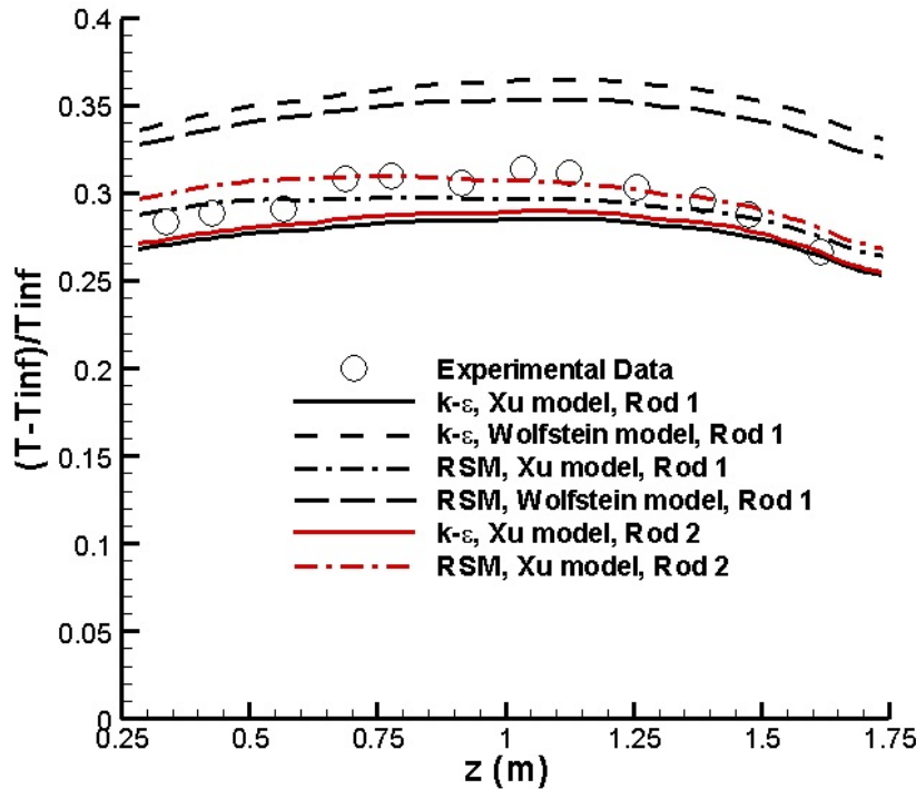
Fig. 27. Comparison between predicted and experimental rod temperatures.
