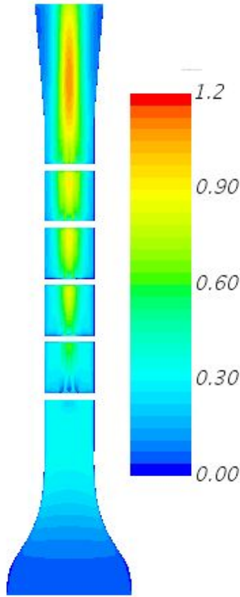
Fig. 40. Contours of velocity magnitude for the RSM model on a y - z plane at x = 0 .
