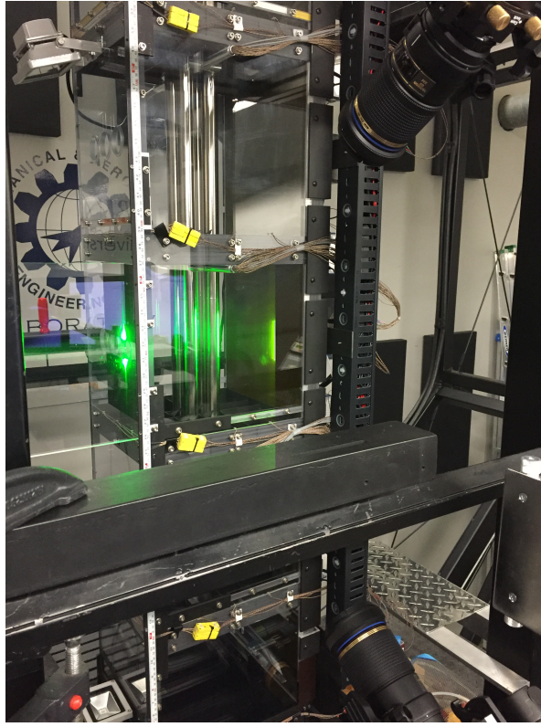
Fig. 8. A photograph of the PIV setup used to acquire SRQ velocity measurements. The camera lenses are shown in the upper right and lower right corners with the cameras out of frame. The laser is fired in a vertical sheet from the left of the image.
