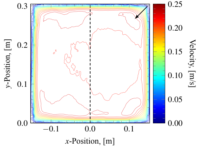
Fig. 17. Contour plot of the test section inflow measurement for the Natural400 case. The first contour level begins at 0 m/s and the increment is 0.0125 m/s. The arrow indicates increasing contour levels and the dashed line represents the location of the line profile in Fig. 18.
