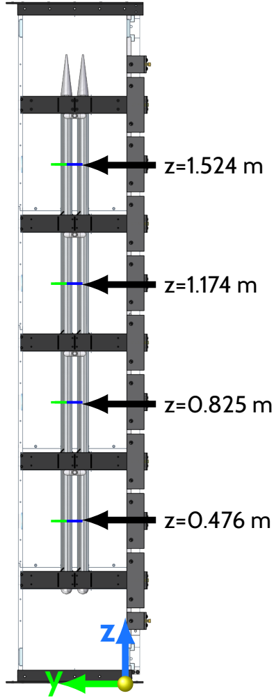
Fig. 10. Locations in the yz -plane of the PIV viewing windows for SRQ data acquisition. The blue and green windows are centered at y = 0.152 m and y = 0.197 m, respectively, on the x = -0.06 m plane. The fields of view on the x = 0 m plane are aligned in the y and z directions with the blue fields of view.
