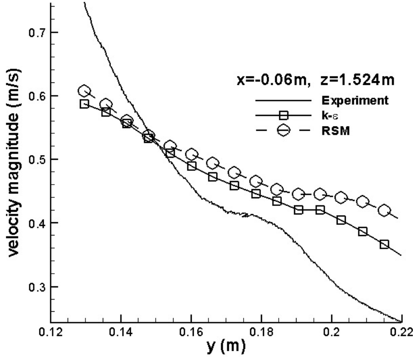
Fig. 36. Comparison between experimental and predicted velocity magnitude at x = -0.06\text{m} , z = 1.524\text{m} .
