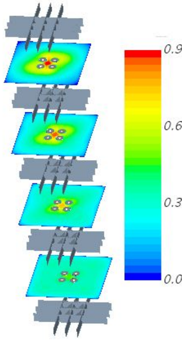
Fig. 37. Contours of velocity magnitude at constant z -planes 0.476m, 0.825m, 1.174m, and 1.524m, corresponding to z locations in Figs. 30 to 37. Spacers shown for reference purposes.
