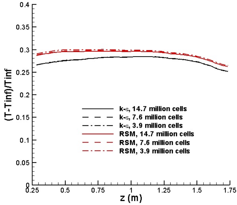
Fig. 28. Grid resolution study results for rod 1.
