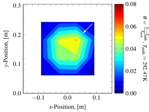
Fig. 15. Outlet fluid temperatures at z = 2 m for the Natural400 case. The contour scale begins at \theta = 0 and has an increment of 0.008. The arrow indicates the direction of increasing temperature. The TCs were arranged in a 4 \times 4 square grid and were evenly spaced across the test section outlet (61 mm apart in the x and y directions). TC uncertainty in terms of \theta was approximately \pm 0.0046 .
