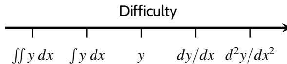
Fig. 2. Spectrum of difficulty to measure or acquire an arbitrary SRQ, y(x) , after [5].
