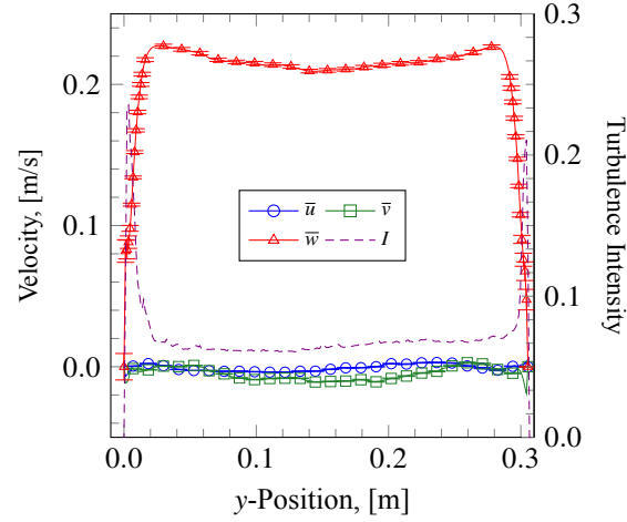
Fig. 18. Inlet velocity profile at the test section centerline ( x = 0 m) for the Natural400 case. The location of the profile is shown as a dashed line in Fig. 17. The velocity used for calculating turbulence intensity was \bar{w}_{\text{bulk}} = 0.1956 m/s.
