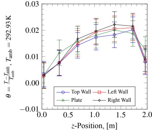
Fig. 14. Wall temperatures in the stream-wise direction for the Natural700 case.
