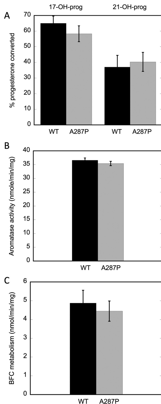
FIGURE 2. CYP17A1, CYP21A2, CYP19A1 (aromatase), and CYP3A11 activities supported by WT and A287P POR proteins. A, percentage of progesterone converted to 17-OH-progesterone by CYP17A1 and 21-OH progesterone by CYP21A2. B, aromatase activity as measured by conversion of androstenedione to estrone. C, conversion of BFC to HFC by xenobiotic-metabolizing CYPs. Black bars are WT POR and gray bars are A287P. Assays were repeated at least three times and were performed as described under "Experimental Procedures."
