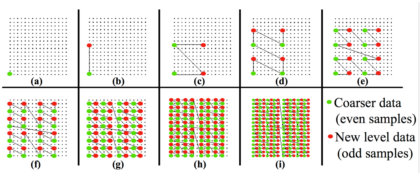
Figure 33 (a-i). The nine levels of resolution of the binary tree hierarchy defined by the 2D space filling curve applied on 16 \times 16 rectilinear grid. The coarsest level of resolution (a) is a single point. The number of points that belong to the curve at any level of resolution (b) to (i) is double the number of points of the previous level.
