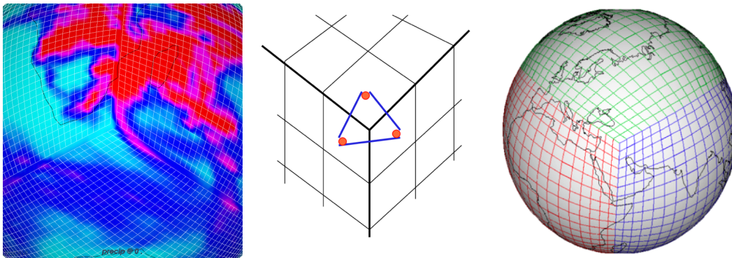
Figure 24. These images show cell-centered precipitation on the cubed-sphere and how the connectivity between cubed-sphere tiles is used in order to fill in the color of the inter-tile gaps and of the triangular cell covering the three-tile corner. This was done explicitly by showing the fields on each tile, and creating 12 gap and 8 corner cell grids.
