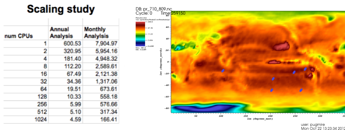
Figure 30. Scaling study and R execution. Left: Scalability of Extreme Value Analysis code. Right: Peaks Over Threshold of 100-year, daily precipitation CCSM3.0 data.
