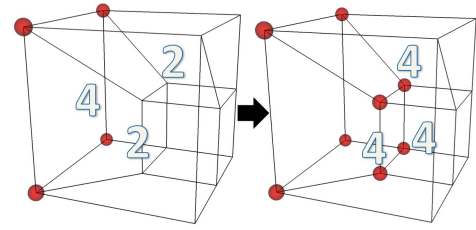
Fig. 23. Example of 3D node marking propagation on an element previously refined using a 1-template.
