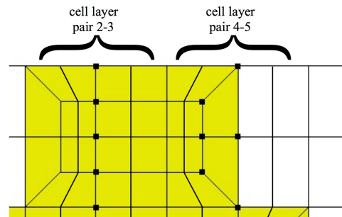
Fig. 21. Example of resulting mesh where node propagation has been performed.
