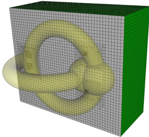
Fig. 34. Cut-away of refined base mesh for a027 model
