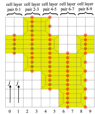
Fig. 11. Nodes marked in J direction at every other column adjacent marked elements.
