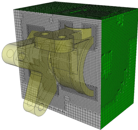
Fig. 36. Cut-away of refined base mesh for driver model
