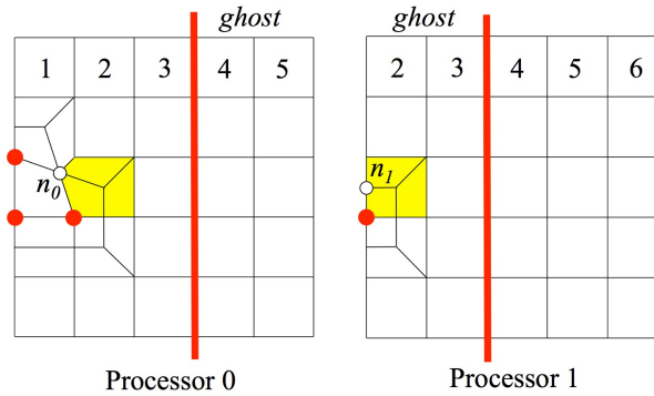
Fig. 31. Illustration of discrepancy between node location n_0 and n_1 on neighboring processors resulting from a 3-template near a processor boundary.
