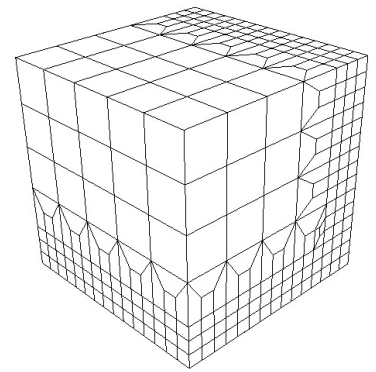
Fig. 3. Example 3D mesh using a 3-refinement procedure
