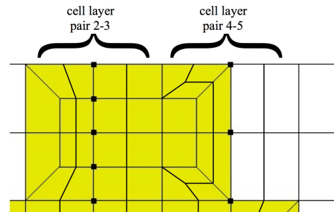
Fig. 19. Resulting mesh from basic marking procedure. Note poor angles produced from 1-templates adjacent the marked nodes a and c in fig. 18.
