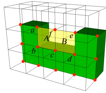
Fig. 25. Node f would also be marked to avoid two adjacent 3 -templates
