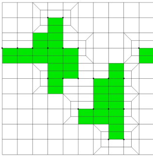
Fig. 9. Templates shown in figure 4 applied to marked nodes in I direction.
