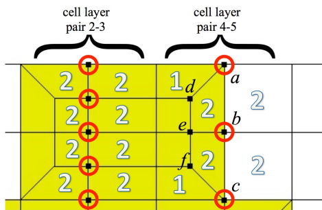
Fig. 18. Close-up of node marking and resulting templates based on procedure described above.
