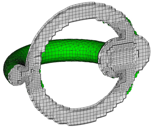
Fig. 35. Sculpt mesh of a027 model
