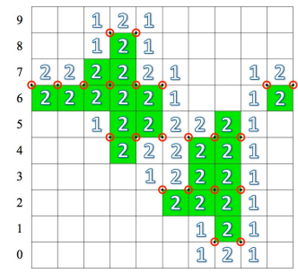
Fig. 8. Refinement templates identified based on marked nodes. In 2D only 1 and 2 templates are permitted.
