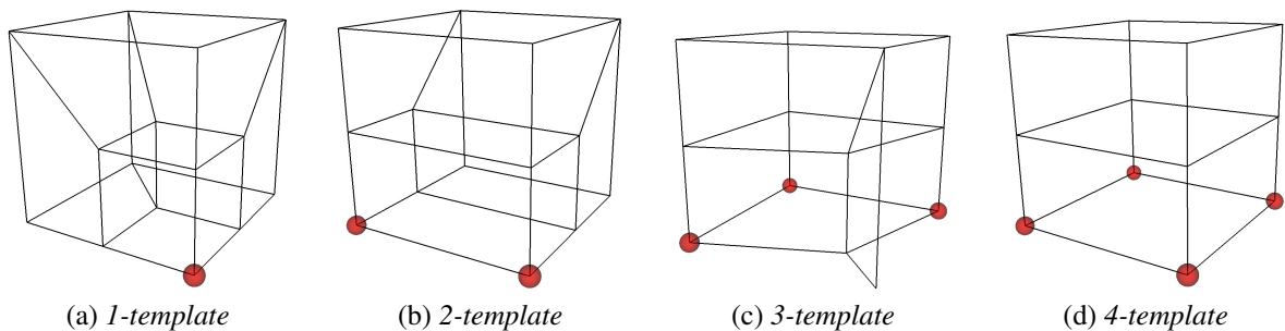
Fig. 5. Complete set of 3D 2-refinement templates. Templates are identified based on the number of marked nodes on a hex
