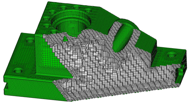
Fig. 33. Sculpt mesh of anc101 model
