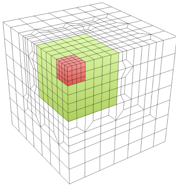
Fig. 26. Example 3D refinement showing first level of refinement from green cells. Green cells will serve as transition zone for second level of refinement from uniformly refined red cells
