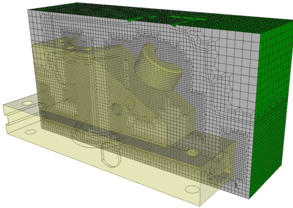
Fig. 32. Cut-away of refined base mesh for anc101 model
