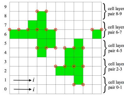
Fig. 7. Each odd-even row pair of quads are traversed and nodes between the rows adjacent to at least one marked quad is also marked.
