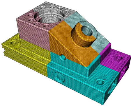
Fig. 38. anc101 model used in performance study. Illustrates final mesh generated with sculpt [4] on 8 processors. Color represents the different processor domains. Performance numbers in fig. 39 are for refinement algorithm only and do not include time to generate the final mesh.
