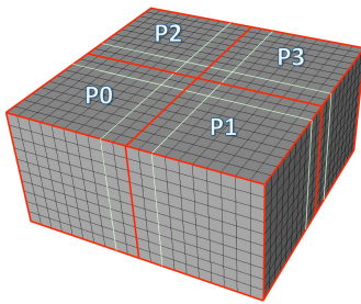
Fig. 29. Example parallel distribution of Cartesian grid on four processors
