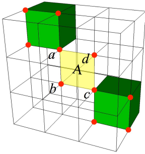
Fig. 24. Nodes b and d at face A would also be marked to avoid an invalid template for adjacent cells at A
