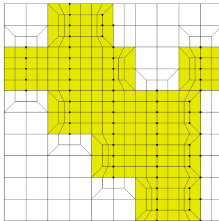
Fig. 12. Templates applied on marked nodes in J direction.
