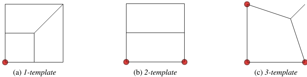
Fig. 4. Complete set of 2D 2-refinement templates. Templates are identified based on number of marked nodes on a quad or hex face. Note that for 2D, only the 1-template and 2-template are required. The 2D 3-template is used only in the context of 3-refinement for refining a hex face of the 3D 3-template (Fig. 5c).
