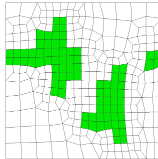
Fig. 13. 2D example from figure 12 following smoothing. Shaded quads illustrate the initial cells identified for uniform refinement.
