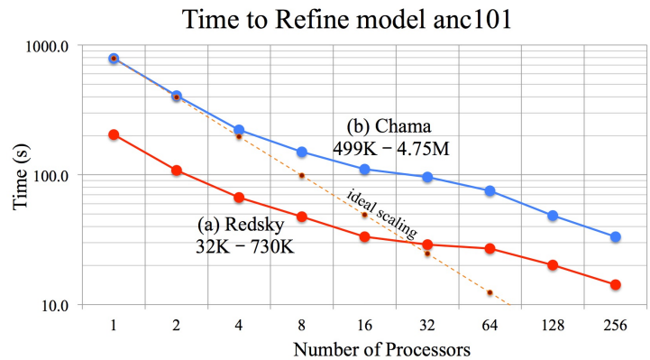
Fig. 39. Performance of refinement vs number of processors for model anc101. (a) Initial hexes in Cartesian grid: 32,400, Final number: 730,512. Tests performed on Sandia's Redsky platform (519/4,152 nodes/cores 2.93GHz Intel, 12GB/node) (b) Initial hexes in Cartesian grid: 498,960, Final number: 4,750,848. Tests performed on Sandia's TLCC2 Chama platform (1,232/19,712 nodes/cores 2.6GHz Intel, 64GB/node). Note all runs on respective machines produced identical meshes regardless of processor count.
