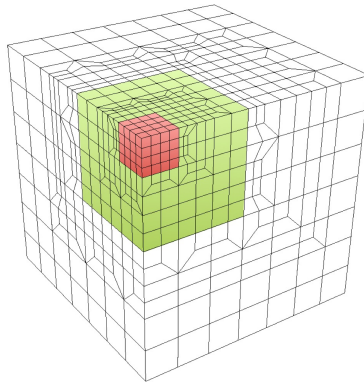
Fig. 27. Transition elements for second level of refinement added.
