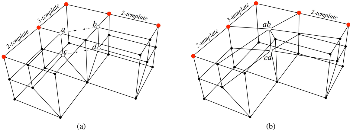
Fig. 17. (a) Two completed 2-templates adjacent a partially completed 3-template. Nodes a and b are merged as well as nodes c and d (b) View of completed 3-template with modified adjacent 2-templates after merging nodes.
