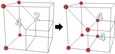
Fig. 22. Example of 3D node marking propagation on an element previously refined using a 2-template.
