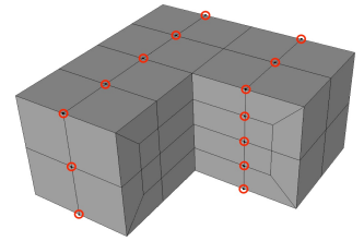
Fig. 16. Cut-away of example 3D mesh with nodes marked in J direction
