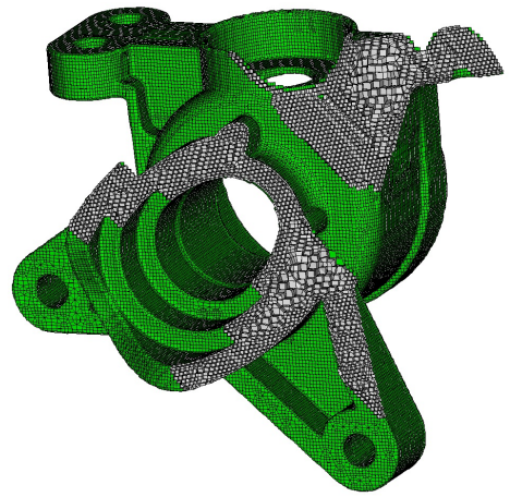
Fig. 37. Sculpt mesh of driver model
