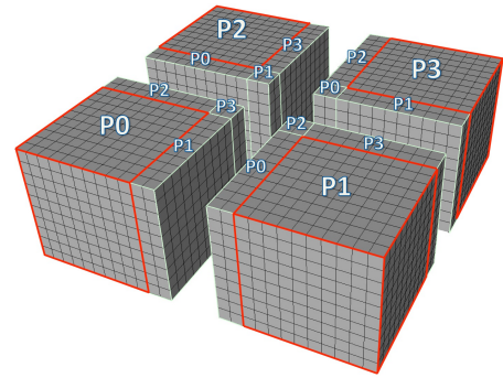
Fig. 30. Exploded view of 4 processors where ghosted cells of neighboring processors are included for each processor
