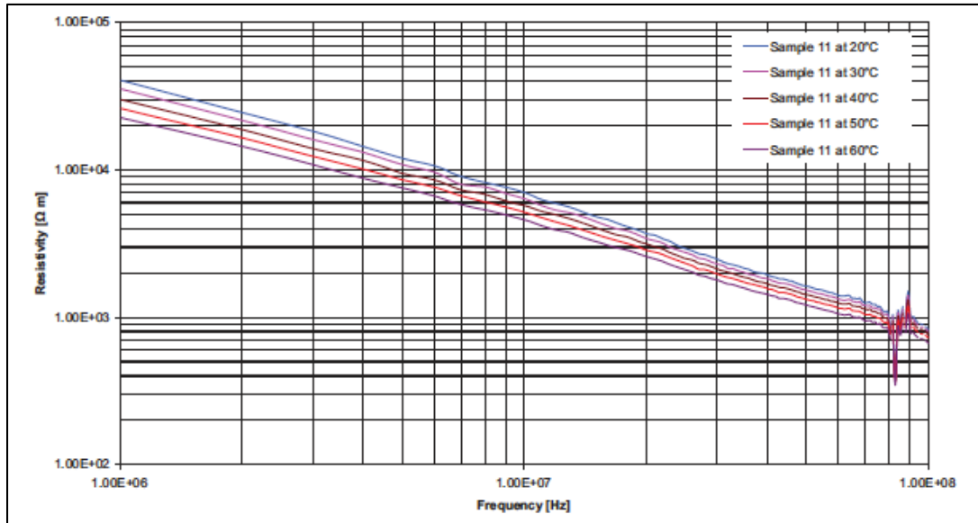
Figure 2: Temperature effect on resistivity – Sample 11 (Patil et al., 2010).
