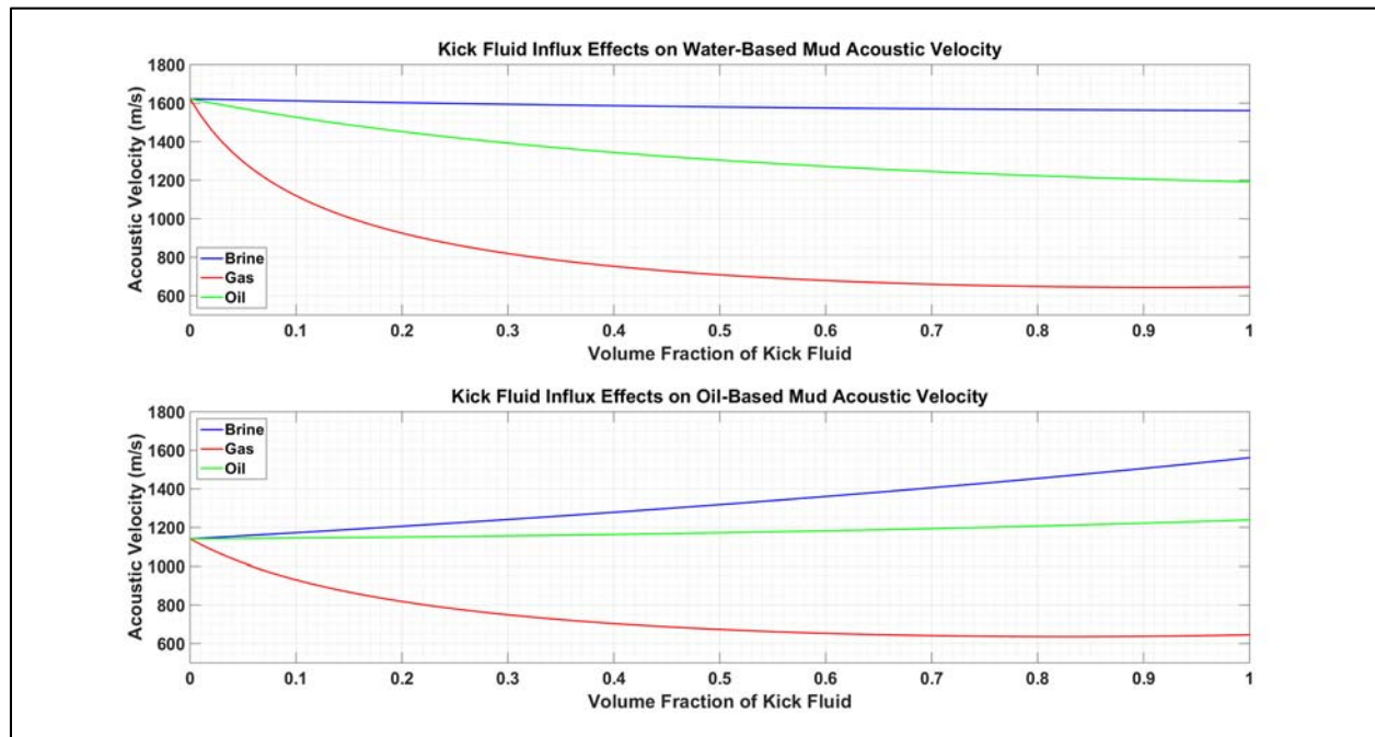
Figure 4: Effects of kick fluid mixing on drilling fluid acoustic/sonic velocity.
