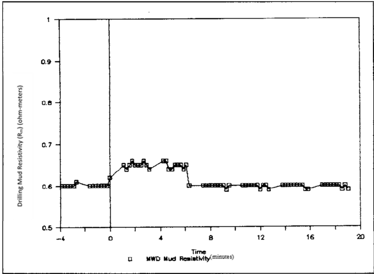
Figure 3: Gas influx detection using a downhole MWD mud resistivity sensor (Bryant et al., 1991).
