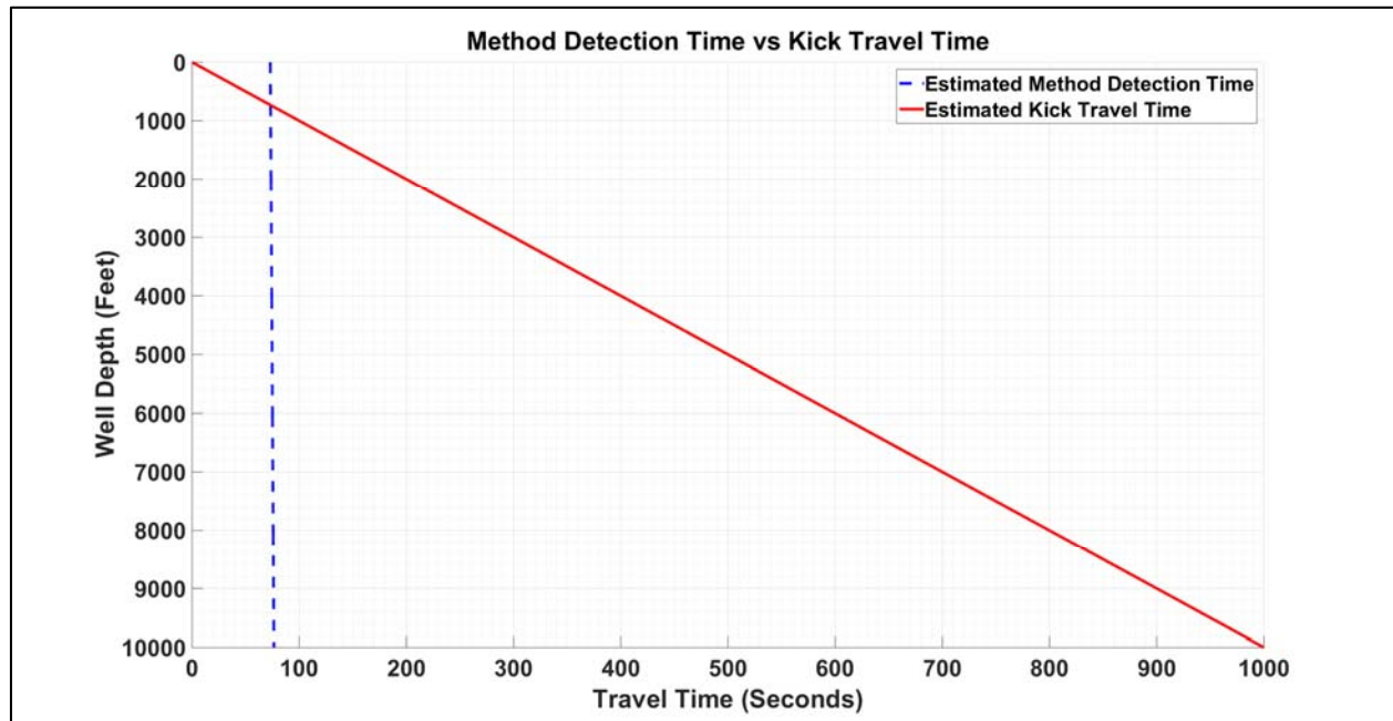
Figure 8: Modeling results for the gas kick scenario.
