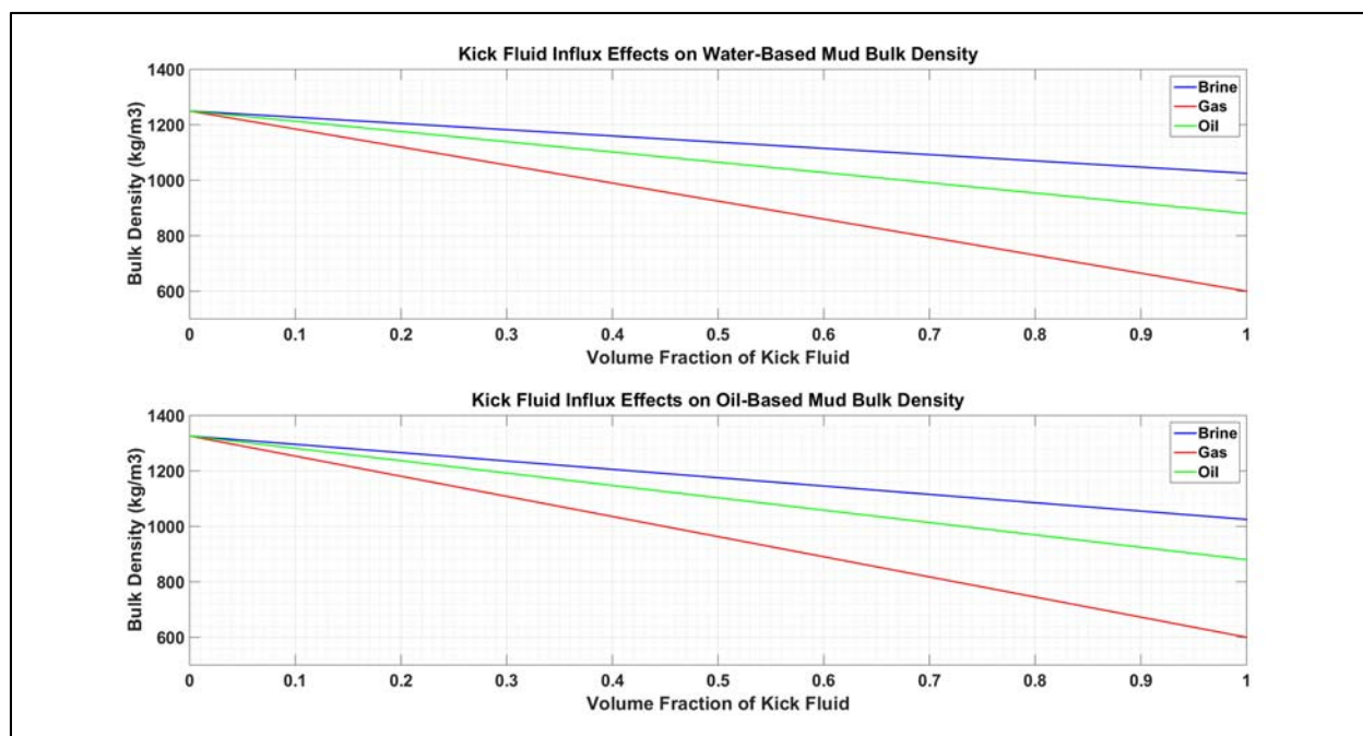
Figure 1: Effects of kick fluid mixing on drilling fluid bulk density.
