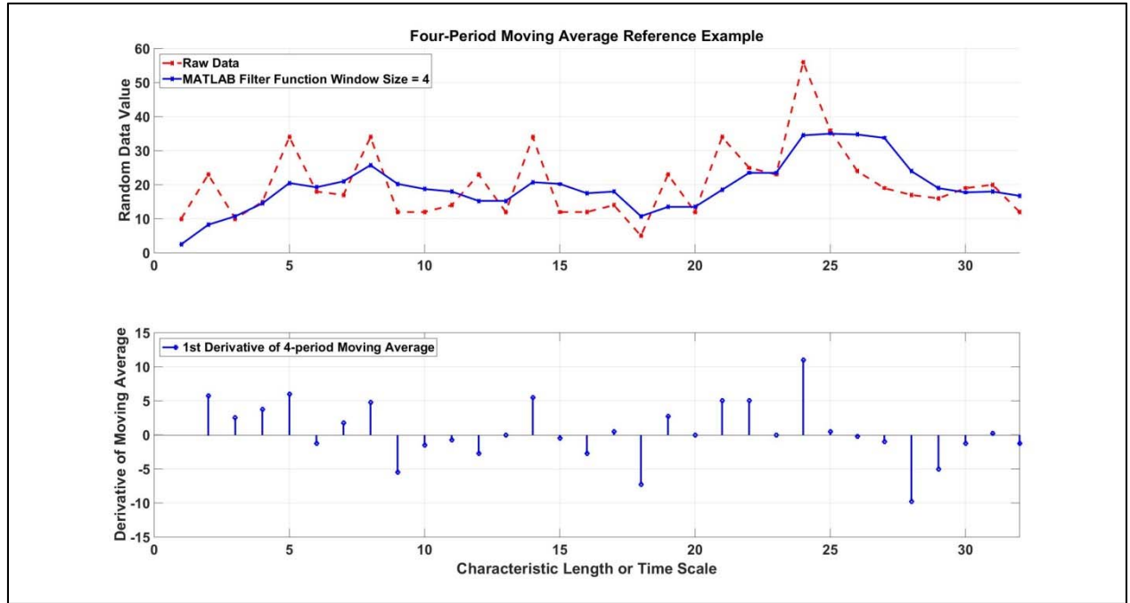
Figure 6: Moving average differential for kick identification.
