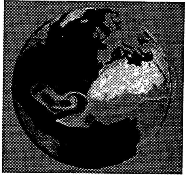
Figure 3. Flow volume for winds in a global climate simulation.
