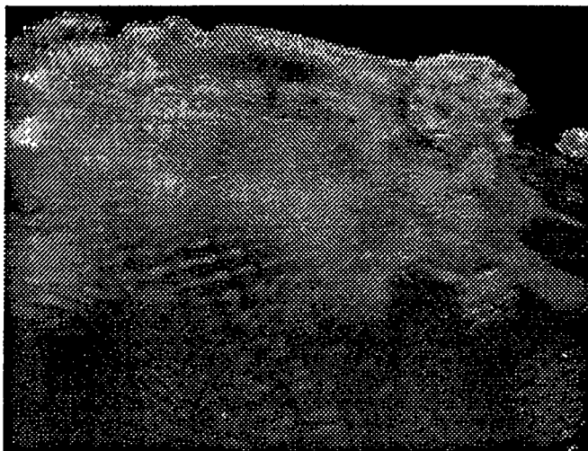
Figure 4. Wind velocity in global climate simulation, indicated by textures splats whose scalar component indicated percent cloudiness.
