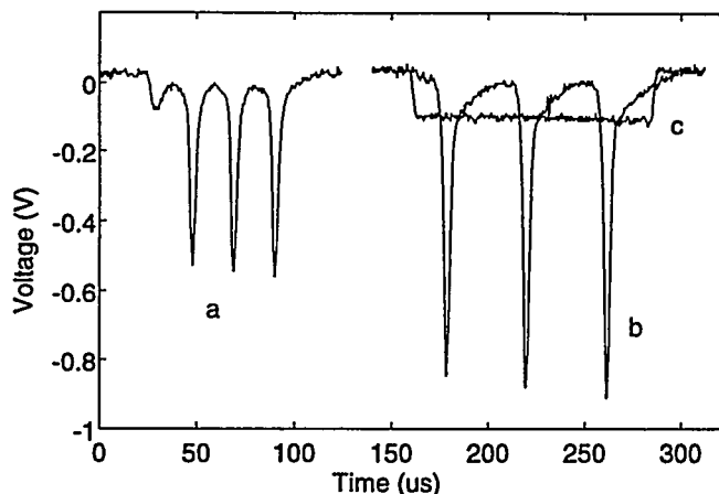
Fig. 4. Digital recording of oscilloscope trace; (a) AAC at 130 kV and 92.2116 MHz, dee at 23.06457; (b) at 140 kV and 92.282 MHz, dee frequency 23.06441 MHz; (c) AAC off.
