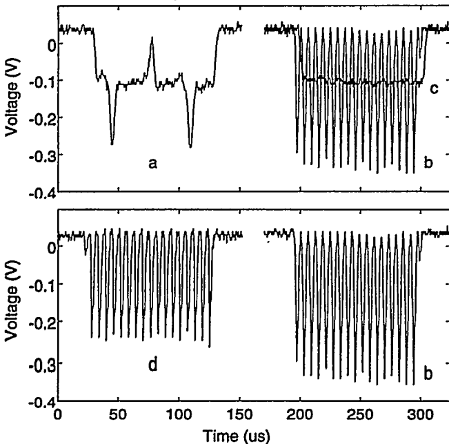
Fig. 5. RFD at (a) 11.54 MHz, HE2 probe at 299.15 inch radius; (b) 11.45 MHz, probe at 301.94 inch, beat period 6.1 \mu s; (c) RFD off, note the longer flight time to the probe; (d) as (b), but with 30% beam intercepted by HE1.
