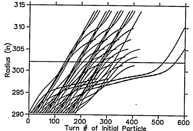
Fig. 6. Radii calculated by GOBLIN of particles started 6.5 \mu s apart for AAC asynchronous with the main dee.
