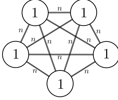
Figure 1. The 3d mirror of (A_{k-1}, A_{kn-1}) theory. k is the number of nodes and n is the number of bifundamentals between a pair of nodes. One of the U(1) has to be decoupled.
