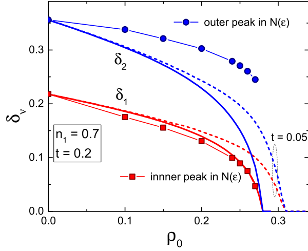
FIG. 5. (Color online) Peak positions of DOS N(\varepsilon) vs \rho_0 marked as dots along with the bands order parameters |\delta_{1,2}| , solid lines for t = 0.2 . The dashed lines are |\delta_{1,2}| for t = 0.05 .
