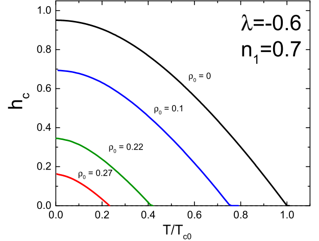
FIG. 10. (Color online) The thermodynamic critical field h_c(t) = H_c/H_{c0} for n_1 = 0.7 and \lambda = -0.6 .
