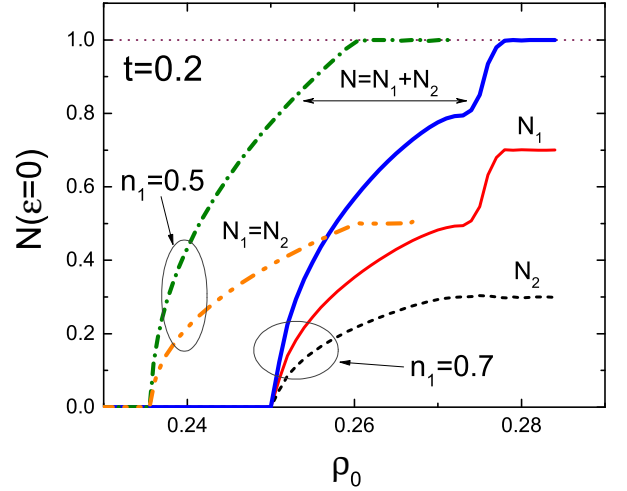
FIG. 7. (Color online) At the left: the zero-bias DOS (normalized to N_n ) as a function of \rho_0 for \lambda = -0.6 , t = 0.2 , and n_1 = 0.5 ; in this case, \tilde{\rho} \approx 0.236 and \rho_c \approx 0.26 so that for 0.236 < \rho_0 < 0.26 the superconductivity is gapless. At the right: DOS( \rho_0 ) at zero energy for the same \lambda and t , but n_1 = 0.7 .
