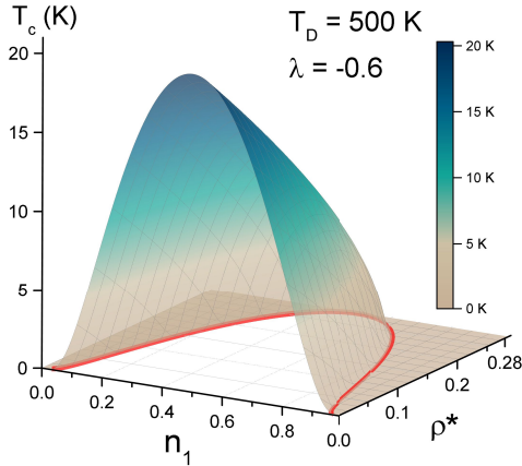
FIG. 1. (Color online) T_c(n_1, \rho^*) for T_D = 500 K, \lambda = -0.6 . The red line at the dome base gives the critical value of \rho_{cr}^* = 1/2\pi T_{c0}(0.5)\tau_{cr} at which the superconductivity is destroyed. For n_1 = 0.5 , \rho_{cr}^* = e^{-\gamma}/2 = 0.28 and the critical rate is 1/\tau_{cr} = \Delta_0(0) , \Delta_0(0) is the order parameter of clean material with n_1 = n_2 at T = 0 .
