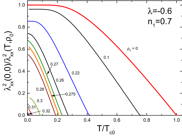
FIG. 12. (Color online) The inverse square of the in-plane penetration depth normalized on the zero- T clean limit value vs t = T/T_{c0} for a set of scattering parameters \rho_0 . In this calculation \langle v_x^2 \rangle_1 / \langle v_x^2 \rangle_2 = 1 and the intraband \rho_{11} = \rho_{22} = 0 .
