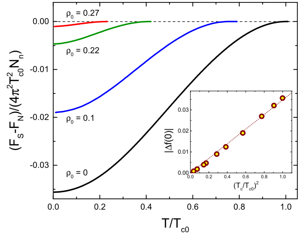
FIG. 9. (Color online) The temperature dependence of the condensation energy normalized on 4\pi^2 T_{c0}^2 N_n for n_1 = 0.7 and a set of scattering parameters \rho_0 . The inset shows that the normalized condensation energy at T = 0 scales approximately as T_c^2 .
