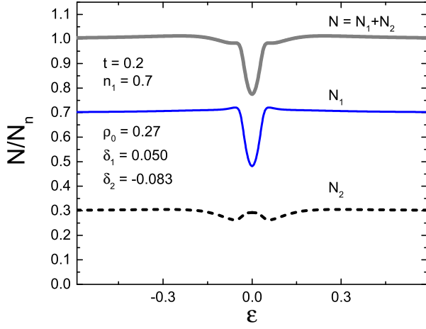
FIG. 6. (Color online) The density of states N normalized on N_n vs energy \varepsilon (in units 2\pi T_{c0} ) for n_1 = 0.7 , t = 0.2 in the gapless state with \rho_0 = 0.27 .
