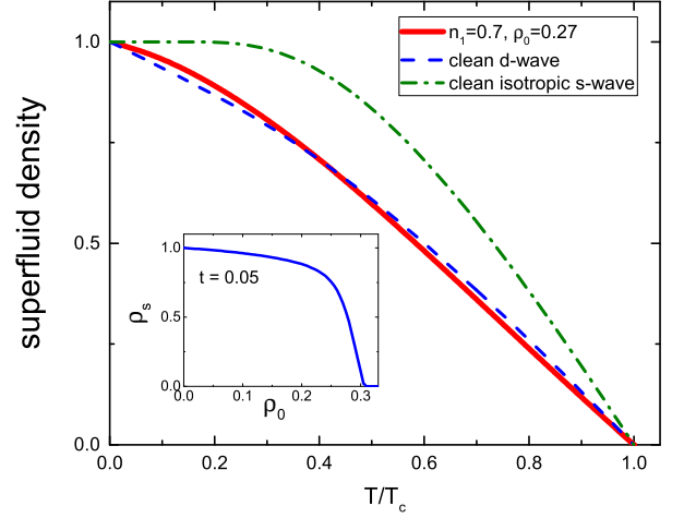
FIG. 13. (Color online) The superfluid density \rho_s vs t = T/T_{c0} for n_1 = 0.7 and \rho_0 = 0.27 of the gapless state normalized on the value at T = 0 . Superfluid densities for s- and d-wave clean cases are shown for comparison.
