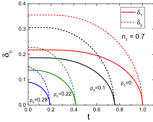
FIG. 3. (Color online) |\Delta_\nu|/2\pi T_c vs t = T/T_{c0} for \lambda = -0.6 , n_1 = 0.7 and a few values of \rho_0 = 1/2\pi T_{c0}\tau .
