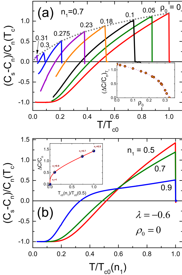
FIG. 11. (Color online) The upper panel: the specific heat vs T/T_{c0}(0.7) for a few scattering parameters \rho_0 . The lower panel: the specific heat vs T/T_{c0}(n_1) for n_1 = 0.5, 0.7 and 0.9 . Inset: the specific heat jump at the critical temperature calculated numerically (dots) and according to Eq. (52), the solid line.
