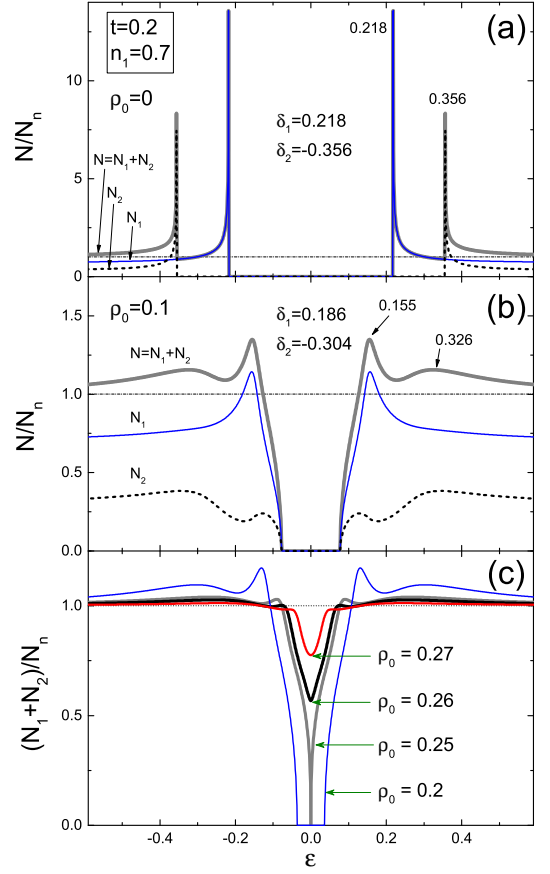
FIG. 4. (Color online) (a) The clean limit DOS as a function of energy \epsilon = \epsilon/2\pi T_{c0} for \lambda = -0.6 and n_1 = 0.7 at t = 0.2 . (b) The same as (a), but for the interband scattering parameter \rho_0 = 0.1 . The bands order parameters for this case are \delta_1 = 0.186 , |\delta_2| = 0.304 ; N(\epsilon) has a typical two-band shape, although the two maxima do not exactly positioned at |\delta_{1,2}| . (c) The total DOS for a set of scattering parameters \rho_0 . Note that with increasing scattering, in the gapless state, the DOS acquires a V-shape with a non-zero minimum.
