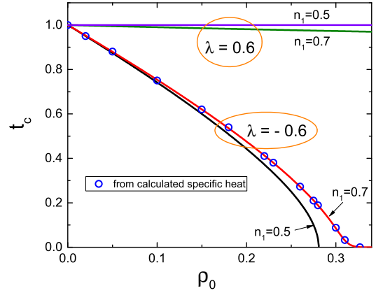
FIG. 2. (Color online) t_c = T_c/T_{c0} versus \rho_0 according to Eqs. (30)-(32). Lower curves are for \lambda = -0.6 ; the black line is for the partial DOS n_1 = 0.5 , the red line is for n_1 = 0.7 . The upper curves are for positive (attractive) interband coupling constant \lambda = 0.6 . The dots are obtained by independent calculation of the specific heat jumps.
