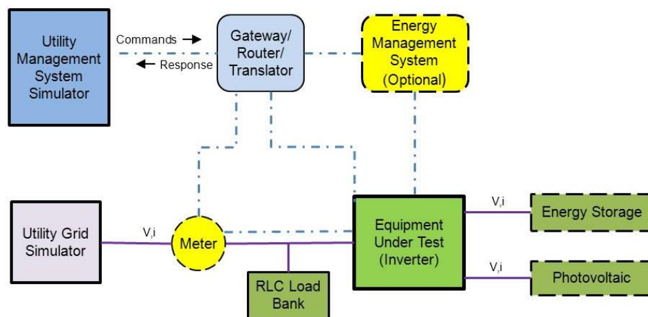
Figure 1. Interoperability Test System.
