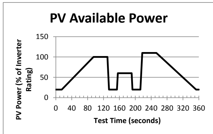
Figure A2- 1. Input PV Power Curve.
