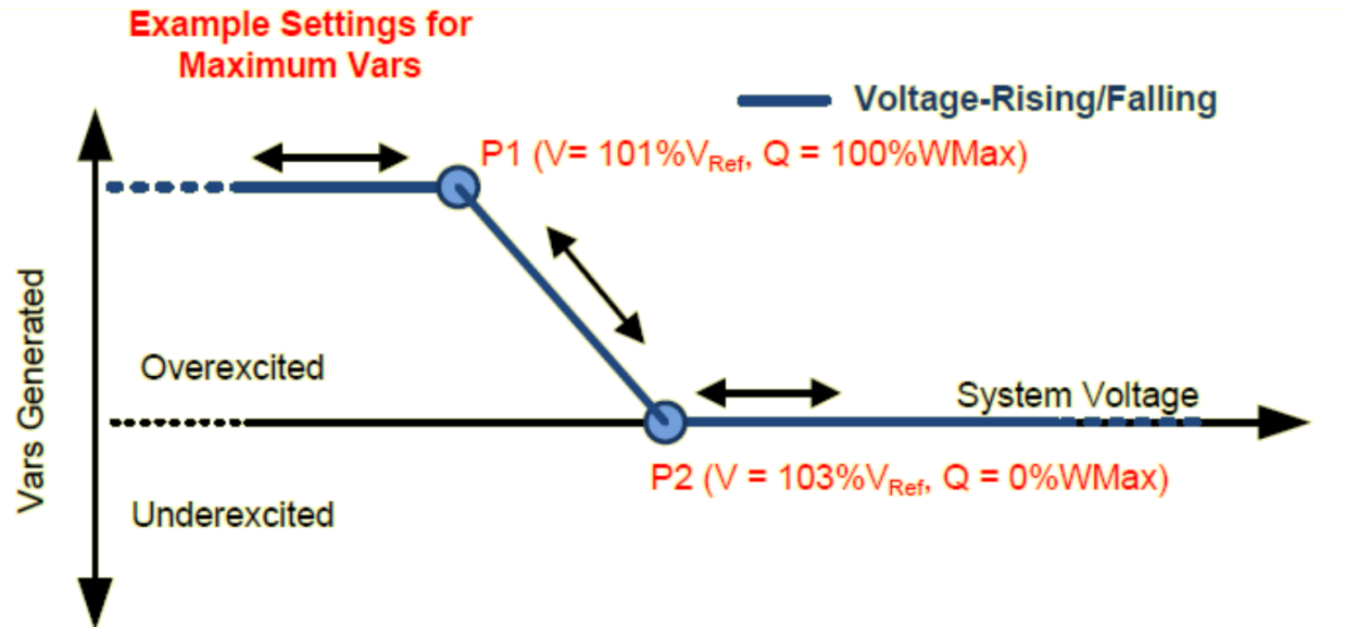
Figure A6-2. Example Volt/Var Array for VV12
