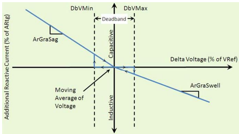
Figure A8-4. Alternative reactive current support behavior
