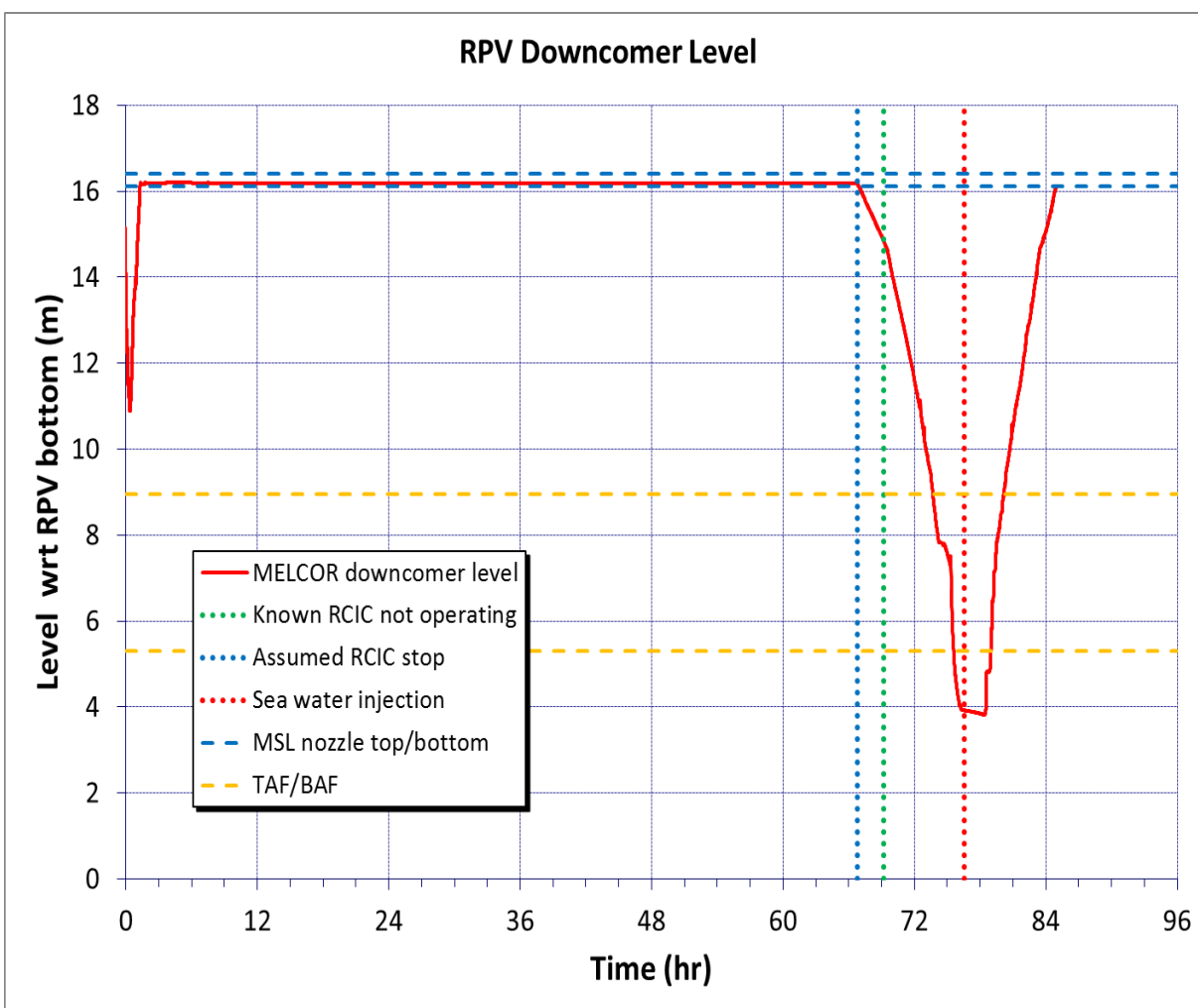
Figure 3 RPV Downcomer Level
