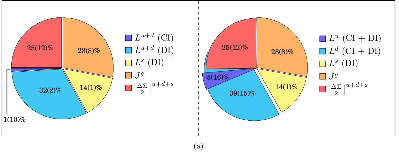
Figure 2: Pie charts for the quark spin, quark orbital angular momentum and gluon angular momentum contributions to the proton spin. The left panel show the quark contributions separately for CI and DI, and the right panel shows the quark contributions for each flavor with CI and DI summed together for u and d quarks.
