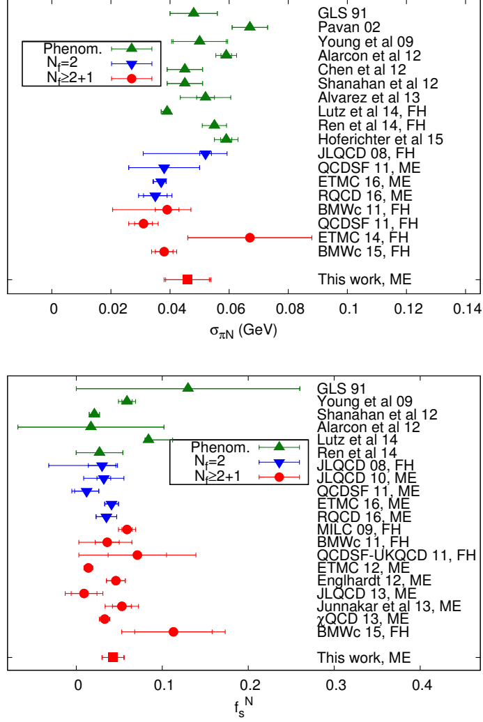
Figure 1: The results of \sigma_{\pi N} (upper panel) and f_s^N (lower panel) from both phenomenology and lattice simulations. The narrow error bar for each data point is the statistical, and the broad one is that for the total uncertainty. The physical proton mass 938MeV is used to obtain f_s^N in this work. They are color-coded in phenomenological and indirect approaches (green), N_f = 2 lattice calculations (blue), and N_f = 2 + 1 lattice calculations (red). Detailed references are given in Ref. [19].
