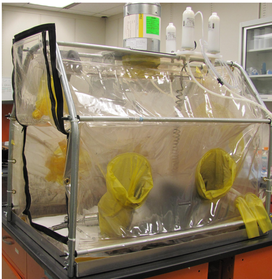
Figure 7. Exterior image of the HEPA-filtered tent, showing duct to local exhaust.
