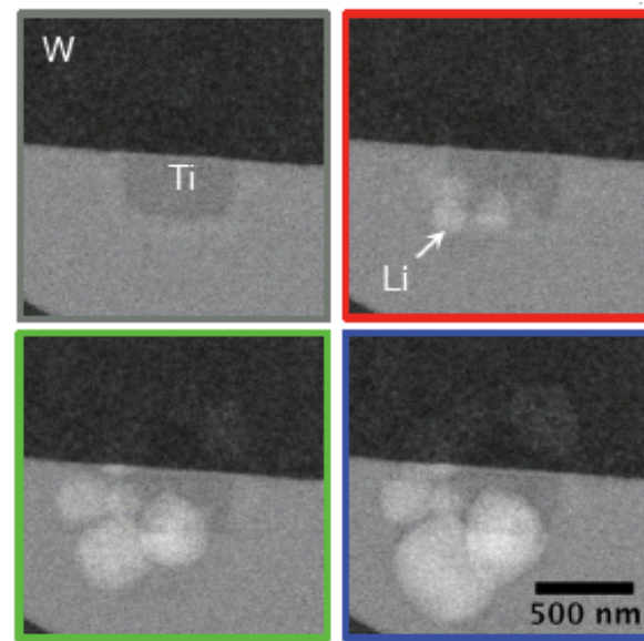
TEM images of Li growth during charging
