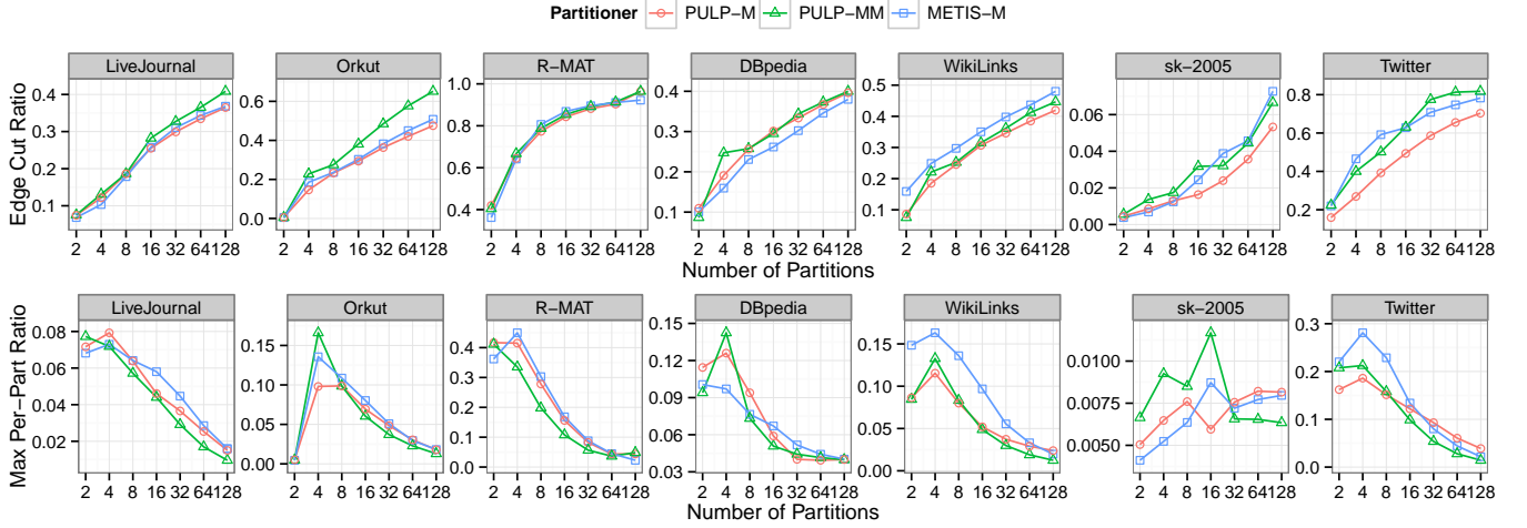
Fig. 2. Quality metrics of total cut edge ratio (top) and maximum per-partition edgecut ratio (bottom) for PULP-M, PULP-MM and METIS-M.
