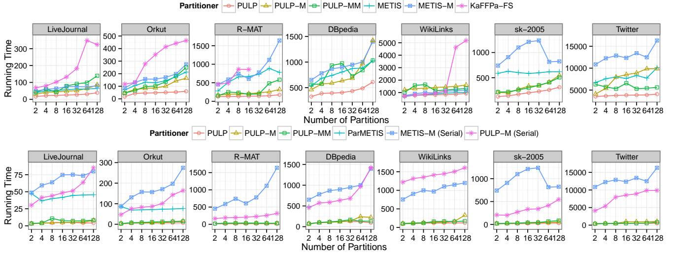
Fig. 1. Partitioning times with PuLP, METIS, and KaFFPa. Top: Comparison of serial running times. Bottom: Parallel and Serial running times.
