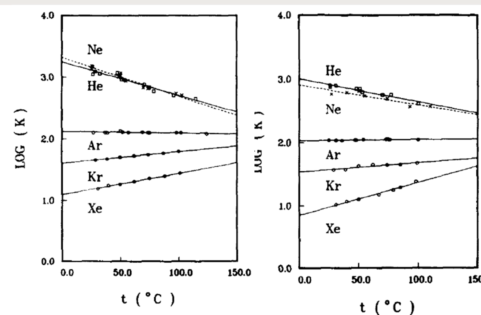
Noble gas solubility in heavy (L) & light (R) oil Kharaka & Specht (1988)
