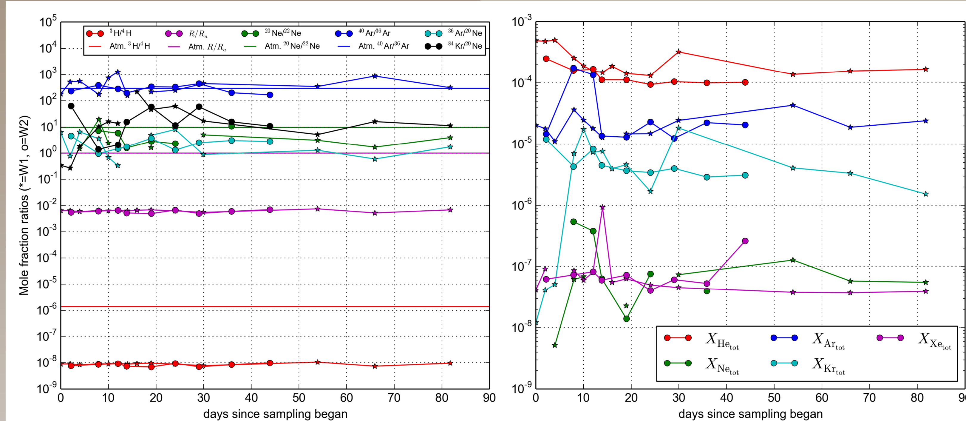
Noble gas isotopic ratios (left) and totals (right) for both wells (Well 1 stars, Well 2 circles)
