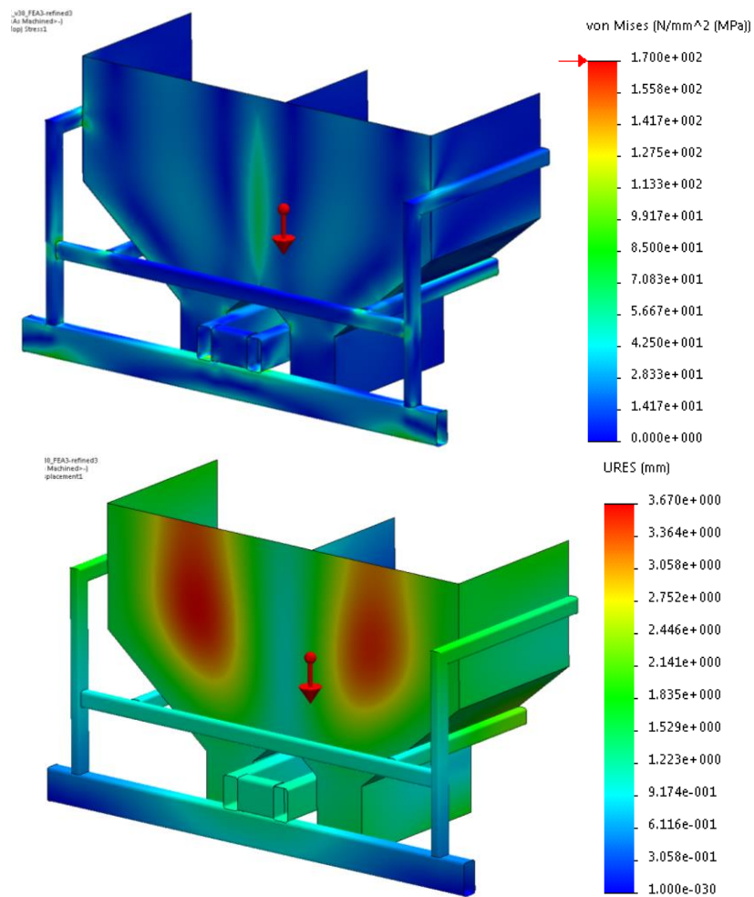
Figure 5. (Top) Thermal and dead loading stresses (MPa) in top hopper, (Bottom) Displacements (mm) in bottom hopper due to loading
