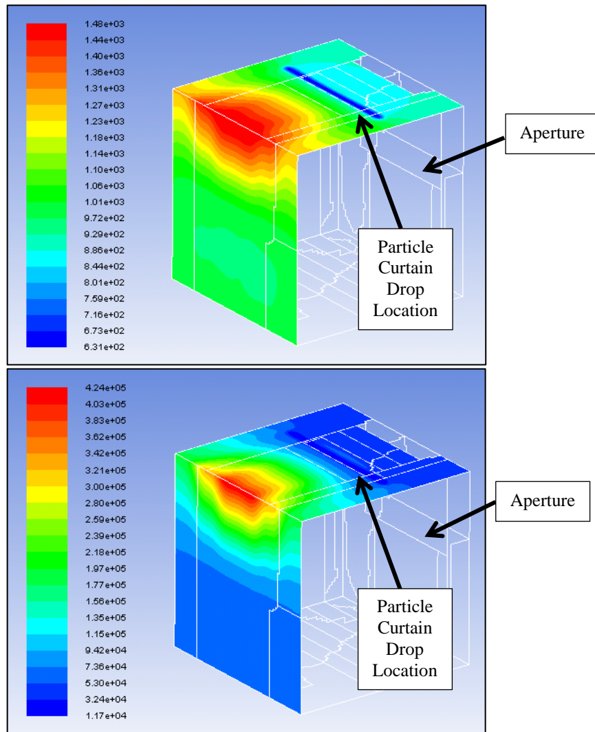
Figure 2. 2 m x 2 m x 2 m, 4 kg/s total particle mass flow rate, (Top) Cavity wall temperatures (K) of top and back wall showing high temperature at the joint of the back and top walls, (Bottom) Surface incident radiation ( \text{W/m}^2 ) on top and back wall showing the high flux concentration on the same joint with high temperatures
