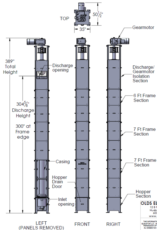
Figure 7. Design of the Olds particle elevator (dimension in inches)
