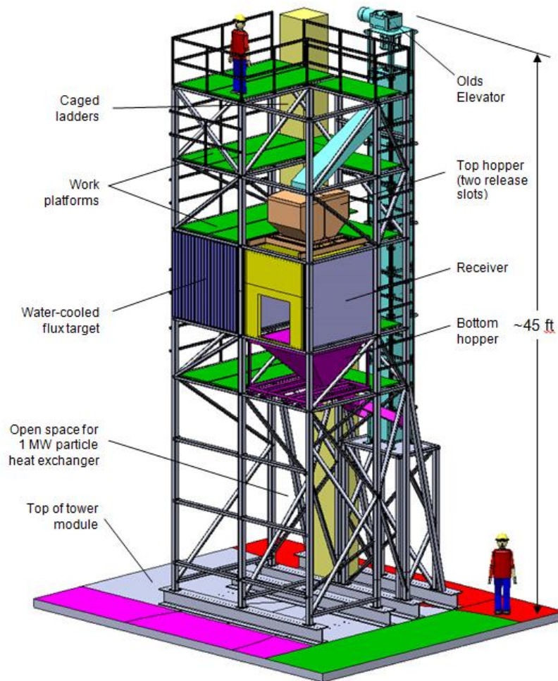
Figure 1. Prototype structure including work platforms and ladders (green and light yellow), bottom hopper (purple), top hopper (light brown), OLDS elevator (light blue), NSTTF module (multi-colored platform at the base; see Figure 1 for color codes). Heat shielding around the receiver and flux target is not shown. This system will be lifted on the module to the top of the 200 ft tower at Sandia's NSTTF.
