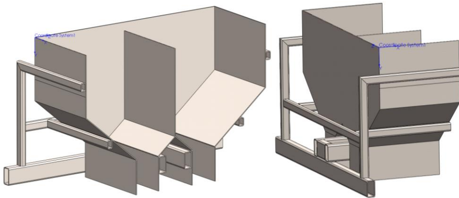
Figure 4. Top Hopper geometry, Isometric views showing inside (left) and outside (right) of symmetrical geometry
