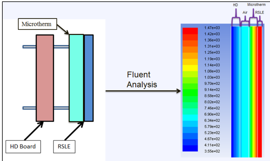
Figure 3. Cavity wall structure composition and thermal analysis (K)
