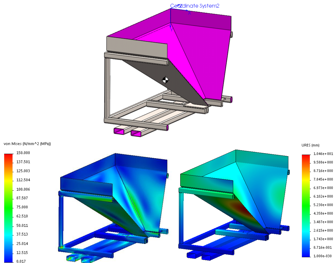
Figure 6. (Top) Half-symmetric bottom hopper geometry, purple surfaces designating inside of hopper; (Bottom-Left) Stress (MPa) contours with thermal and dead loading; (Bottom-Right) Displacement (mm) contours with thermal and dead loading
