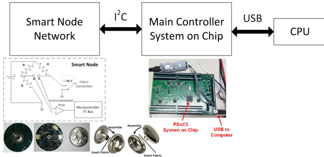
Figure 2: Smart nodes (embedded within fabric snaps) are used at each sensing point on the conductive fabric sensing layer to provide a means for making resistance measurements and relaying the resistance data back to the main controller. A front-end instrumentation amplifier connected to a Wheatstone bridge provides stable resistance measurements across the surface area of the WCS. Images courtesy ORNL.
