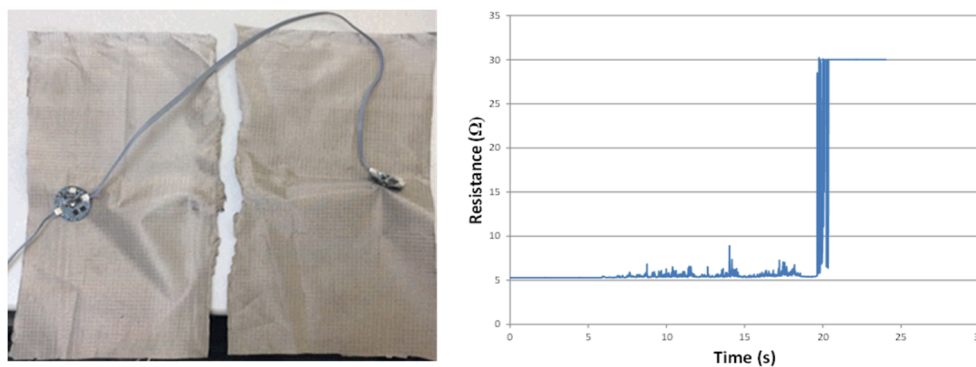
Figure 4: (Left) A \sim 0.30 m x 0.30 m fabric sheet in which two smart nodes are placed on the left and right sides of the sheet, and a cut is made down the middle of the sheet. (Right) Resistance measured between the two smart nodes over a 25 second time period in which the cut is made during the time interval from 6 – 20 seconds. Images courtesy ORNL.
