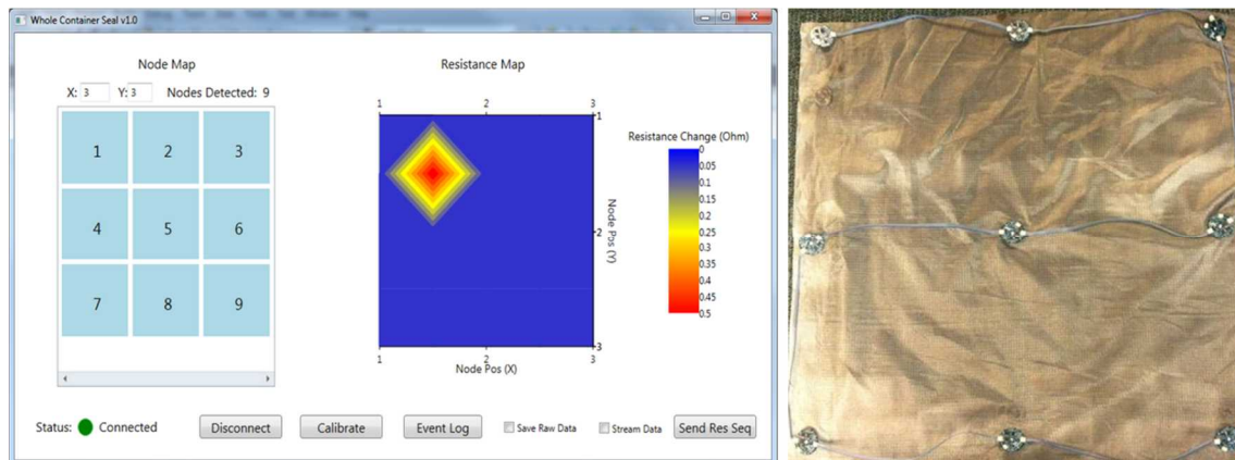
Figure 3: (Left) Software for communicating with the WCS, interfacing with smart nodes, visualizing data, and logging data and alarms. (Right) Smart nodes connected in a grid pattern where one cable is strung between the smart nodes and connected to the main controller. Images courtesy ORNL.
