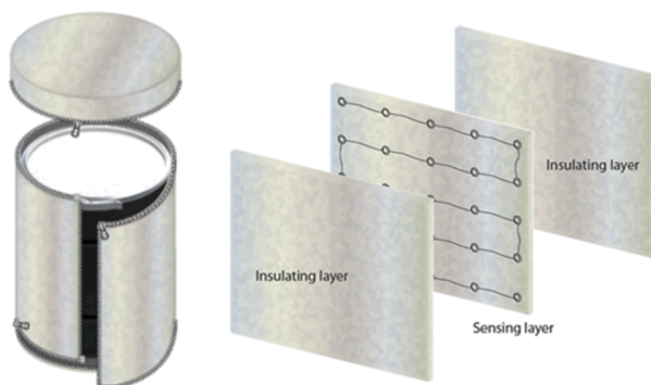
Figure 1: (Left) Conceptual design of the WCS where the sensing system is embedded into the fabric comprising the seal. The seal is scalable for use in sealing containers of various sizes. (Right) Multilayer fabric structure. Images courtesy ORNL.
