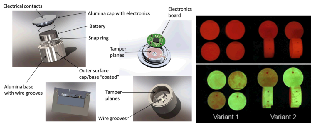
Figure 5: (Left) The Ceramic Seal design features. (Right) Ceramic Seals are shown on top uncoated, with alumina based sol gel doped with terbium coatings on the bottom. Excited by 254 nm UV. Images courtesy Tetramer Technologies.
