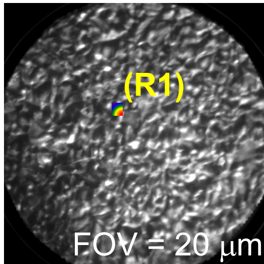
CuInGaSe 2 Photoemission Image
