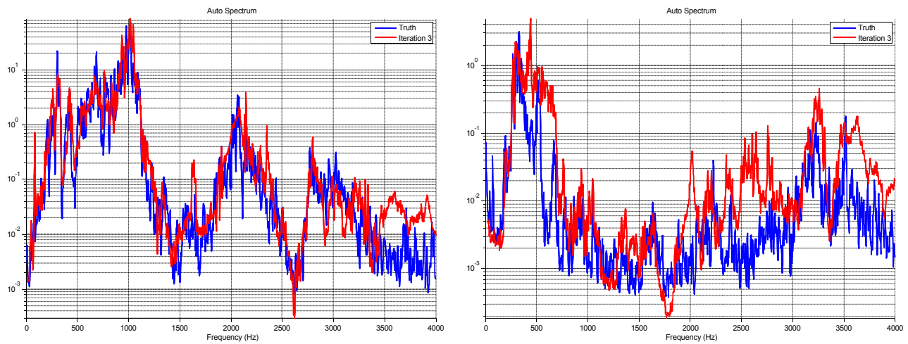
Figure 5 - Individual Acceleration Spectral Density - Best (left) and Worst (Right) Comparisons of Acoustic Test (blue) and Vibration Test (red)
