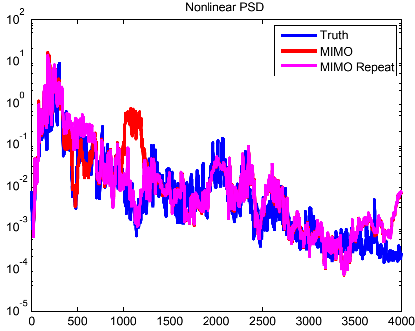
Figure 6 - PSD with Intermittent Nonlinearity - Acoustic Test (blue) Vibration Test (red) - Repeat of Vibration Test (magenta)
