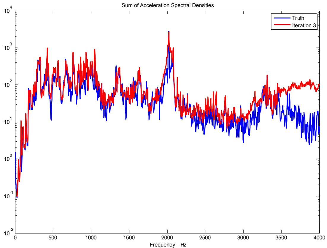
Figure 4 - Comparison Metric (Sum of PSDs) for 37 accelerometers for the Acoustic Test (blue) and 6 Shaker Vibration Test (red)
