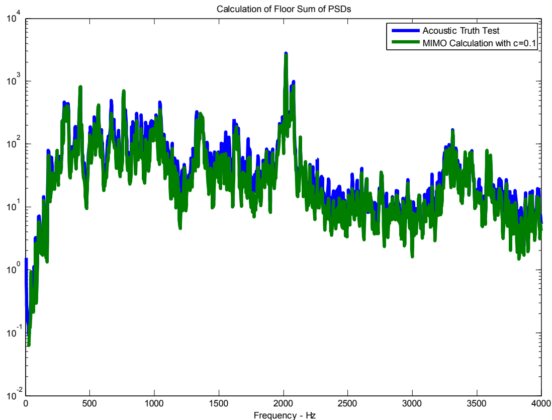
Figure 12 - Calculated Sum of PSDs Match for 6 Floor Mounted Shakers and Tikhonov c value of 0.1
