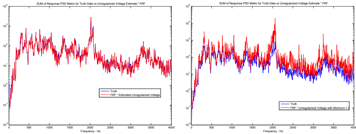
Figure 7 - Mathematical Prediction of Sum of Acceleration PSDs Result with Some Negative Autospectra (left) - Result with All Autospectra Positive (Right)
