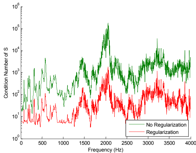
Figure 8 - Condition Number of the S Matrix with and without Regularization
