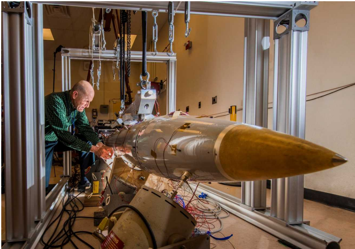
Figure 1 - Industrial Structure Mounted on Support Rack in One Test Configuration
