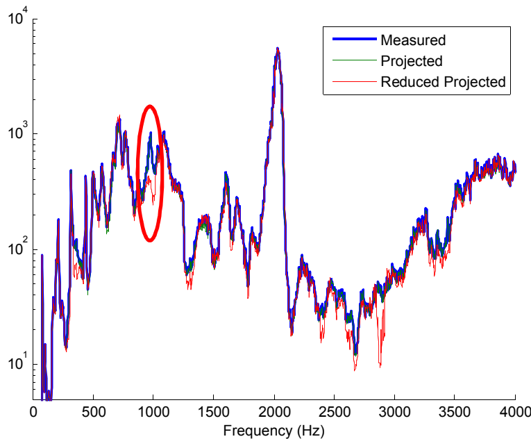
Figure 10 - Sum of 37 PSDs from some Measured Data (blue), Mathematical Prediction from Voltage Calculated Using All 37 Responses (green), Mathematical Prediction from Voltage Calculated Using 12 Responses (red)
