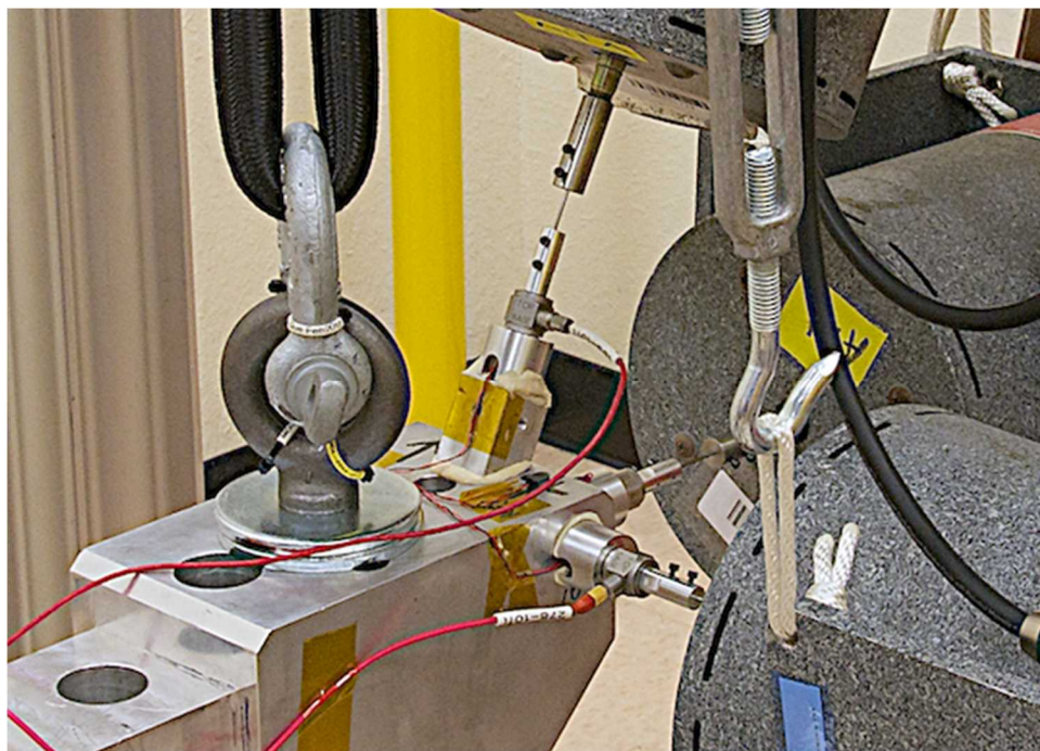
Figure 2 - Shaker Attachment Hardware
