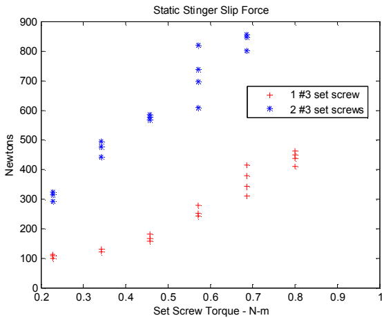
Figure 11 - Static Stinger Slip Force vs Set Screw Torque
