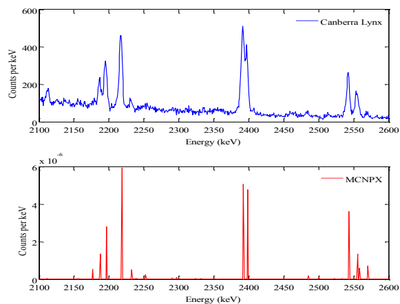
Figure 3.9 Comparison between measured and simulated delayed gamma spectra (2.1 MeV-2.6 MeV, ^{238}\text{U} ).
