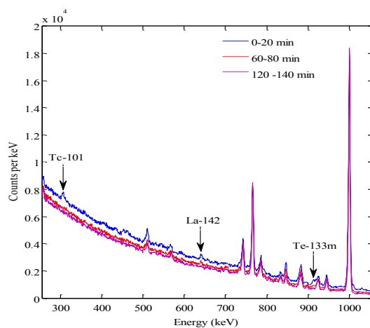
Figure 2.39 Measured delayed gamma spectra with the list-mode system (0.3 MeV-1.0 MeV, DU).
