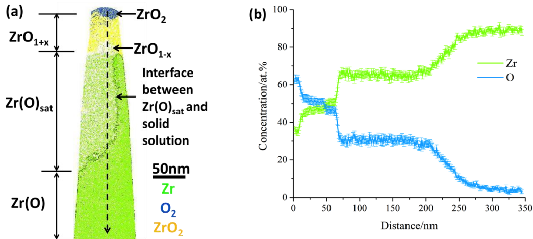
Figure 9: Zircaloy-4 oxide region: (a) 10 nm slice from an APT reconstruction showing the presence of different oxide phases; (b) concentration profile taken along the arrow indicated in (a).
