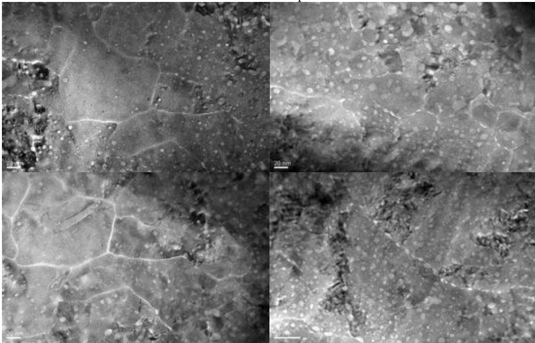
Figure 5: Higher magnification images of the Zry-4 sample following 40 minutes at 800°C taken from multiple locations.
