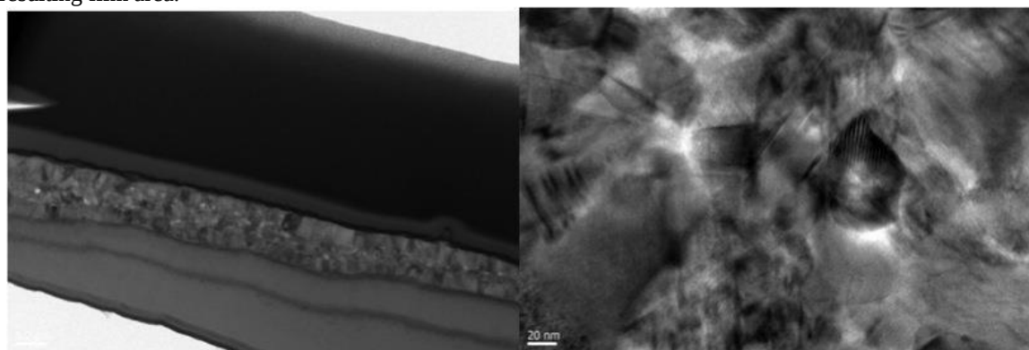
Figure 9: Overview TEM image showing a cross section from a thin Ti TEM sample. Image on the right shows a higher magnification image of the cross section of the sample.
