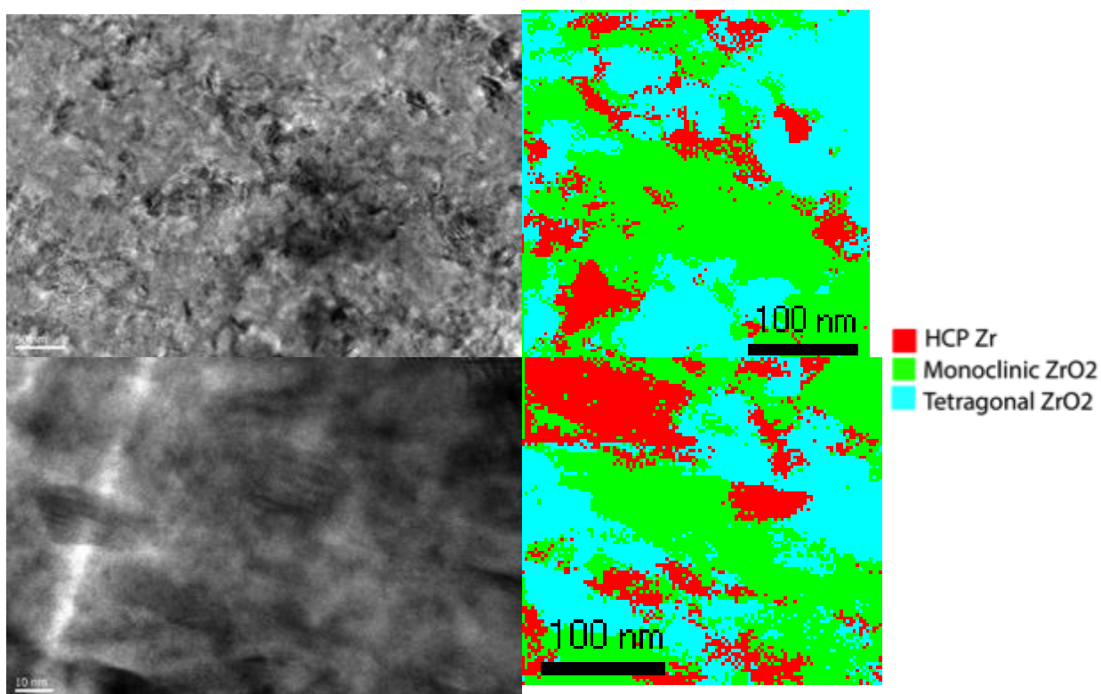
Figure 8: TEM images and corresponding phase maps for in-situ and ex-situ corroded samples. The in-situ sample is represented by the top two images, the autoclave corroded sample is shown in the bottom two images.
