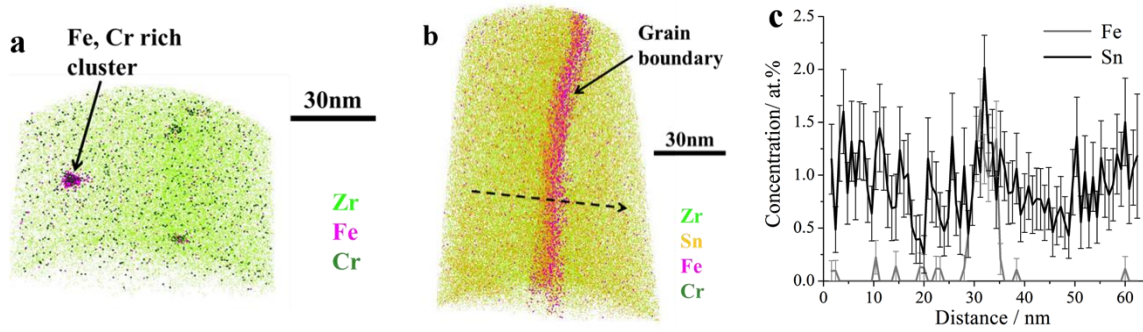
Figure 4: Bulk Zircaloy-4: (a) APT reconstruction showing Fe,Cr rich clusters; (b) APT reconstruction showing grain boundary with Fe and Sn segregation; (c) line profile across grain.
