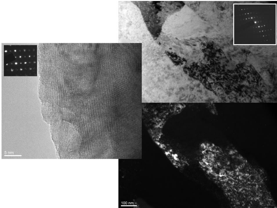
Figure 1: TEM brightfield/darkfield pairs (with corresponding diffraction), and high-resolution image (with corresponding diffraction) of oxide layers in as-corroded Zircaloy-4.
