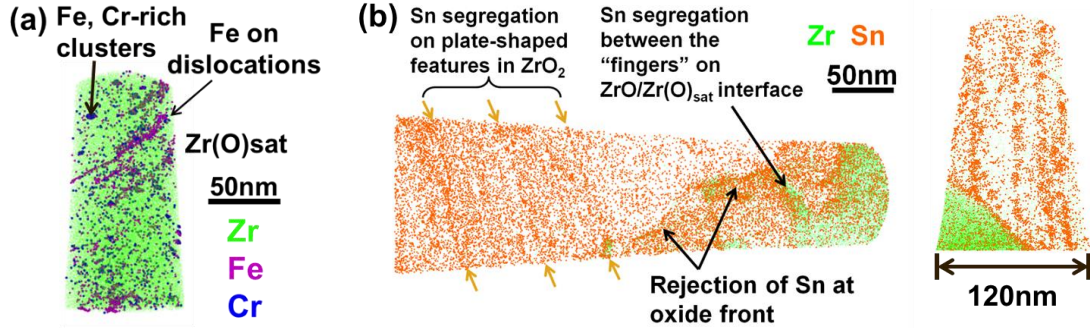
Figure 14: (a) APT reconstruction showing segregation of Fe at dislocations and Fe, Cr rich clusters in Zr(O) sat ; (b) 10 nm slices taken from two distinct APT reconstructions showing distribution of Sn.
