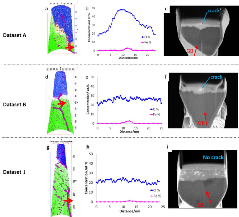
Fig. 23: Three representative APT reconstructions from crystal bar Zr (dataset A and B) and ZrFeCr (dataset J). The Fe and O concentration profiles (b, e, h) were measured by placing a 10nm diameter cylinder along the
