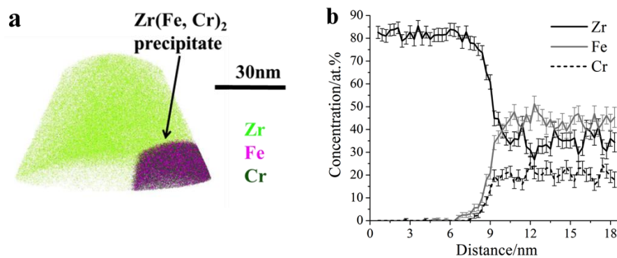
Figure 5: Bulk Zr-Fe-Cr: (a) APT reconstruction showing part of an Fe, Cr rich intermetallic precipitate; (b) line profile across the precipitate interface.
