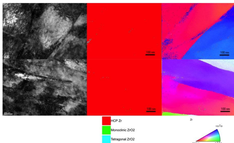
Figure 13: Bright field TEM image with corresponding phase and orientation maps resulting from precession diffraction scans showing multiple grains present in a FIB sample.
