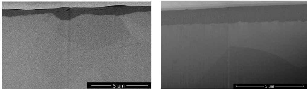
Figure 19: SEM images of (left) 7 days pure Zr sample showing the faster oxide growth along grain boundary; (right) ZrFeCr sample showing no preferential oxidation along grain boundary.
