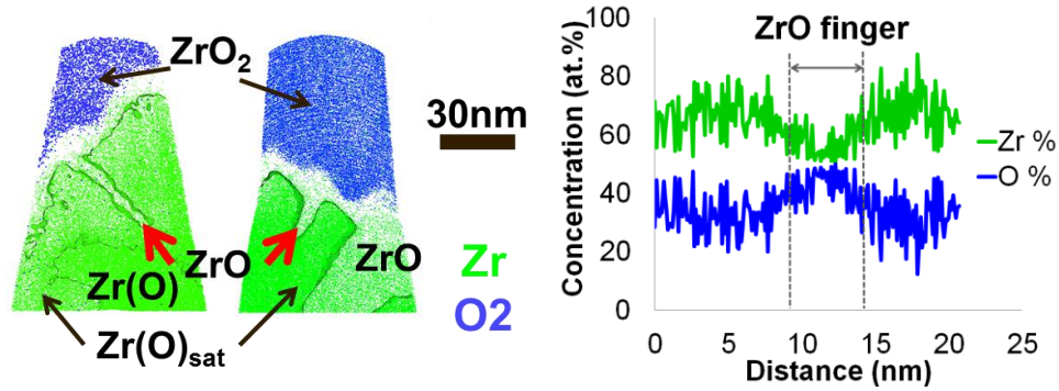
Figure 8: (left) 10 nm slices of two representative APT datasets taken from 7 day crystal bar Zr revealing the presence of ZrO fingers at \text{ZrO}_2/\text{Zr(O)}_{\text{sat}} interface; (right) concentration profile of Zr and O across the ZrO finger.
