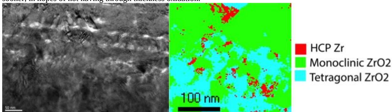
Figure 10: TEM image of the cross section from an in-situ sample and the corresponding phase map showing through thickness oxidation of the in-situ TEM sample
