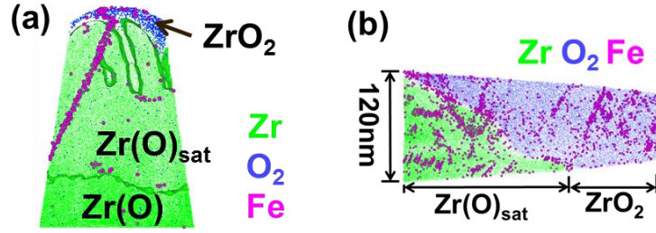
Figure 16: Zr-Fe-Cr oxide region: (a) 10 nm slice one from APT reconstruction showing the Fe segregation at grain boundary of \text{Zr(O)}_{\text{sat}} ; (b) APT reconstruction showing the Fe segregation on dislocations in \text{Zr(O)}_{\text{sat}} and Fe clustering on planar features in \text{ZrO}_2 .
