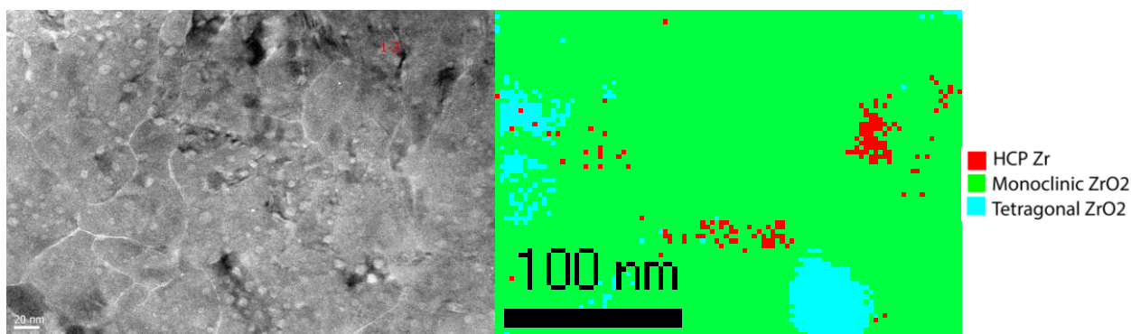
Figure 6: TEM image (on left) showing the region over which the Nanomegas scan was taken to create the phase map (on right).
