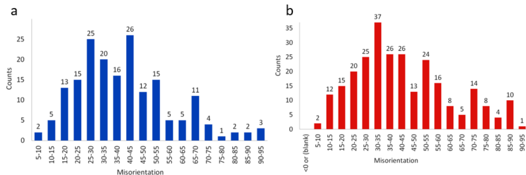
Figure 22: Distribution of grain boundary misorientation angles in (a) crystal bar Zr and (b) ZrFeCr.
