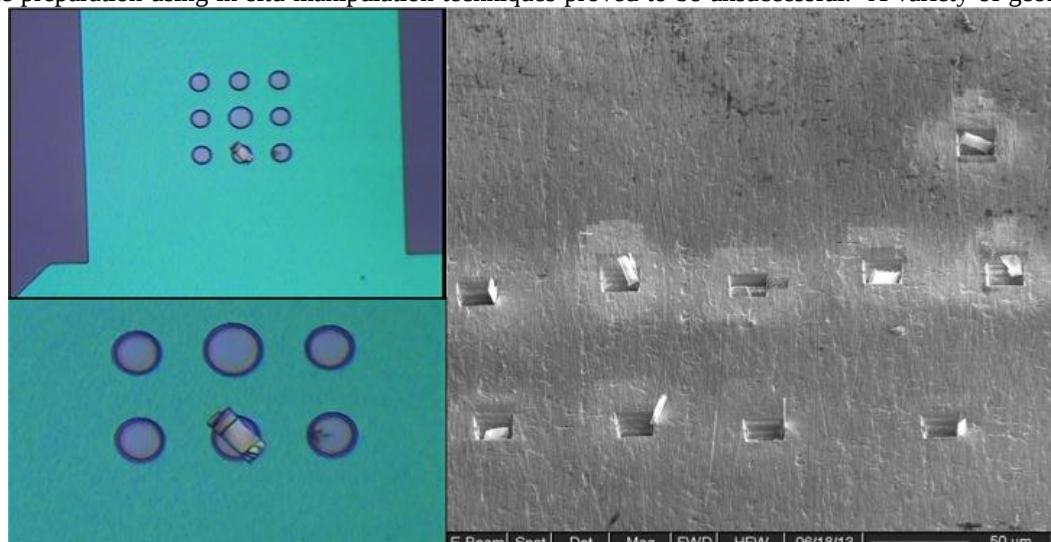
Figure 2: FIB image on right shows lamella cut loose and prepared for ex situ liftout. The two images on the left show a FIB sample successfully lifted out and placed over an electron transparent window on the E-chip
