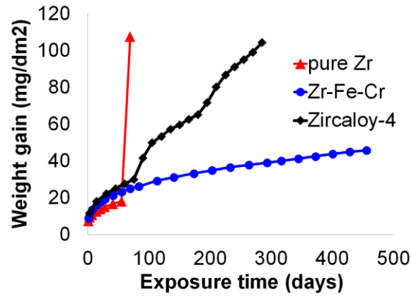
Figure 1: Corrosion weight gain-exposure time for studied alloys oxidized in 360°C water.
