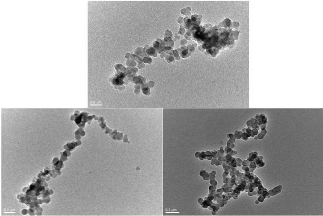
Figure 17: TEM images showing the initial morphology of soot particles intended for humidity testing of the environmental cell holder
