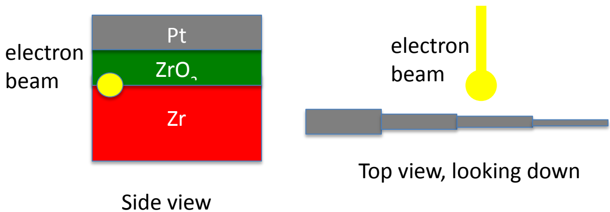
Figure 15: Schematic showing the appearance of a sample used for studying the stability of a tetragonal \text{ZrO}_2 in thin TEM samples.
