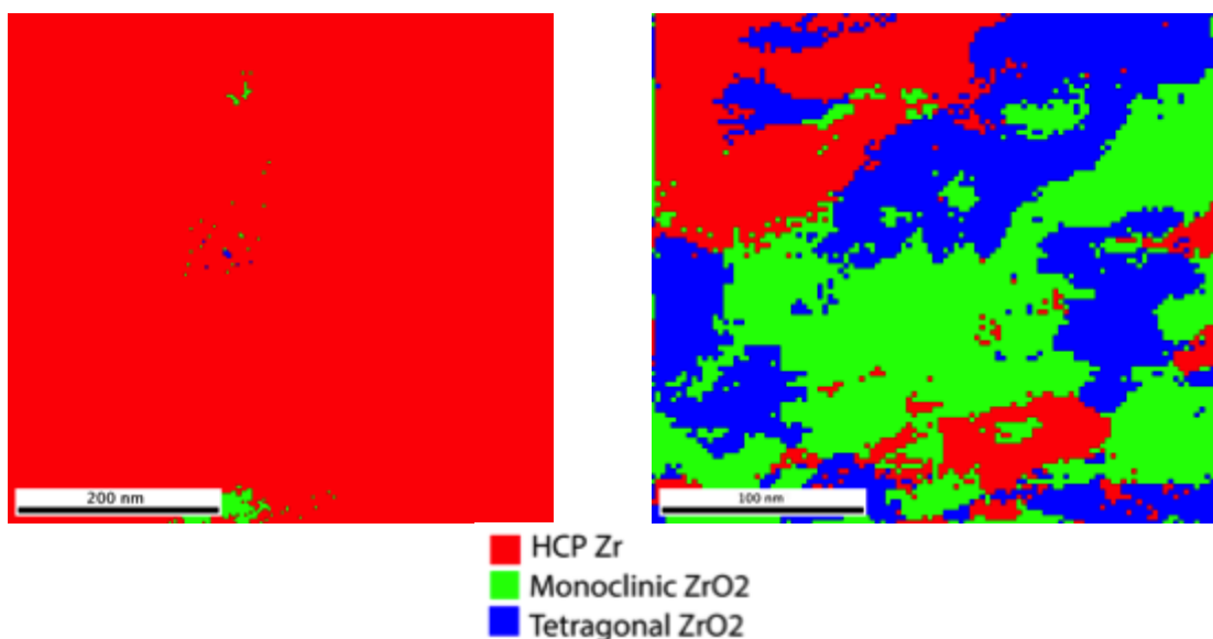
Figure 11: Phase maps for an in-situ sample. On left the phase map for a pristine sample, on right, a phase map for the same sample following an in-situ oxidation experiment
