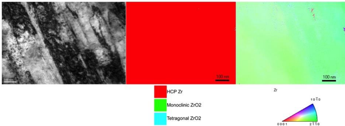
Figure 14: Bright field TEM image with corresponding phase and orientation maps resulting from a precession diffraction on a pure Zr FIB sample.
