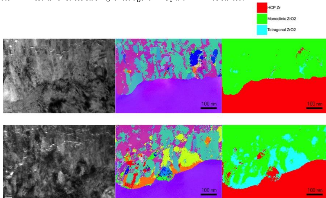
Figure 16: TEM images and corresponding precession diffraction scans showing the stability of tetragonal \text{ZrO}_2 in TEM samples. The top row of images shows the results from the thinnest section of the sample, while the lower row shows the sample information for a thicker region of the sample.
