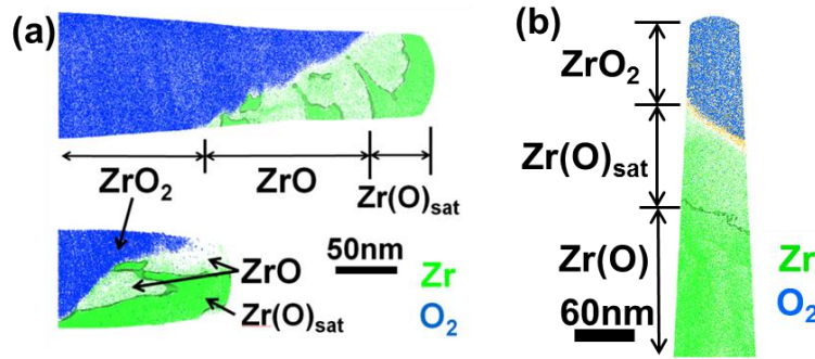
Figure 10: 10 nm slices from APT reconstructions showing the presence of different oxide phases and interface morphologies in (a) 60 days and (b) 90 days Zircaloy-4.
