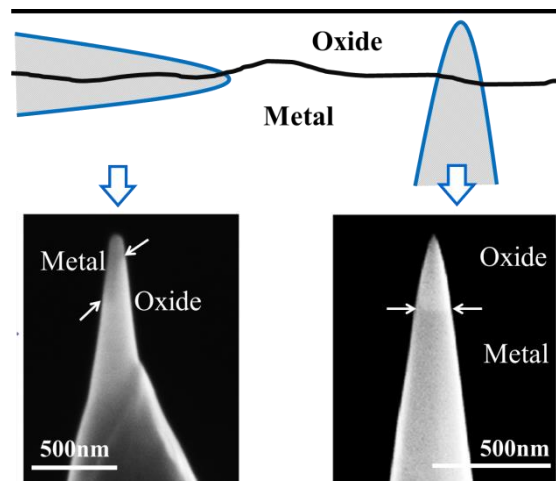
Figure 2: Schematic illustration and SEM images of the two orientations chosen for the APT specimens
