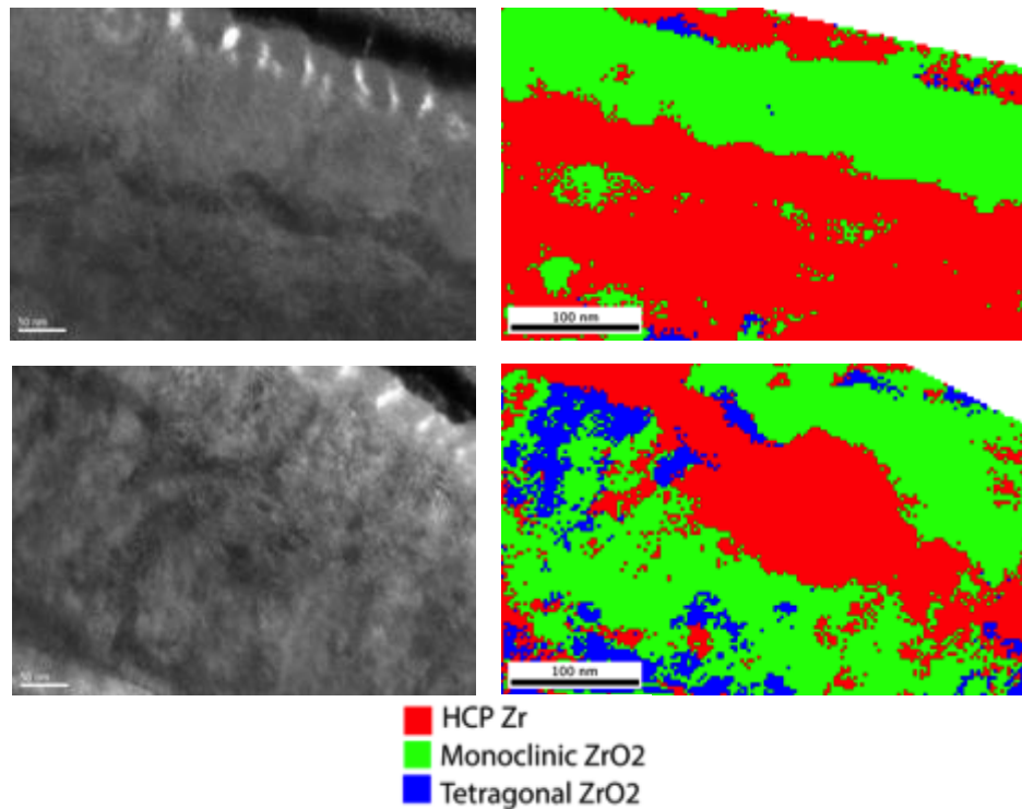
Figure 12: TEM images and corresponding phase maps for two different areas from a cross section of the sample seen in figure 11 showing oxide thickness and phases present.
