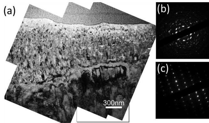
Figure 25: (a) TEM bright field image of 7 day ZrFeCr; (b) electron diffraction pattern taken from oxide layers when the metal grains were tilted to [-12-10] zone axis as shown in (c).
