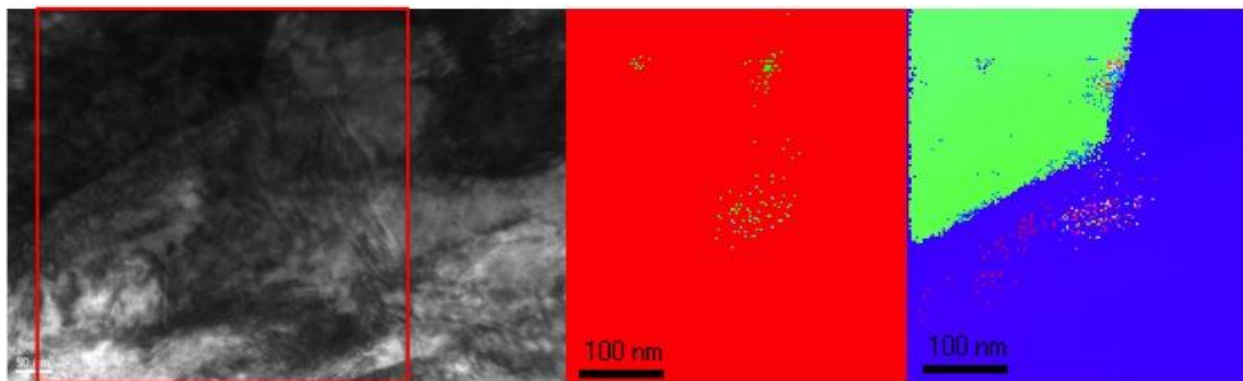
Figure 7: Bright field TEM image (on left) showing the approximate area (red box) from which the phase map (center) and orientation map (right) were generated using Nanomegas.
