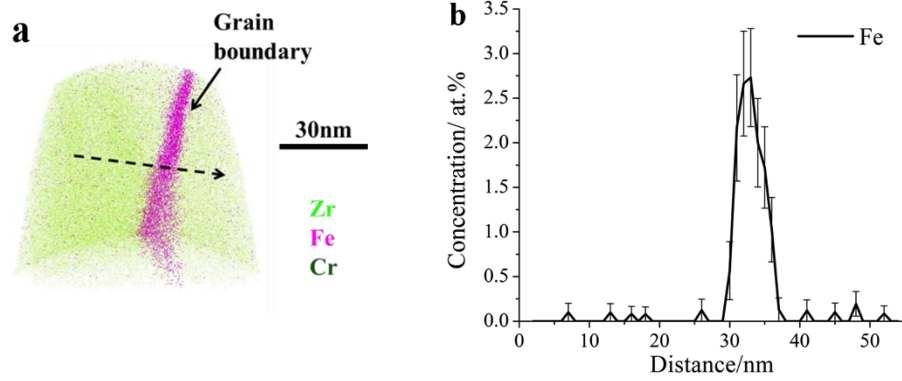
Figure 6: Bulk Zr-Fe-Cr: (a) APT reconstruction showing the grain boundary with Fe segregation; (b) concentration profile across the grain boundary along the arrow shown in (a).
