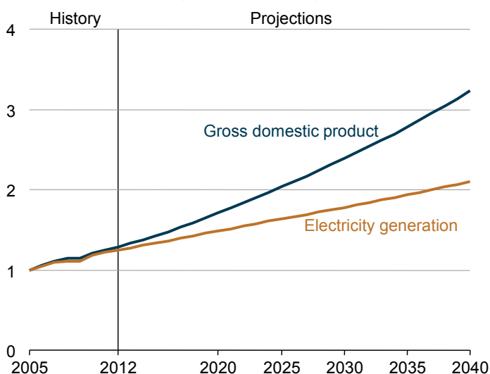
Figure 5-2. Growth in world electricity generation and GDP, 2005–40 (index, 2005 = 1)
