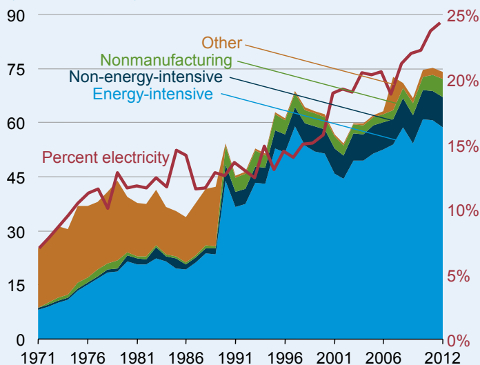
Figure 7-15. Industrial sector electricity demand in the Philippines by industry type, 1971–2012 (terawatthours)
