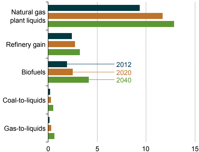
Figure 2-12. World other liquid fuels production by source, 2012, 2020, and 2040 (million barrels per day)
