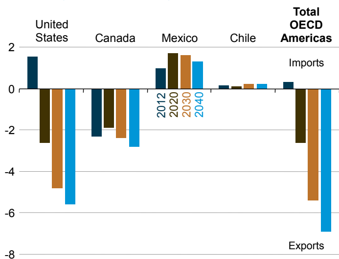
Figure 3-30. OECD Americas net natural gas trade, 2012–40 (trillion cubic feet)
