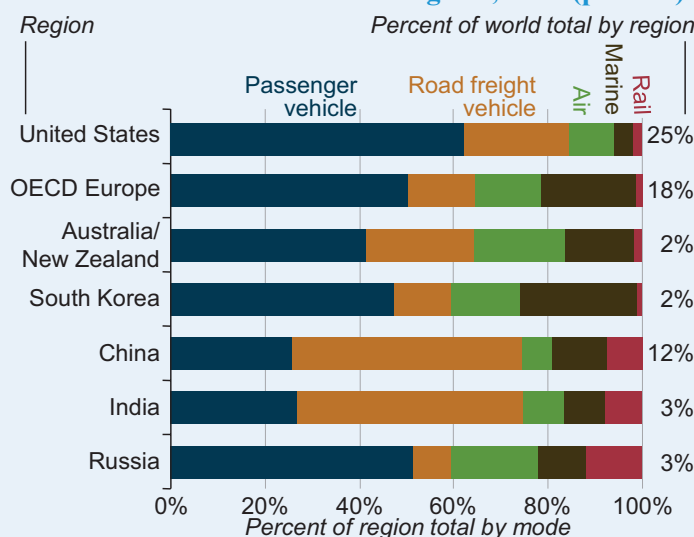
Figure 8-9. Transportation energy consumption by mode in selected countries and regions, 2012 (percent)
