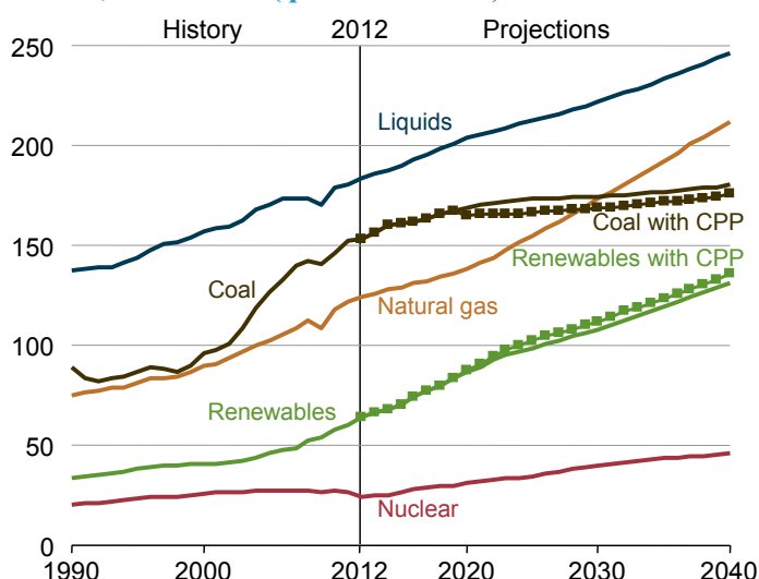
Figure 1-5. World energy consumption by energy source, 1990–2040 (quadrillion Btu)
