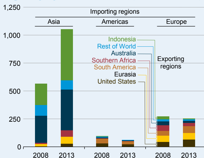
Figure 4-18. World coal trade by importing and exporting regions, 2008 and 2013 (million short tons)
