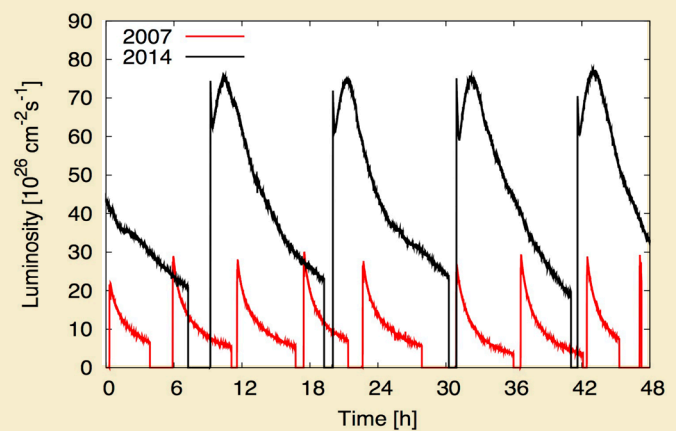
Figure 2: A breakthrough in stochastic beam cooling was able to overcome the internal heating process of the high-energy heavy-ion beams of the Brookhaven RHIC and reduce the beam width up to fivefold. With the brighter beams, the collision frequency or luminosity was vastly increased.
