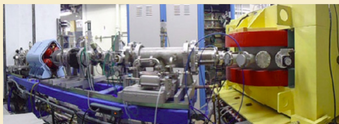
Figure 1: University accelerator facilities such as LENA, the Laboratory for Experimental Nuclear Astrophysics at the Triangle Universities Nuclear Laboratory (TUNL), provide stable, neutron and gamma beams that are critical for measurements of astrophysical reactions that involve stable nuclei and govern the evolution of stars.
