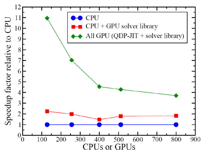
Figure 7.2: The strong reduction of time-to-solution as a result of software development is shown as the speedup gained as compared to the computing time with CPUs or GPUs only as the number of units increases. Shown are speedup factors only utilizing a solver library, and also including the QDP-JIT compilation framework on GPUs. [Image credit: B. Joo].
