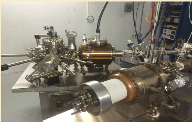
Figure 1: Over 20 years of R&D have dramatically increased the performance of polarized electron sources. Foreground: early-generation source. Back: recent load-lock, ultra-high vacuum source using super-lattice GaAs/GaAsP photocathodes. Such sources can deliver a record 4 mA, 90% polarized electron current.
