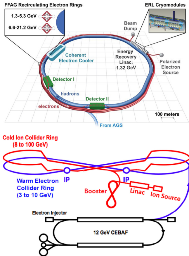
Figure 7.1: Top: The schematic of eRHIC at BNL, which would require construction of an electron beam facility (red) to collide with the RHIC blue beam at up to three interaction points. Bottom: The schematic layout of MEIC at JLab includes the 12-GeV CEBAF and would require construction of an ion linac, an ion collider ring (red), and an electron collider ring (blue) for collisions at two interaction points.
