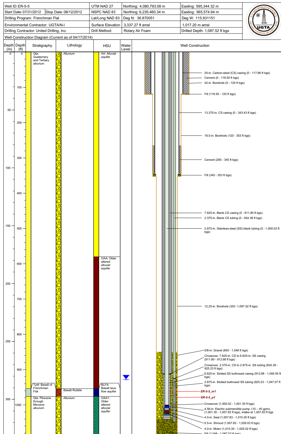
Figure C-4 Well ER-5-5 Construction Diagram
