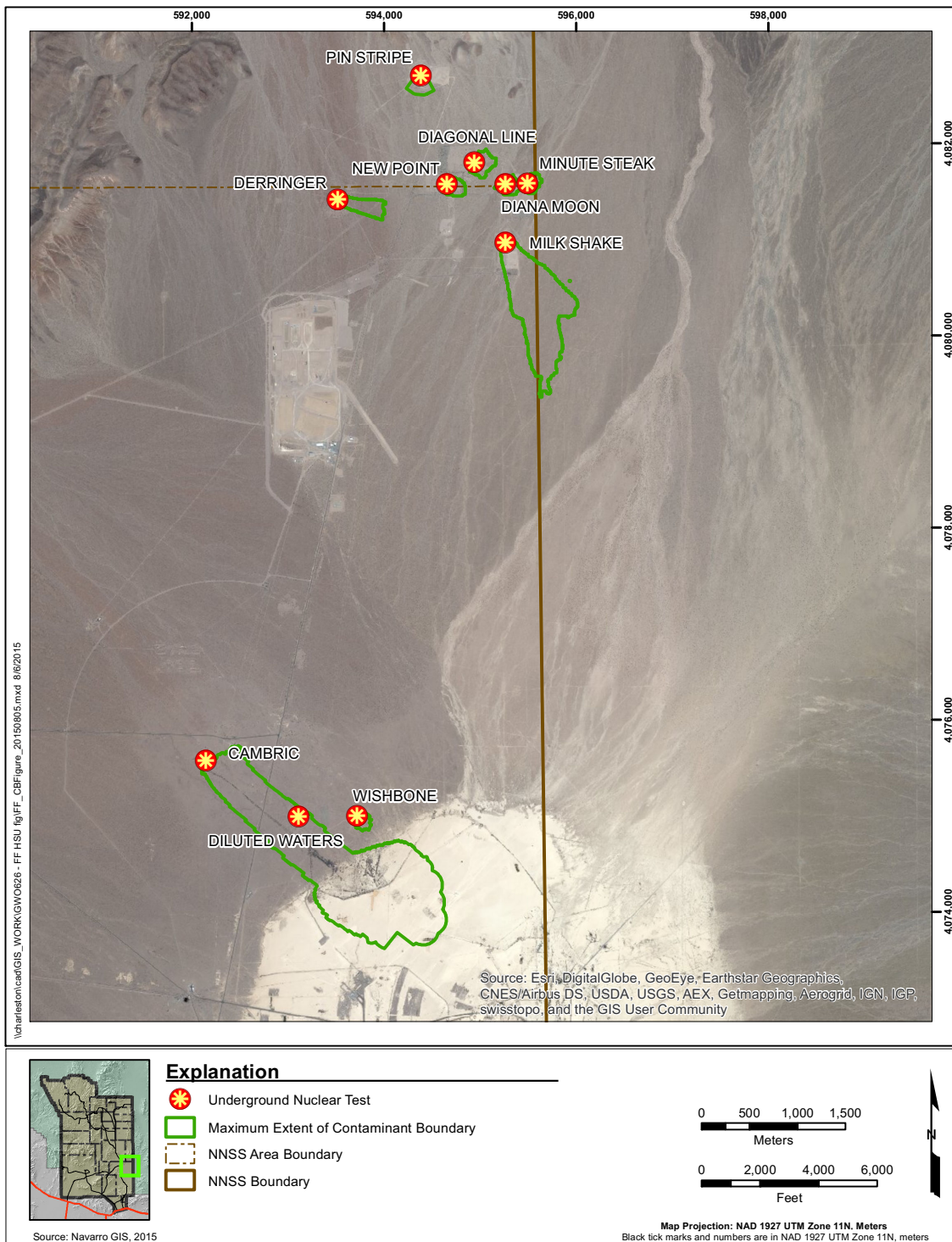
Figure 3-1 Frenchman Flat Contaminant Boundaries
