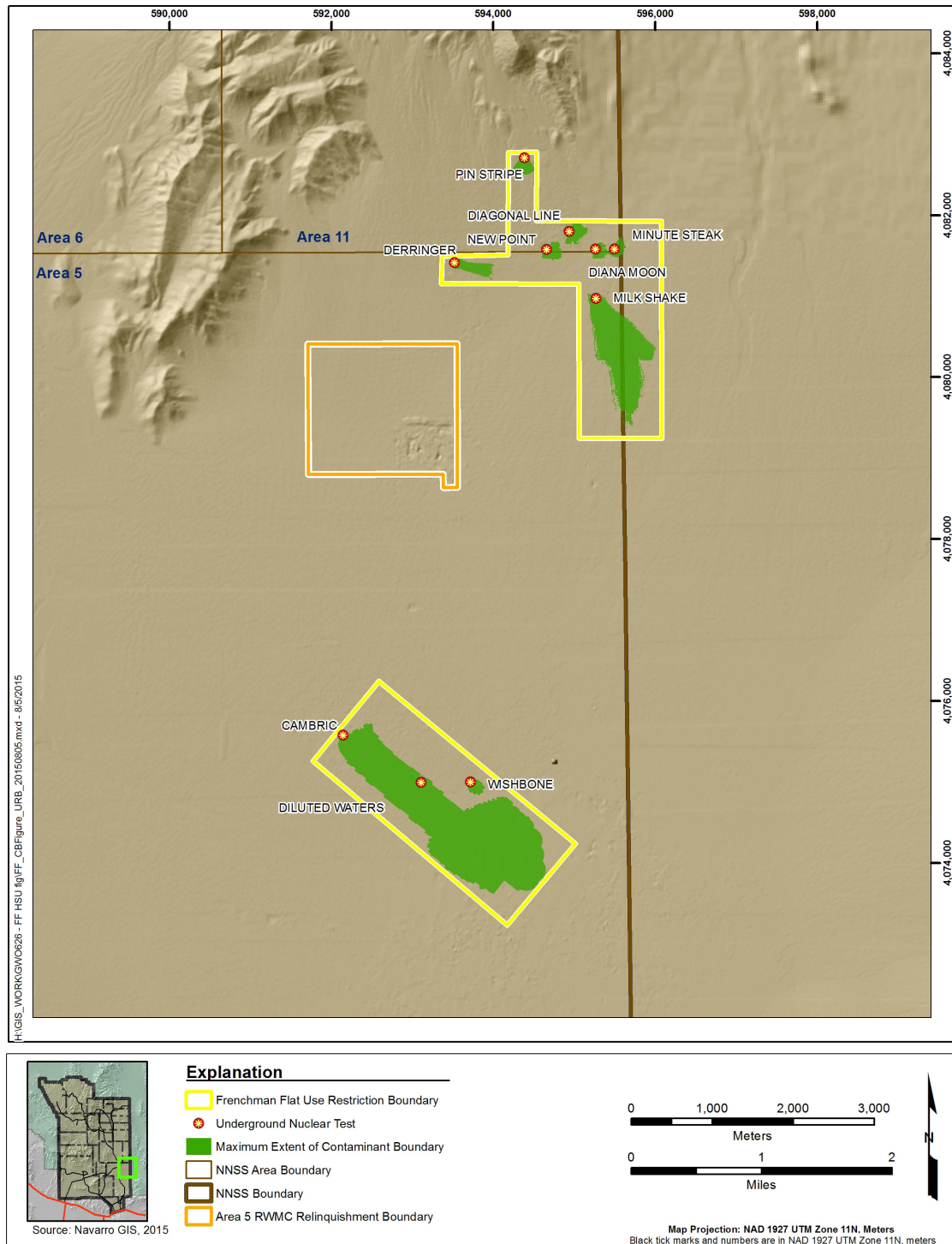
Figure 3-2 Frenchman Flat CAU 98 Groundwater UR Boundaries
