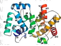
Structure of RVFV (Smith, PNAS , 2010)
