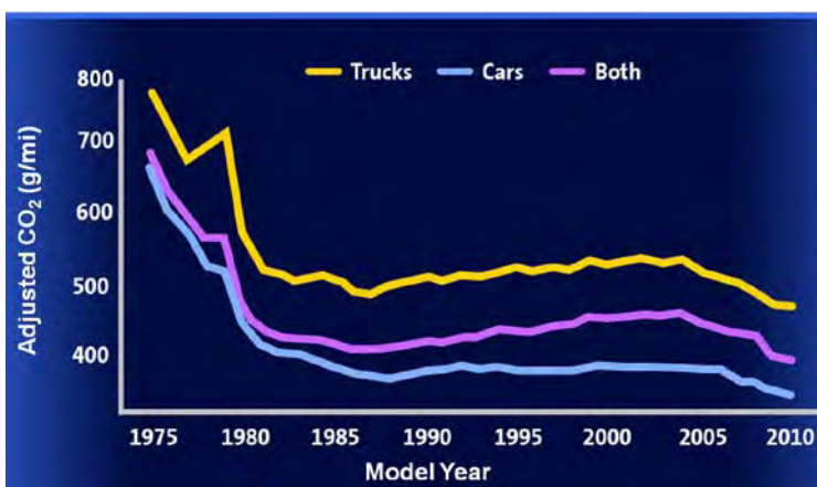
Figure 1. Reduction in the CO 2 output of cars and trucks in the US per mile traveled showing a dramatic decrease over the last 35 years and recent acceleration of progress toward even lower emissions. (Figure courtesy of GM. Data from "Light-Duty Automotive Technology, Carbon Dioxide Emissions, and Fuel Economy Trends: 1975 Through 2010," EPA-420-R-10-023, November 2010)
