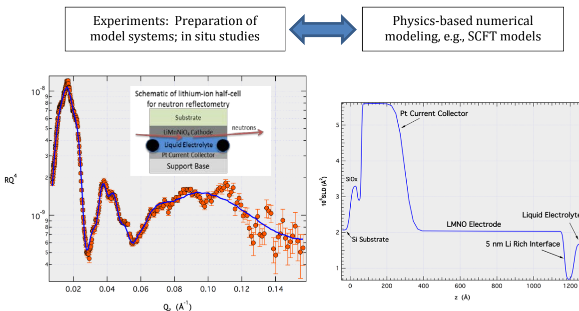
Figure 2. Complementary relationships between reflectivity measurements and computational experiments.
