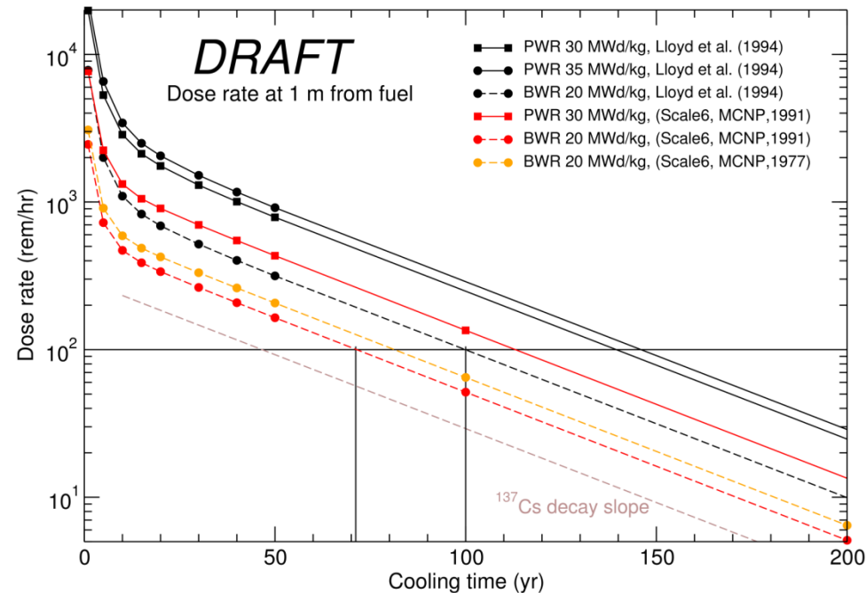
FY2010 Results - Dose Rates for PWR/BWR Low Burn-up Fuels
