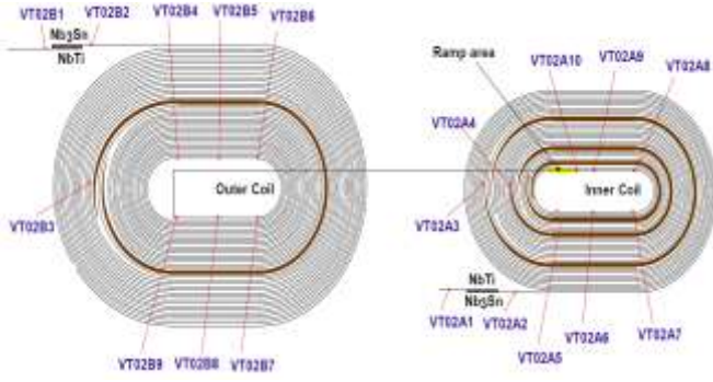
Fig. 6. Voltage tap position in inner and outer layers of the 11 T demonstrator dipole coil.
