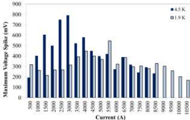
Fig. 11. The maximum spike voltage at a different current intervals.
