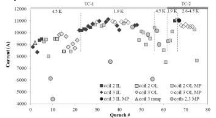
Fig. 7. Quench history and origin in TC1 and TC2.
