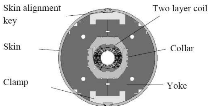
Fig. 1. Cross-sections of the cold mass.
