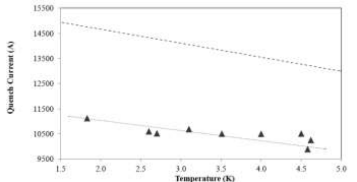
Fig. 9. Temperature dependence of magnet quench current ( dl/dt=50 A/s). The top dashed line represents the dependence of magnet SSL vs. temperature.
