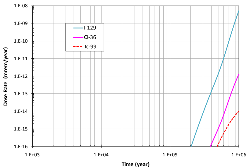
Figure 3. Estimated mean annual dose to a hypothetical receptor located above a borehole repository, base case material properties for the host rock and seal system.
