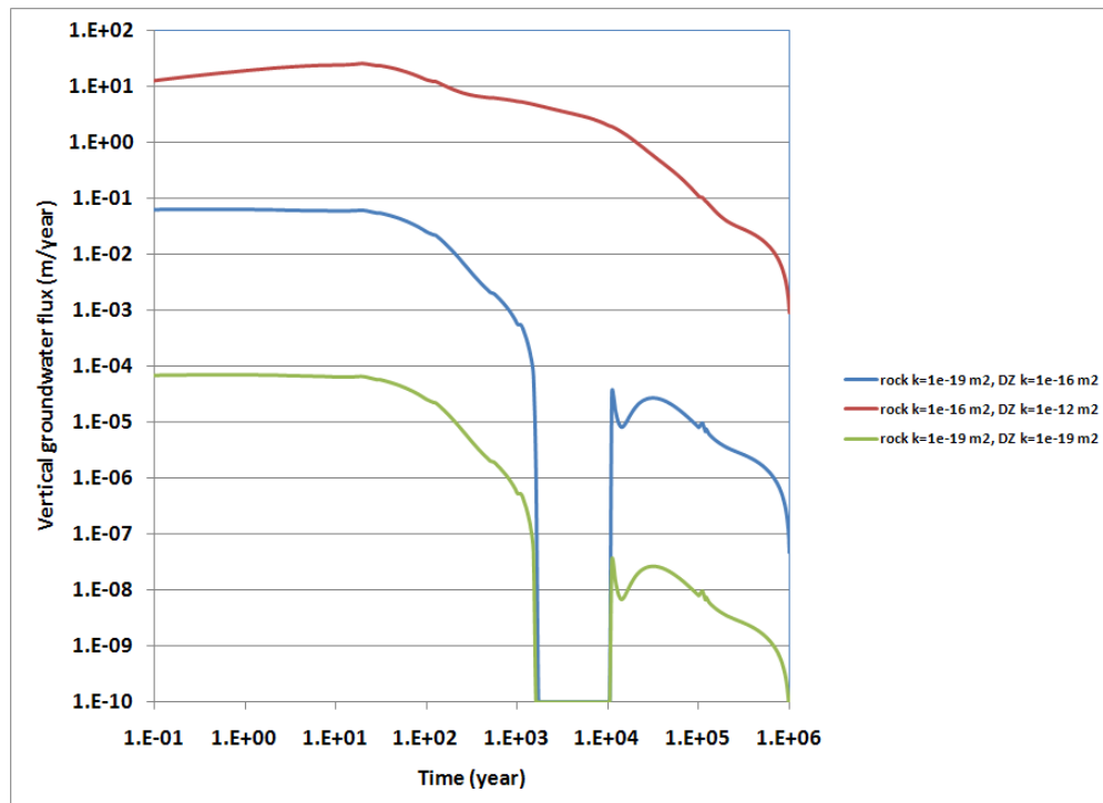
Figure 2. Upward groundwater flux (borehole center, 3000 m depth) versus time. Note that flow is downward for the base case and the lower-permeability seal case between approximately 1000 and 10,000 years (Ref. 16, Figure 3.4-3).
