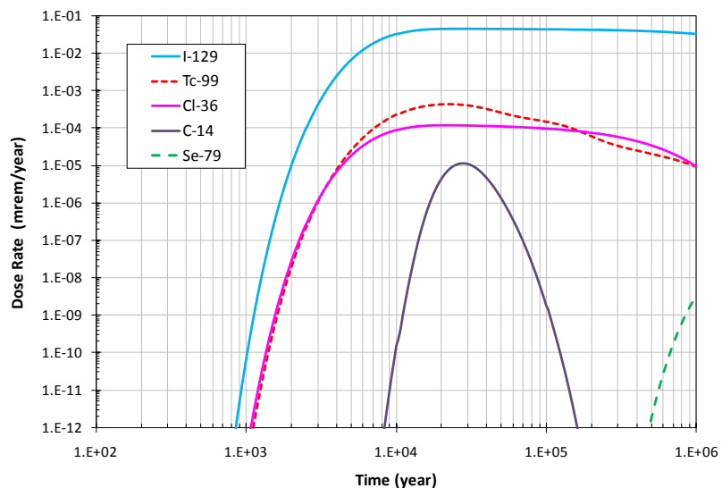
Figure 4. Estimated mean annual dose to a hypothetical receptor located above a borehole repository, fully degraded material properties for the host rock and seal system (seal permeability equivalent to fine sand).
