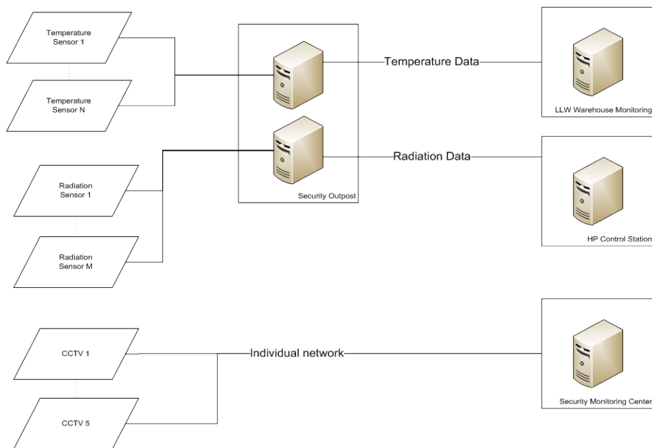
Figure 4: Current design of data flows for the Chinshan Independent Spent Nuclear Fuel Storage Installation
