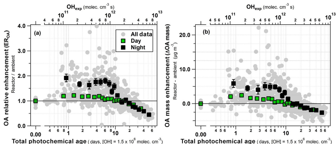
Figure 4. (a) Relative OA enhancement ( \text{ER}_{\text{OA}} = reactor OA / ambient OA) vs. estimated reactor photochemical age for the sampling period. (b) Absolute OA mass concentration enhancement ( \Delta\text{OA mass} = reactor OA – ambient OA) vs. photochemical age. The data have been averaged into 6 % quantiles for day and night measurements, with vertical error bars indicating standard errors.
