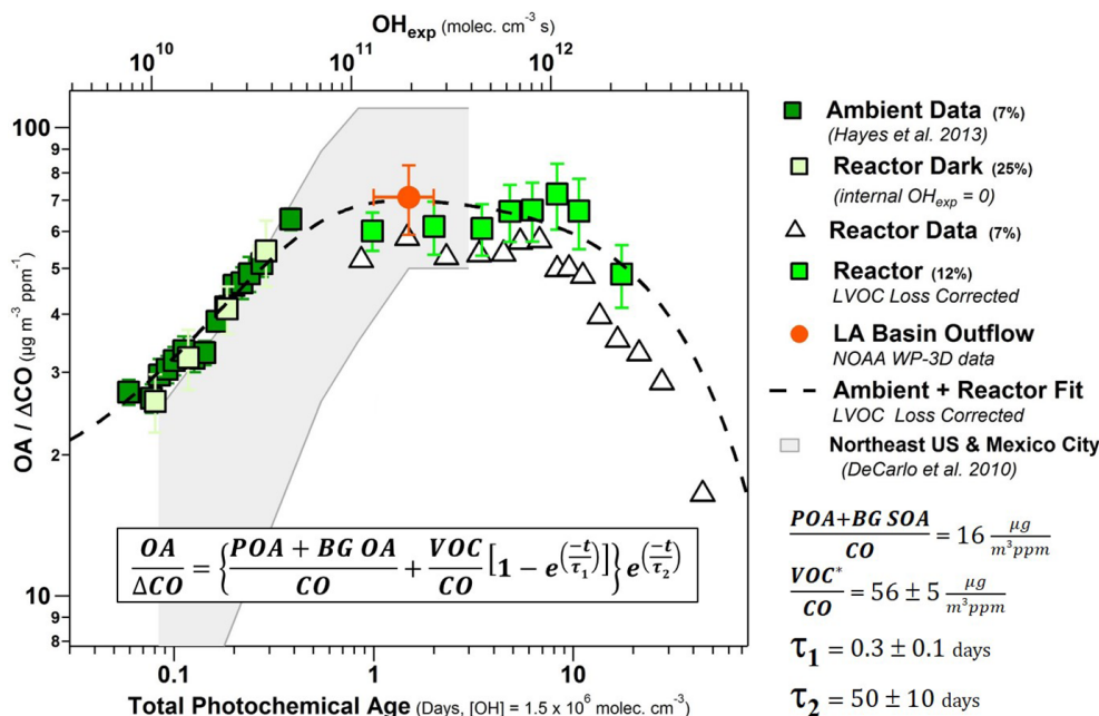
Figure 9. Ratio of OA to excess carbon monoxide (above background levels) vs. total photochemical age in days (at OH = 1.5 \times 10^6 \text{ molec. cm}^{-3} ) for ambient and reactor data, with vertical error bars indicating standard errors. Also shown in the value for LA Basin outflow from aircraft measurements from the NOAA WP-3D during CalNex (Bahreini et al., 2012b). See Hayes et al. (2013) for a discussion of the determination of CO background levels. Averages for quantiles of ambient (7 %), reactor (7 %), reactor dark (25 %, internal OH_{exp} = 0 ), and reactor vapor loss-corrected (12 %) data are shown. A fit to reactor data is also shown, including background (BG) SOA and primary organic aerosol (POA; see text for details). Results from field studies in the northeastern USA and Mexico City are shown in the background (DeCarlo et al., 2010). Note that the LVOC loss correction can only be applied when reactor output OA is larger than ambient OA, which reduces the number of data points.
