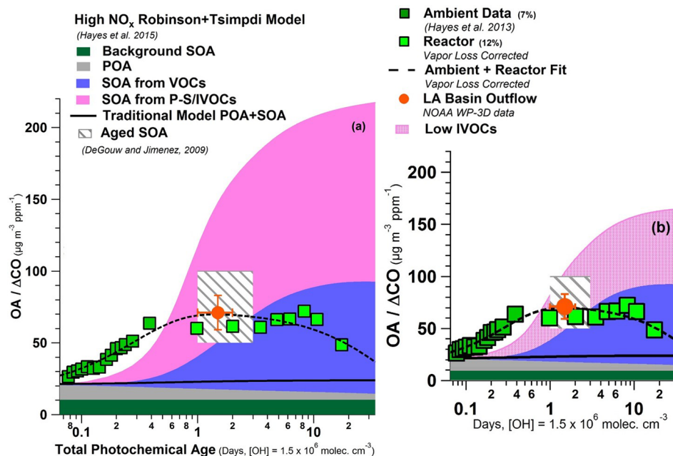
Figure 11. Comparison of reactor data with model results for evolution of \text{OA} / \Delta\text{CO} vs. total photochemical age in days (at \text{OH} = 1.5 \times 10^6 \text{ molec. cm}^{-3} ) with (a) traditional SOA formation model, high \text{NO}_x Robinson + Tsimpdi model from Hayes et al. (2015). Also shown is the summary of urban aged ratios from de Gouw and Jimenez (2009). (b) High \text{NO}_x Robinson + Tsimpdi model from Hayes et al. (2015) run with one-half IVOCs per the results of Zhao et al. (2014). ( \text{POA} + \text{BGSOA} ) / \Delta\text{CO} is 21 \mu\text{g m}^{-3} \text{ ppm}^{-1} , which somewhat is higher than the value of 16 \mu\text{g m}^{-3} \text{ ppm}^{-1} previously reported by Hayes et al. (2013).
