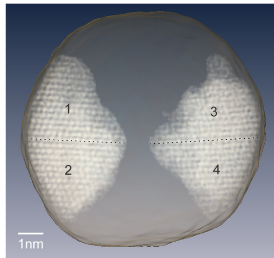
Fig. 1. Identification of four major grains inside Au nanoparticle in 3-D [Scott 2012].
