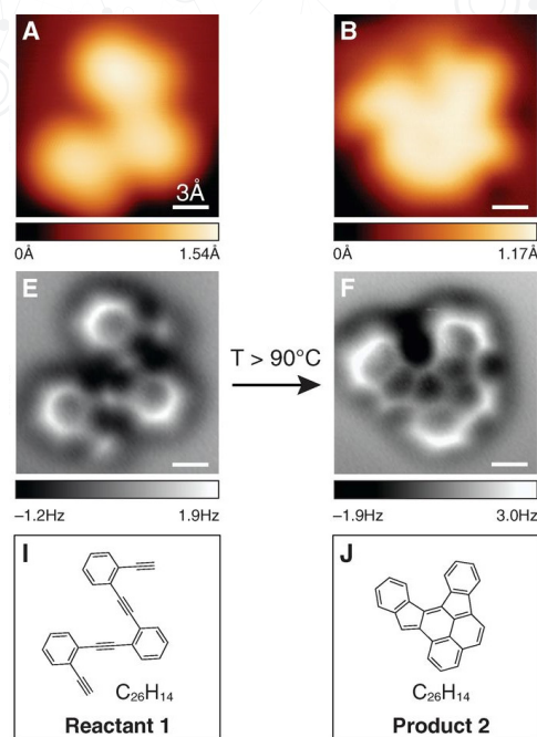
Fig. 5. Non-contact atomic force microscopy images (center) of a molecule before and after reaction show dramatic improvement over images from a scanning tunneling microscope (top) and closely resemble the classic molecular structure diagrams (bottom) [de Oteyza 2013].
