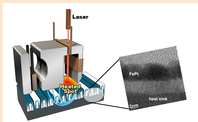
Fig. 3. Schematic illustration of the envisioned next generation magnetic data storage devices where laser heating will assist reversal of the magnetic bit magnetization. An ultrafast local probe of the lattice can ideally determine the currently unknown energy transfer between FePt and heat sink layers. Figure courtesy of Gerardo Bertero.
