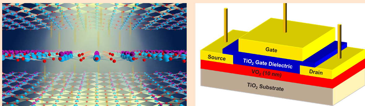
Fig. 7. Schematic illustration of light-induced superconductivity in high T_c cuprates via ultrafast melting of stripe order (left). Ultimately the ultrafast electric field control of emergent behavior such as metallicity could lead to novel oxide electronics applications (right). Figures courtesy of Andrea Cavalleri and Stuart Parkin.
