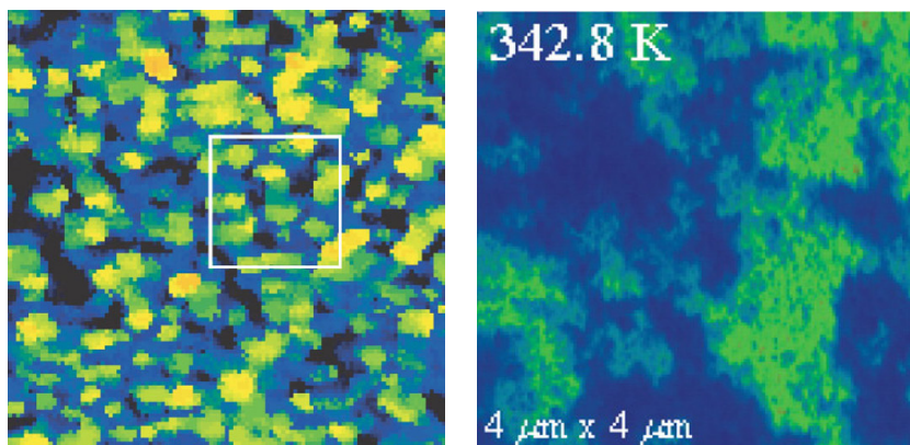
Fig. 2. STM images of the superconducting gap (left, from [Lang 2002]) and metallic/insulating regions (right, from [Qazilbash 2007]). The left panel shows a 50 nm x 50 nm field of view. These images demonstrate the intrinsic electronic nanostructure of such materials.
