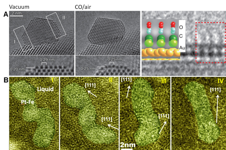
Fig. 8. (A) Gas environmental TEM studies of Au nanoparticle (NP) catalysts supported on \text{CeO}_2 . The inter-atomic distance of Au NPs in 1 Torr CO is increased in contrast to that in UHV. High magnification image of Au NPs with adsorbed CO matches the simulated image. [Yoshida 2012] (B) Real time imaging of Pt-Fe NP growth and shape evolution in a liquid solution of \text{Pt}(\text{acac})_2 , \text{Fe}(\text{acac})_2 dissolved in oleylamine and pentadecane by liquid cell TEM. Surfactant ligands on the surface of Pt-Fe NP play an important role in nanoparticle interaction and shape evolution. [Liao 2012]
