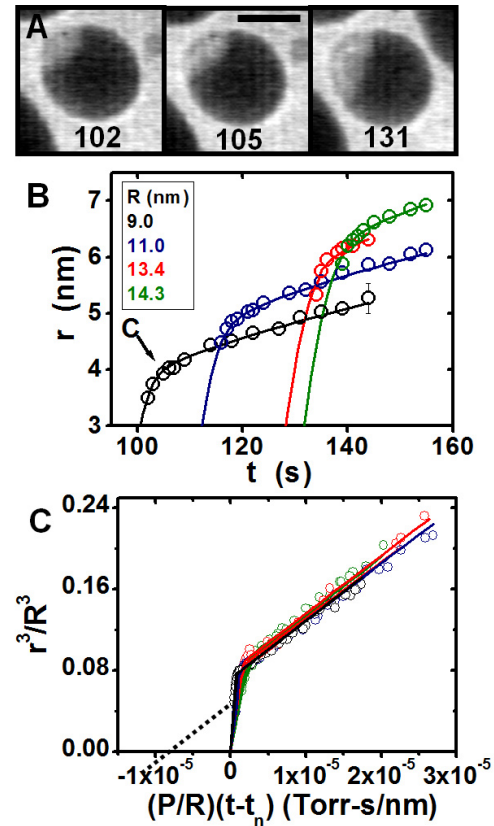
Fig. 9. ((A) Images of a growing Si nucleus (bright region) in a nanoscale eutectic droplet of AuSi (on SiN) during exposure to disilane. Disilane cracks on the surface, releasing Si into the droplet. When the Si super-saturation rises sufficiently, Si nucleates at the droplet periphery. Times in sec, 525°C, 4 \times 10^{-6} torr, scale bar 10 nm. (B) Linear dimension r of several Si nuclei versus time t for droplets of different initial radius R (indicated in the box) during the same growth experiment. (C) Plots of r^3/R^3 versus (P/R)(t - t_n) for all nuclei analyzed at 525°C and four different nominal pressures: 0.35 (black), 0.8 (blue), 1.5 (red), and 4.0 \times 10^{-6} (green) torr disilane. t_n is the nucleation time. The jump size can be related to the super-saturation at t_n . [Kim 2008]
