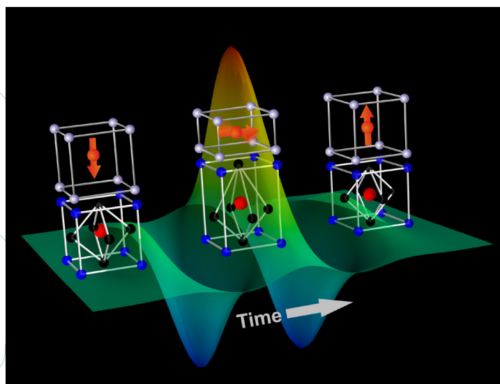
Fig. 12. A single-cycle THz pulse coupling to ferroelectric polarization in a multiferroic material. The availability of such pump pulses will provide unprecedented opportunities for understanding and the ultrafast control of materials properties for use in the next-generation functional devices.
