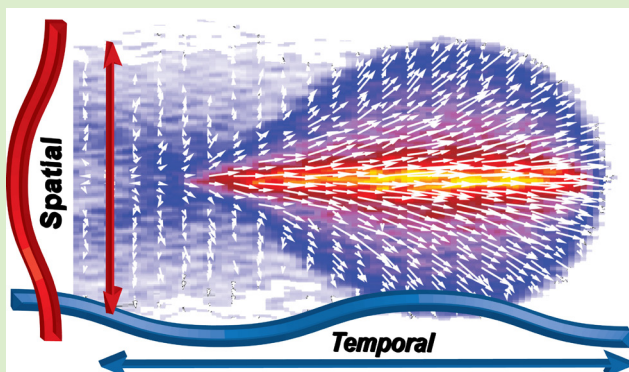
Fig. 11. Free-space propagating ultrashort electron pulse exhibiting collective and stochastic space charge dynamics. The electron pulse manipulation using longitudinal and transverse lenses to reconstruct electron six-dimensional phase space allows optimization of combined temporal, spatial, and spectroscopic resolution.
