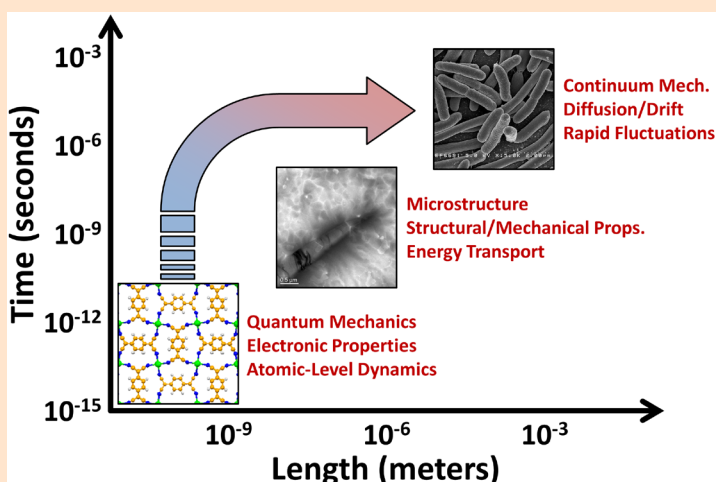
Fig. 4. Length-time plot illustrating multiscale dynamics and how quantum-level properties emerge at the larger mesoscale described by continuum mechanics.
