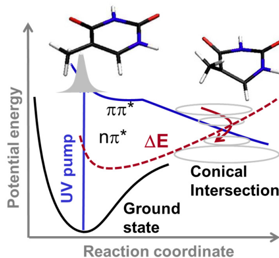
Fig. 6. The relaxation of photo-excited thymine is a key process in DNA photo protection. Simulations indicate that the molecule relaxes through a conical intersection. The structures are from [Hudock 2007]. Figure courtesy of Markus Guehr.
