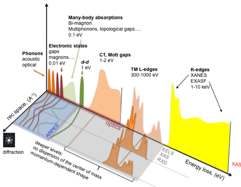
Fig. 10. Taxonomy of excitations and their observability by pump-probe techniques. The different excitations are mapped on to the 3D space formed by momentum (reciprocal space), energy, and spectroscopic intensity. Courtesy of F. Carbone.
