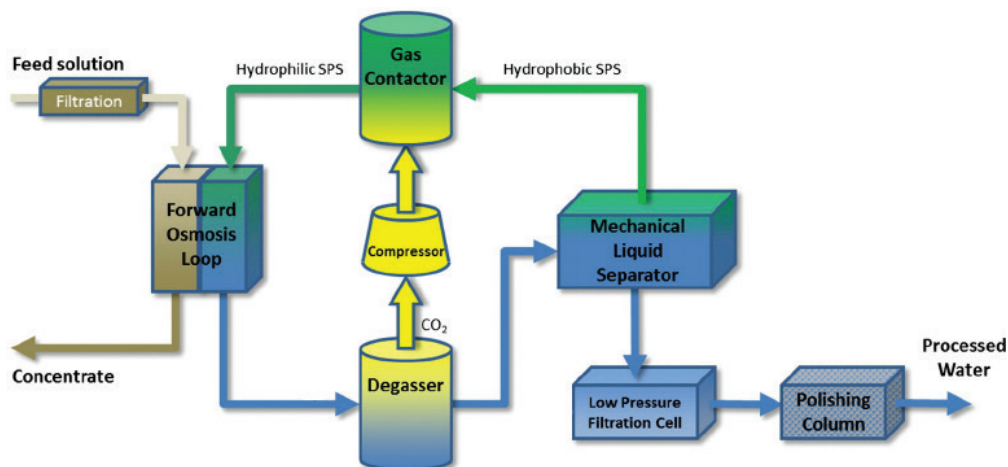
The proposed Switchable Polarity Solvent - Forward Osmosis system being developed by Idaho National Laboratory
