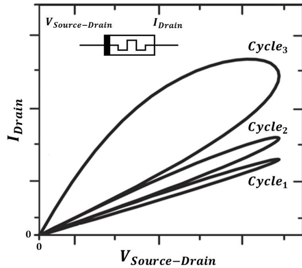
Figure 8. I-V characteristic of a memristor, the basis of a possible neuromorphic architecture.
