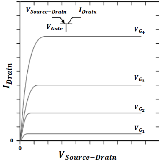
Figure 7. I-V characteristic of a transistor, the basis of von Neumann architecture.
