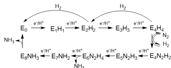
Figure 9. Lowe and Thorneley (LT) kinetic scheme for nitrogenase catalysis. Accumulation of electrons and protons on FeMo-co is represented by En states where n represents the total number of electrons and protons accumulated. Reaction scheme from R. Thorneley and D. Lowe, in Molybdenum Enzymes (Ed. T. G. Spiro), p. 221, Wiley, NY (1985).
