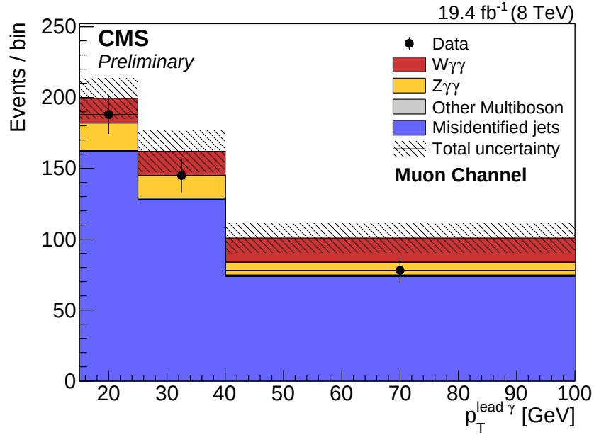
Figure 3: Validation of the data-driven estimates of misidentified electrons and jets signal-like events that have 15 \text{ GeV} < p_T^{\text{sublead}} < 25 \text{ GeV} in the muon channel. The misidentified jet and misidentified electron contributions are estimated using data-driven techniques. The W^\pm\gamma\gamma , Z\gamma\gamma and other multiboson contributions are given by simulation. The hatched area represents the combined uncertainty from all background estimates.
