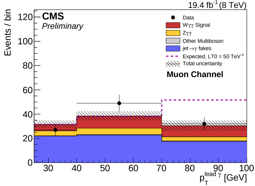
Figure 2: Observed data with predicted background contributions, expected SM W^\pm\gamma\gamma signal and the contribution from an aQGC where the f_{T,0} parameter is 50 \text{TeV}^{-4} (dashed line).
