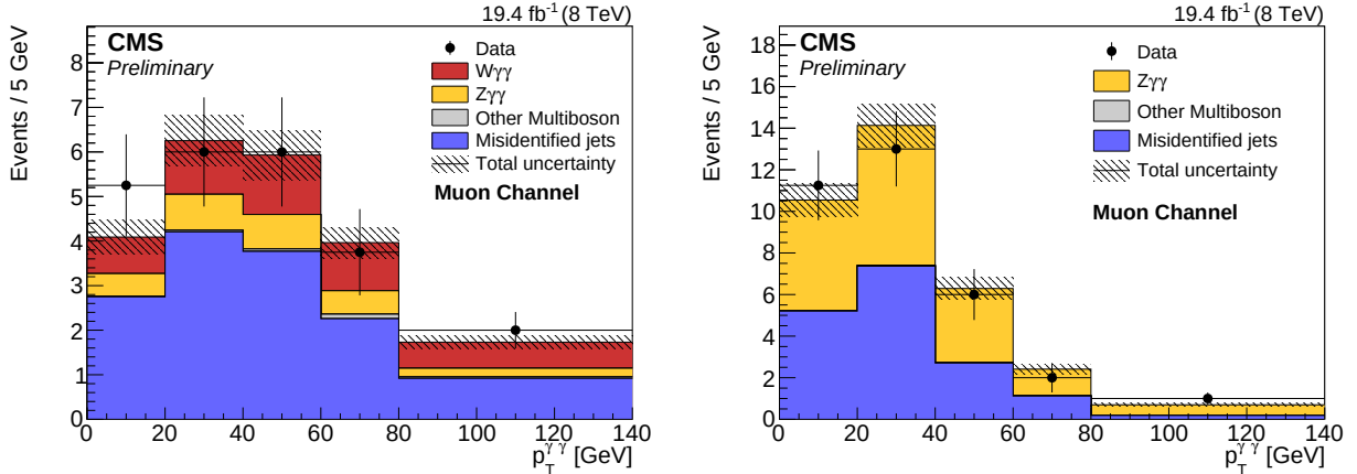
Figure 1: The p_T of the diphoton system in the muon channel for the W^\pm\gamma\gamma analysis (left) and Z\gamma\gamma analysis (right). The jet misidentification background contribution is determined from data-driven methods. In each plot, the other multiboson contributions are estimated using simulation and are normalized to their production cross section. The hatched band represents the total uncertainty of all background sources, combined in quadrature. The last bin includes all events having p_T^{\gamma\gamma} > 80 GeV, but the normalization is to the displayed bin width.
