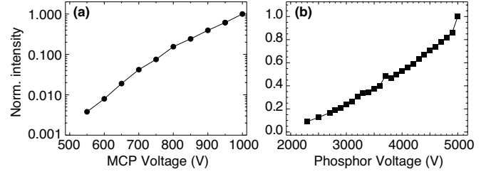
FIG. 4. Normalized detector sensitivity as a function of voltage (a) on MCP, at fixed V_{ph} = 4500 V; (b) on phosphor, at fixed V_{MCP} = 950 V.
