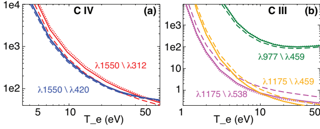
FIG. 1. Electron temperature sensitive line intensity ratios of \Delta n = 0 to \Delta n = 1 transitions of carbon ions. (a) C IV, lines represent three typical divertor densities as follows: 4.92 \times 10^{-19} \text{ m}^{-3} (.....); 1.64 \times 10^{-20} \text{ m}^{-3} (—); 4.92 \times 10^{-20} \text{ m}^{-3} (---). (b) C III, lines represent three typical divertor densities as follows: 5 \times 10^{-19} \text{ m}^{-3} (.....); 1 \times 10^{-20} \text{ m}^{-3} (—); 5 \times 10^{-20} \text{ m}^{-3} (---).
