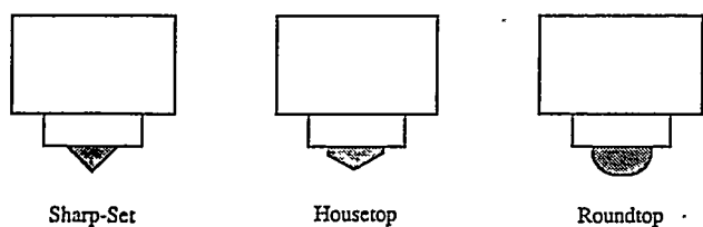
Figure 11 - Profiles of TSP cutters used in single-cutter wear tests. (TSP disk cutter not shown.)
