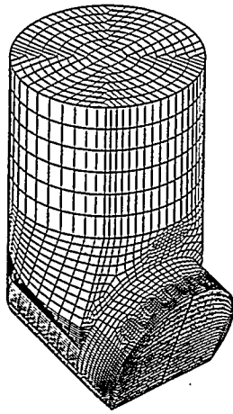
Figure 1 - Typical claw-cutter finite-element mesh.
