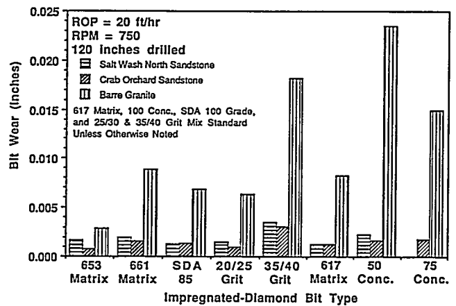
Figure 14 - Measured bit wear for various impregnated-diamond bit designs in three hard, abrasive rock types.
