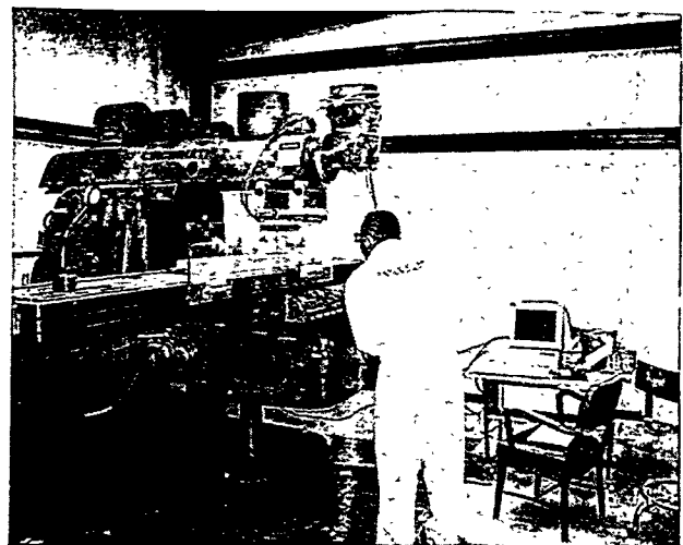
Figure 6 - Horizontal milling machine used to perform instrumented, linear, single-cutter tests for Track-Set bit design.
