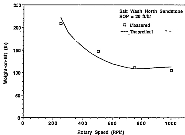
Figure 15 - Comparison of measured drilling performance with that predicted by the model developed for impregnated-diamond drill bits.
