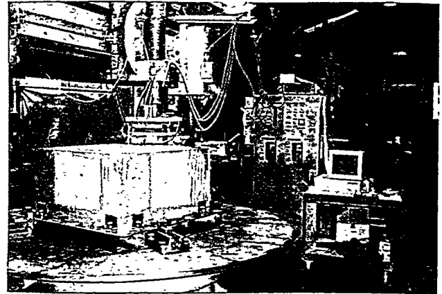
Figure 2 - Vertical lathe set-up used to wear-test single PDC and TSP cutters.
