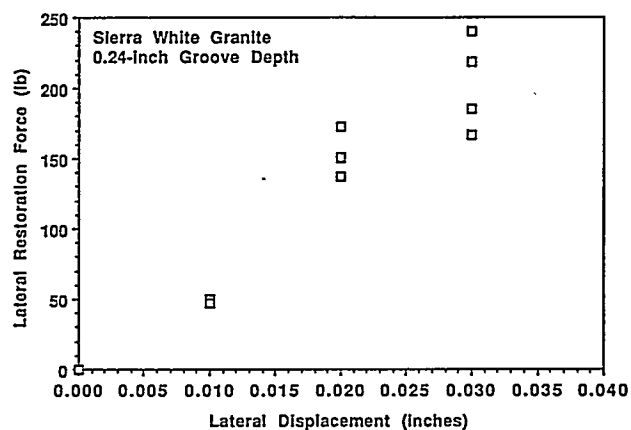
Figure 10 - Measured lateral restoration forces in single-cutter tests in Sierra White Granite.
