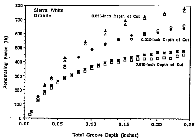
Figure 8 - Measured penetrating forces in single-cutter, engagement-angle tests in Sierra White Granite.
