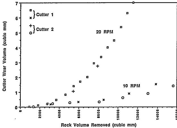
Figure 3 - Conventional PDC cutter wear rates measured on the vertical lathe in Sierra White Granite at two rotary table speeds.
