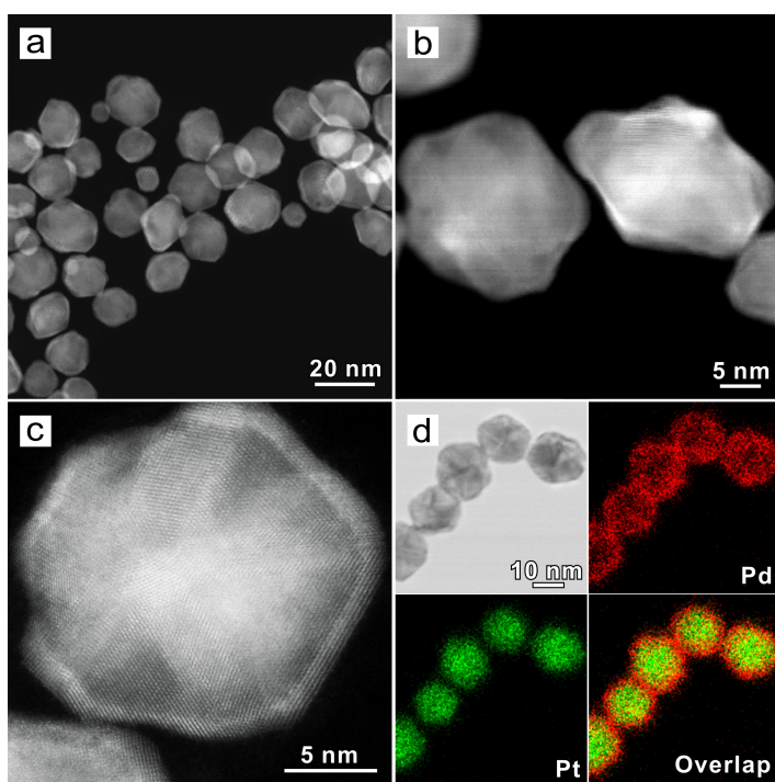
Figure 2. Structural and compositional analyses of the Pd@Pt core-shell concave decahedra with 47.5 wt% Pt. (a) Low- and (b) high-magnification HAADF-STEM images of the decahedra, showing that more Pt was deposited on the vertices and edges of a Pd decahedral seed than the faces. (c) Atomic-resolution HAADF-STEM image of an individual decahedron. (d) HAADF-STEM image of the concave decahedra and the corresponding EDX mapping of elemental Pd and Pt.
