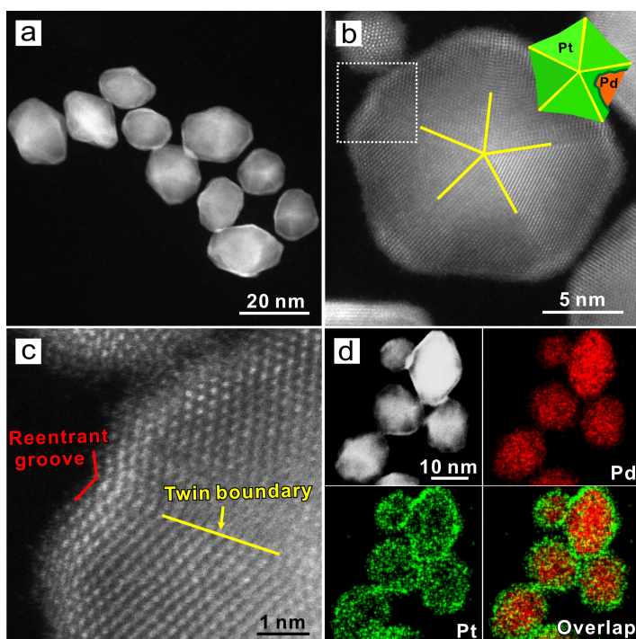
Figure 1. Structural and compositional analyses of the Pd@Pt core-shell concave decahedra with 29.6 wt% Pt. (a) HAADF-STEM image. (b) Atomic-resolution HAADF-STEM image and a model of the decahedron viewed along its 5-fold axis (inset). (c) Atomic-resolution HAADF-STEM image taken from the corner marked by a box in (b), showing a reentrant groove present at the vertex and a twin boundary. (d) HAADF-STEM image of the concave decahedra and the corresponding EDX mapping of elemental Pd and Pt.
