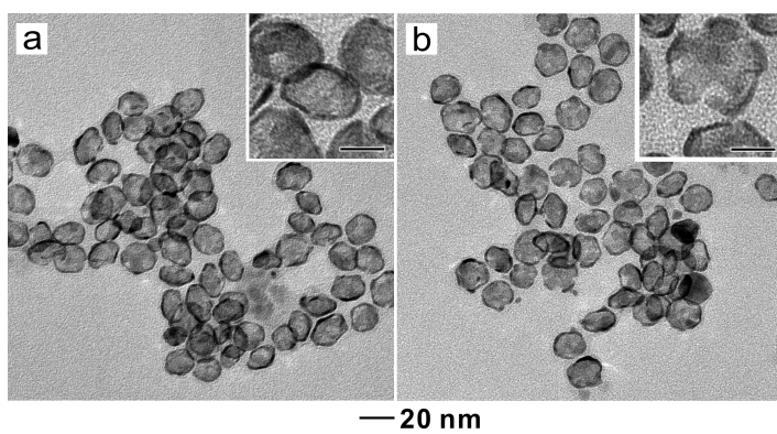
Figure 4. (a) TEM image of the products obtained by etching the Pd@Pt concave decahedra with 47.5 wt% Pt at 90 °C for (a) 2 h and (b) 3 h, respectively. The scale bars in the insets are 10 nm.
