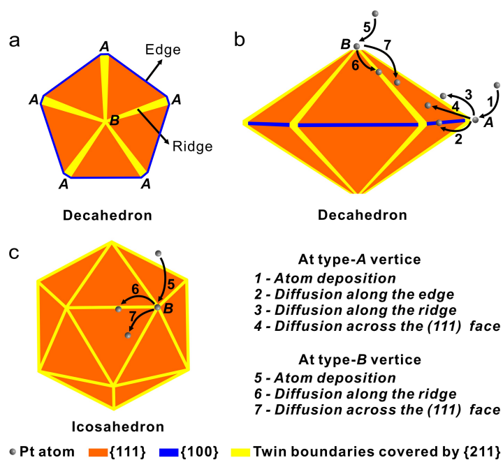
Figure 3. (a) Schematic of a decahedron viewed along its 5-fold axis, showing the type- A and type- B vertices, as well as the ridges and edges. (b,c) Schematic illustrations showing how the Pt atoms are deposited onto Pd decahedral and icosahedral seeds, respectively, and the possible routes for the initially deposited Pt atoms to diffuse across the surface.
