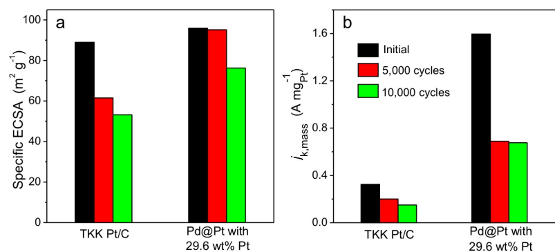
Figure 6. Comparison of the durability for the carbon-supported Pd@Pt concave decahedra with 29.6 wt% Pt and the TKK Pt/C catalyst. The comparison is based on (a) the specific ECSAs and (b) the mass ORR activities at 0.9 V_{\text{RHE}} for the catalysts before and after the accelerated ORR durability tests. The color scheme specified in (b) applies to both panels.
