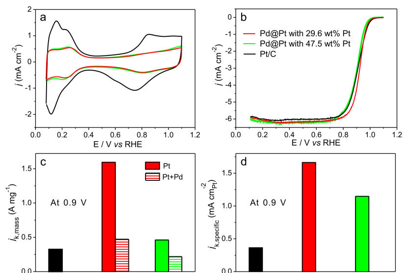
Figure 5. Electrochemical properties of the carbon-supported Pd@Pt concave decahedra with 29.6 wt% and 47.5 wt% Pt, respectively, in comparison with the TKK Pt/C catalyst. (a) CVs of the catalysts in a N_2 -saturated HClO_4 solution at room temperature. (b) Comparison of positive-going ORR polarization curves of the catalysts in an O_2 -saturated HClO_4 solution. (c) Mass and (d) specific ORR activities at 0.9 V_{RHE} , which are given as kinetic current densities ( j_k ) normalized to the mass of Pt (or Pd+Pt) and ECSAs, respectively, of the catalyst. The color scheme specified in (b) applies to all other panels.
