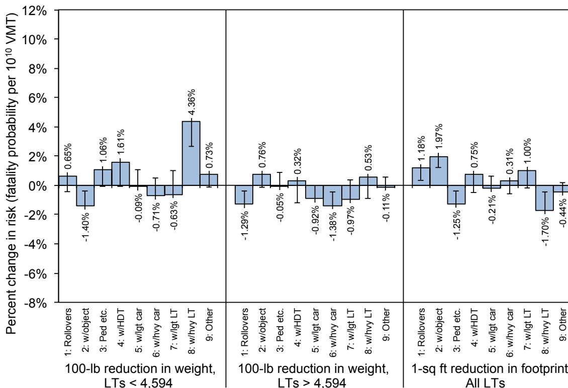
Figure 2.3. Estimated effect of mass or footprint reduction on risk in light trucks, by type of crash
