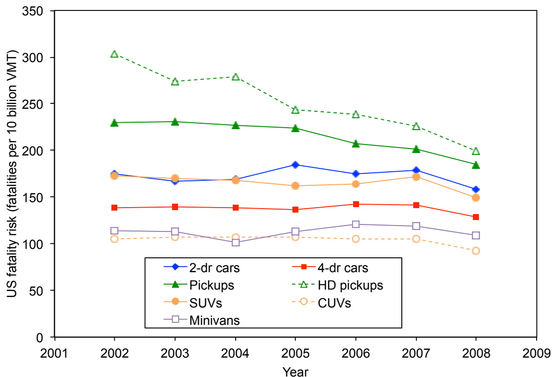
Figure 5.8. US fatality risk per VMT, by vehicle type and calendar year
