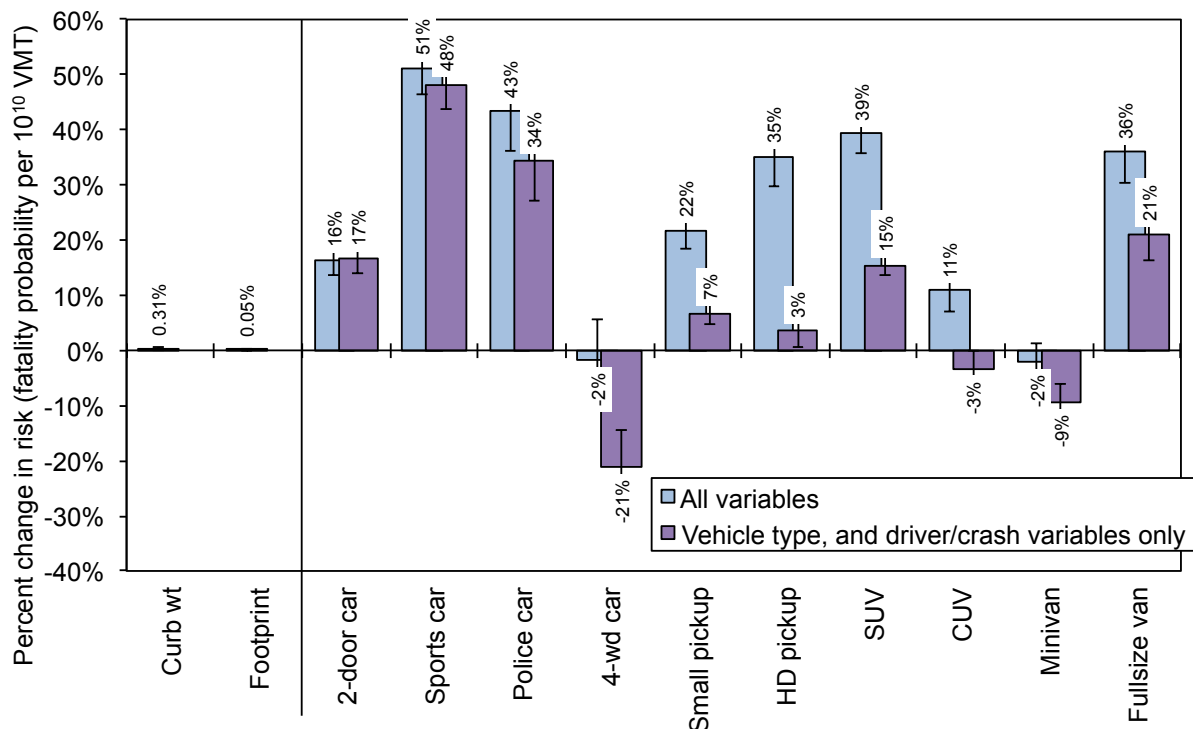
Figure 6.13. Effect of mass and footprint reductions across all vehicle types, and a comparison of fatality risk by vehicle type compared to four-door sedans
