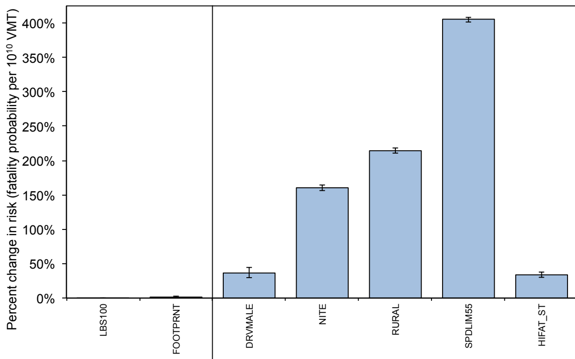
Figure 2.10. Estimated effect of selected control variables on risk, CUVs and minivans
