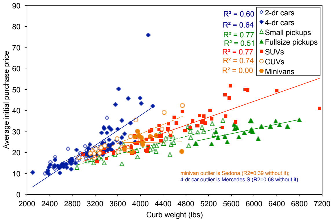
Figure 4.19. Relationship between vehicle mass and initial purchase price, by vehicle model
