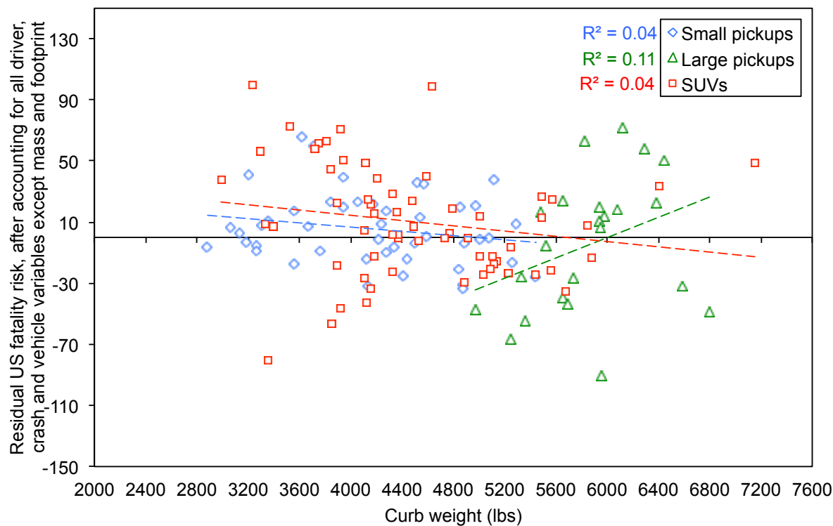
Figure 4.14. Residual US fatality risk per VMT after accounting for all driver, crash, and vehicle variables except mass and footprint vs. curb weight, light truck models
