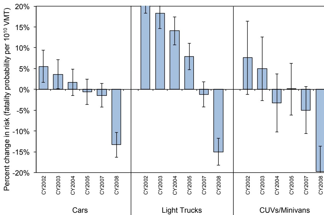
Figure 5.4. Effect of calendar year variables on risk, by vehicle type
