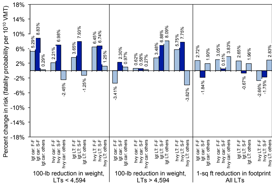
Figure 6.9. Estimated effect of mass reduction on risk to light truck occupants only in two-vehicle crashes, by crash partner vehicle type and crash configuration
