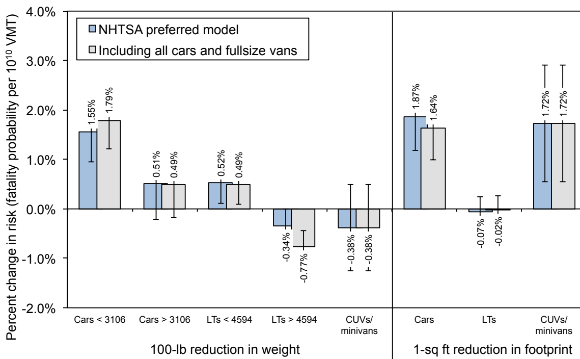
Figure 5.15. Estimated effect of mass and footprint reduction on US fatality risk per VMT, after including sports, police, and all-wheel drive cars, and fullsize passenger and cargo vans, by vehicle type
