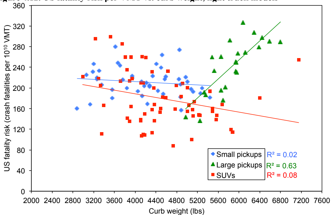
Figure 4.13. Predicted US fatality risk per VMT after accounting for all driver, crash, and vehicle variables except mass and footprint vs. curb weight, light truck models
