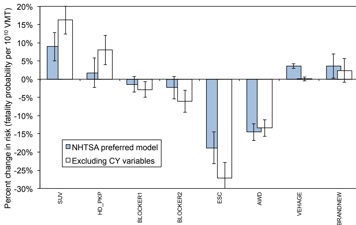
Figure 5.12. Estimated effect of selected control variables on light truck risk, including and excluding calendar year variables
