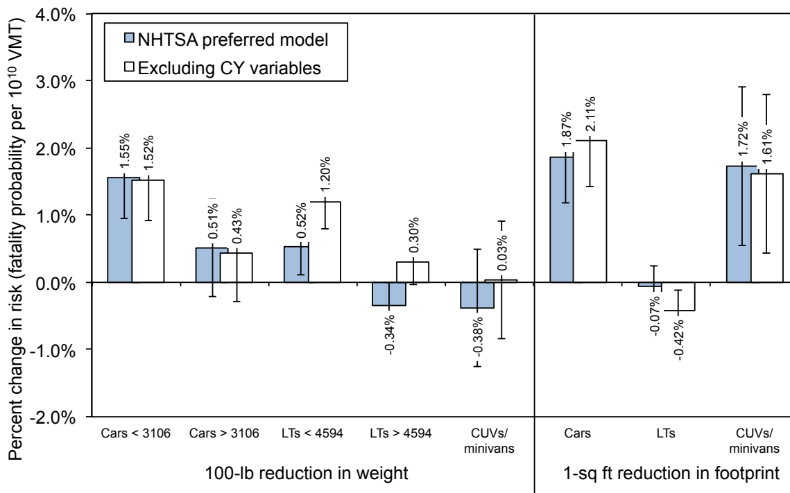
Figure 5.10. Effect of increasing weight or size on risk, including and excluding calendar year variables
