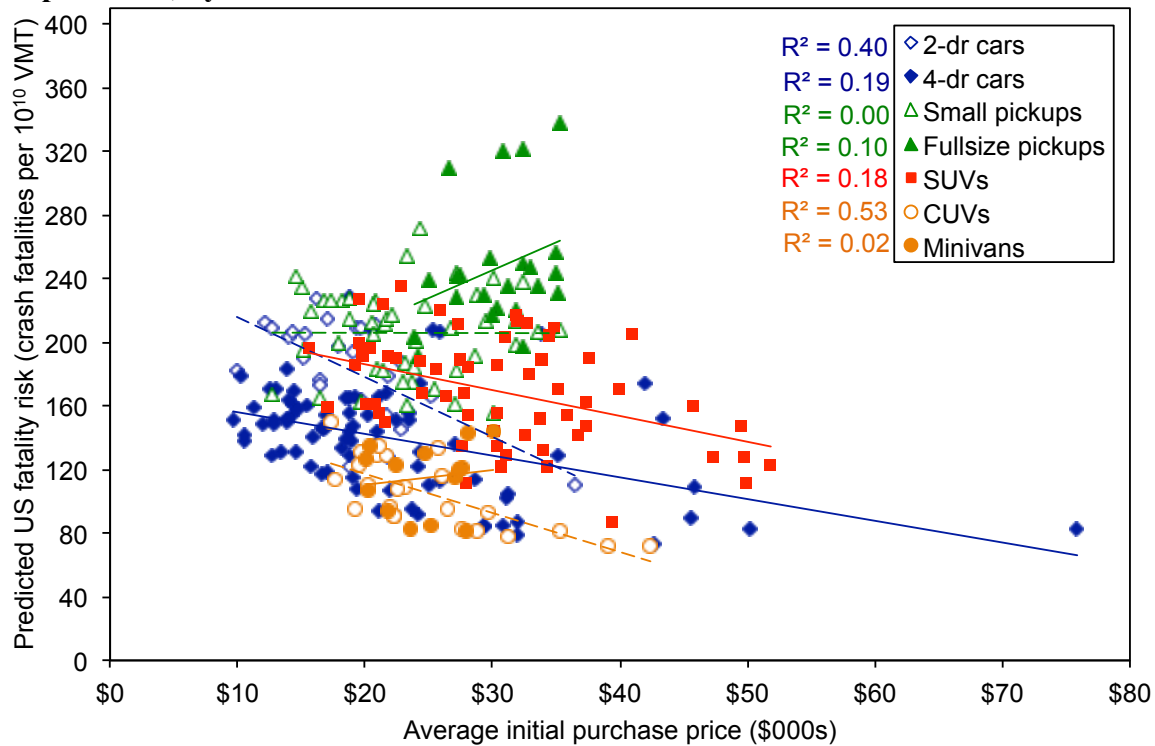
Figure 4.18. Relationship between vehicle initial purchase price and predicted US fatality risk per VMT, by vehicle model
