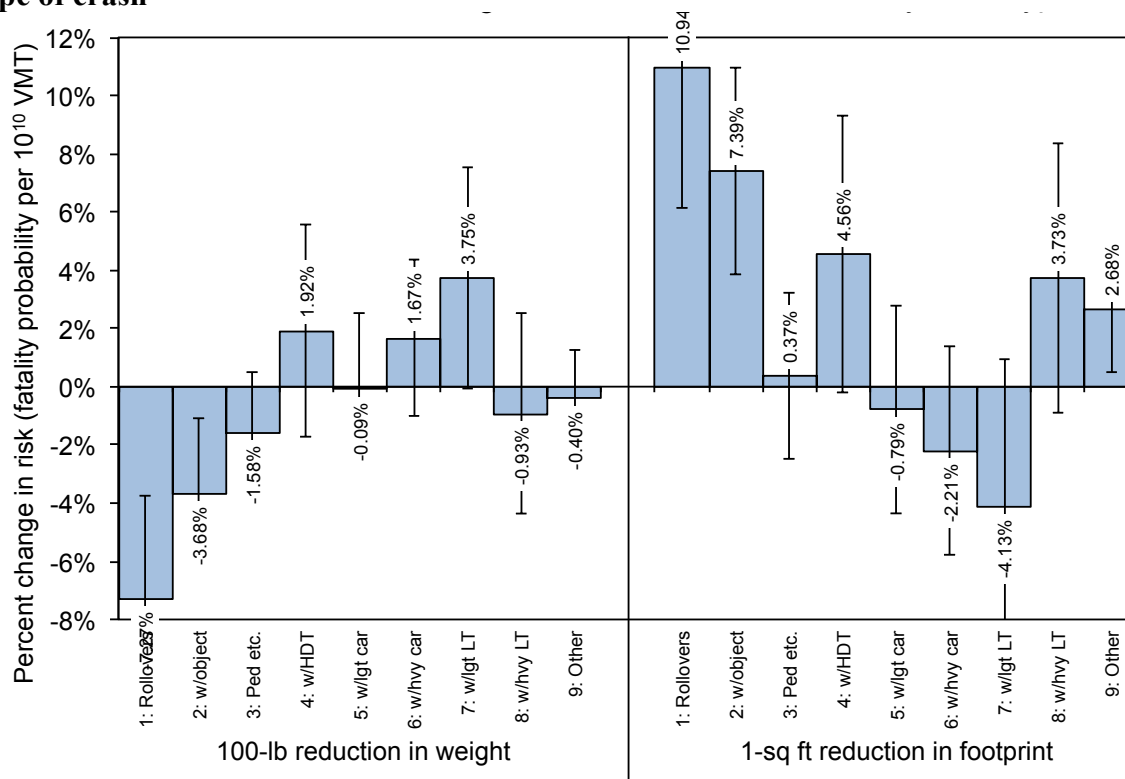
Figure 2.4. Estimated effect of mass or footprint reduction on risk in CUVs/minivans, by type of crash
