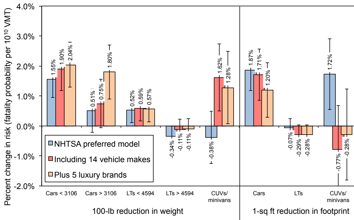
Figure 5.2. Estimated effect of mass or footprint reduction on US fatalities per VMT, after controlling for vehicle manufacturer, by vehicle type
