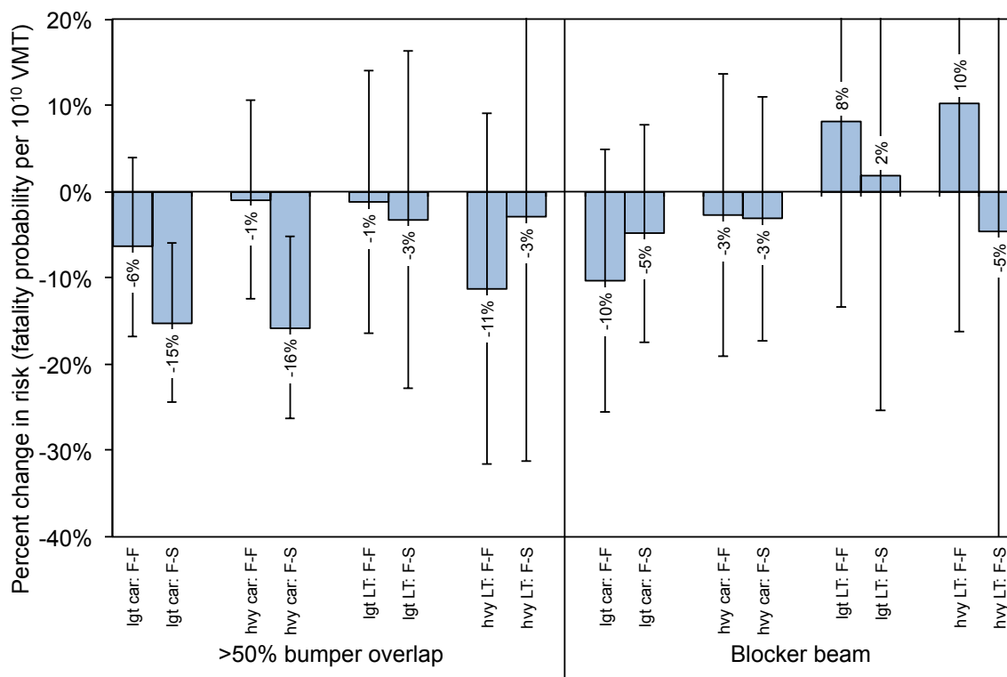
Figure 6.11. Effect of compatibility measures on risk imposed by light trucks on other light-duty vehicles, by crash partner vehicle type and crash configuration
