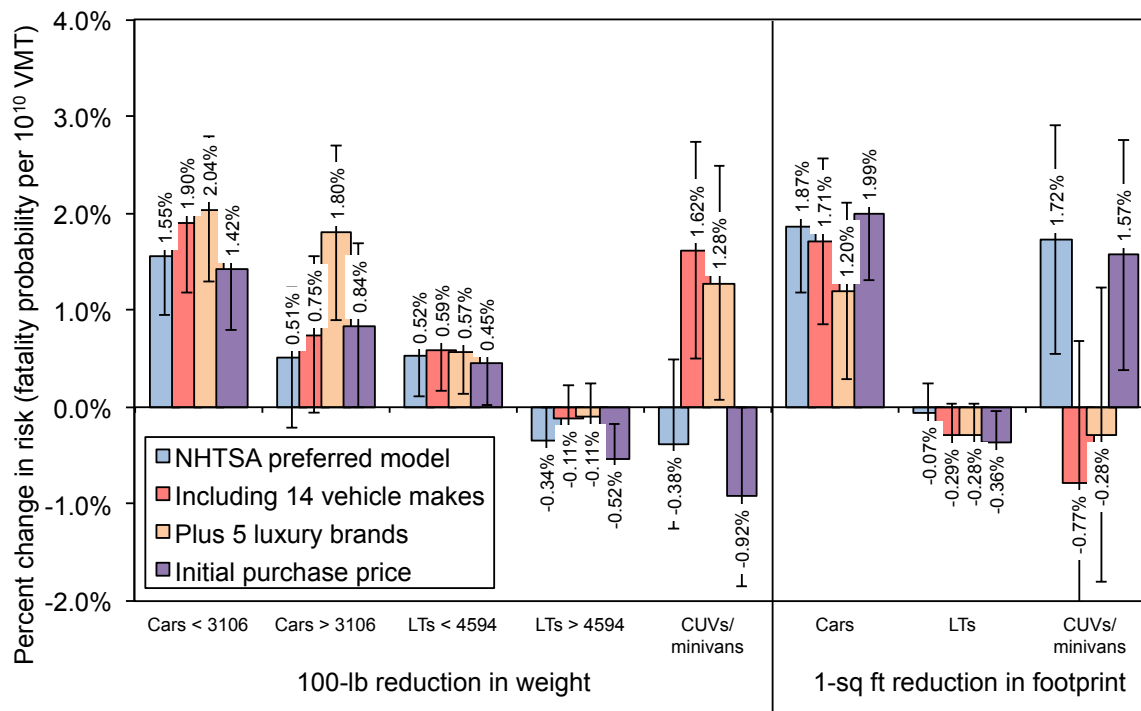
Figure 5.3. Estimated effect of mass or footprint reduction on US fatalities per VMT, after controlling for vehicle manufacturer or for initial vehicle purchase price, by vehicle type
