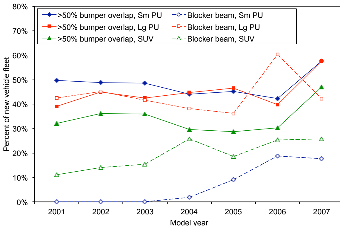
Figure 6.10. Market penetration of compatibility measures in light trucks, by light truck type and model year
