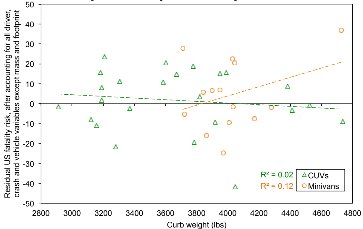
Figure 4.17. Residual US fatality risk per VMT after accounting for all driver, crash and vehicle variables except mass and footprint vs. curb weight, CUV/Minivan models
