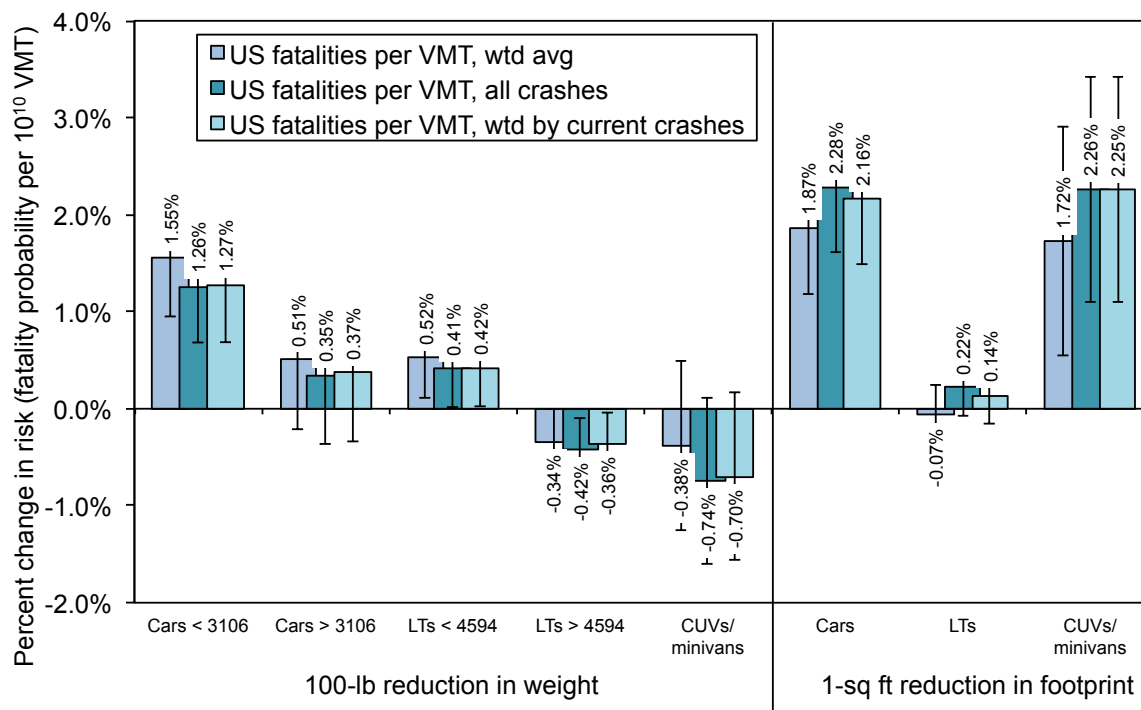
Figure 2.1. Estimated effect of mass or footprint reduction on US fatality risk per VMT, across all crash types and weighted average effect in each type of crash, by vehicle type
