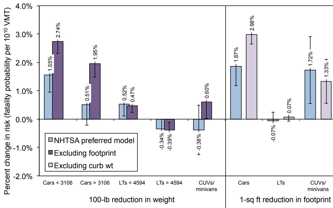
Figure 3.3. Estimated effect of mass or footprint reduction on risk, by vehicle type: mass only, footprint only, and both
