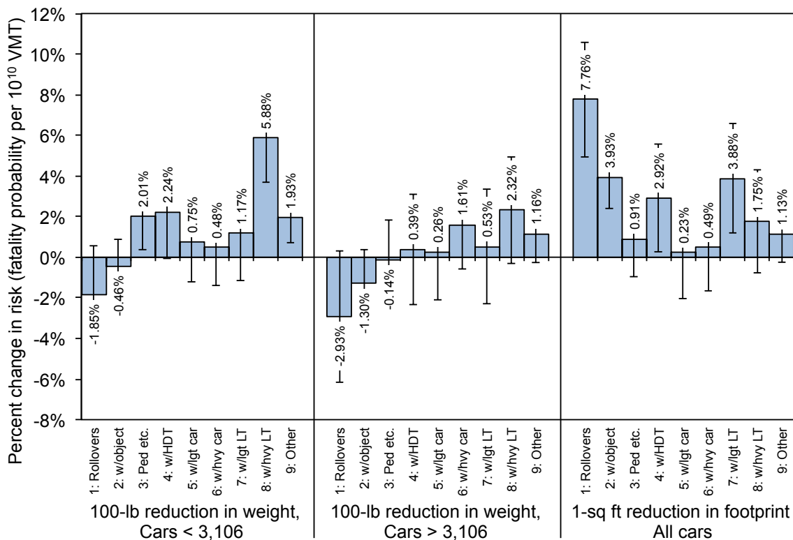
Figure 2.2. Estimated effect of mass or footprint reduction on risk in cars, by type of crash
