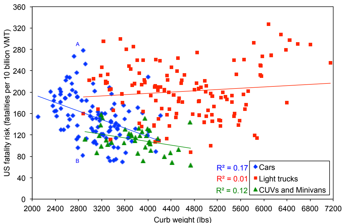
Figure 4.6. US fatality risk per VMT and curb weight, by vehicle model
