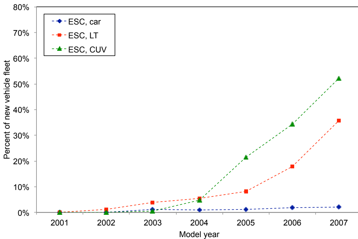
Figure 6.1. Market penetration of ESC, by vehicle type and model year
