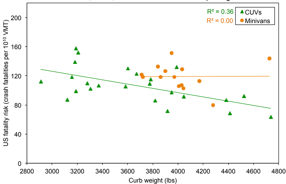
Figure 4.15. US fatality risk per VMT vs. curb weight, CUV/Minivan models
