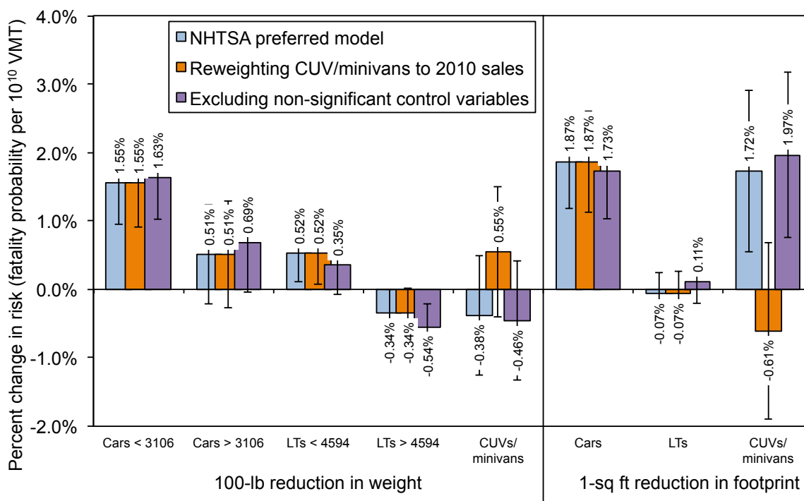
Figure 5.16. Estimated effect of mass and footprint reduction on US fatality risk per VMT, after reweighting CUV/minivan fatalities to 2010 sales and excluding non-significant control variables, by vehicle type
