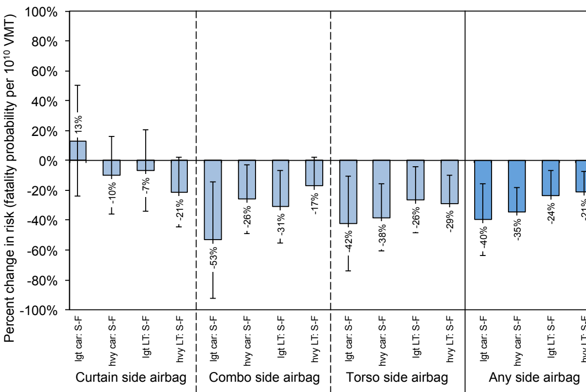
Figure 6.4. Estimated effect of side airbags on risk to car occupants only, when struck in the side by another light-duty vehicle, by crash partner vehicle type
