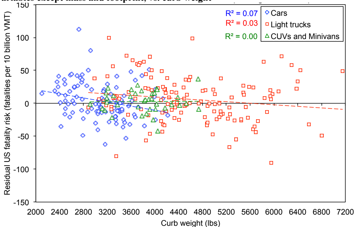
Figure 4.8. Residual US fatality risk after accounting for all driver, crash, and vehicle variables except mass and footprint, vs. curb weight
