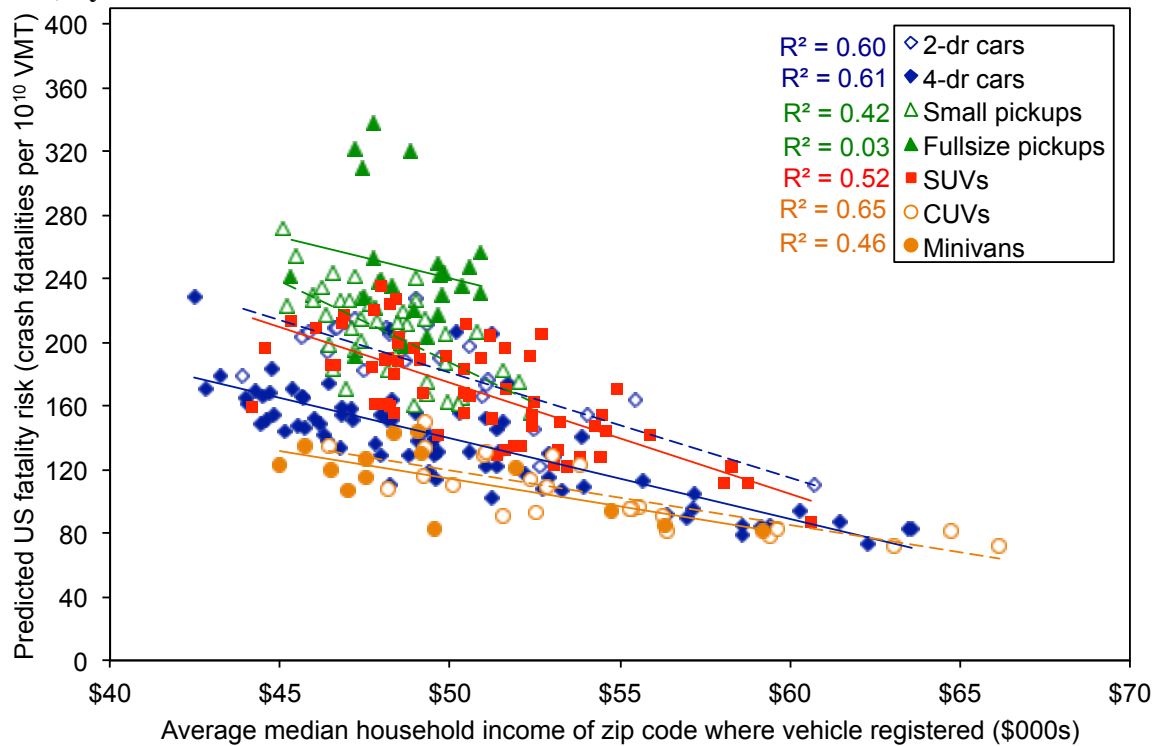
Figure 4.20. Relationship between household income and predicted US fatality risk per VMT, by vehicle model
