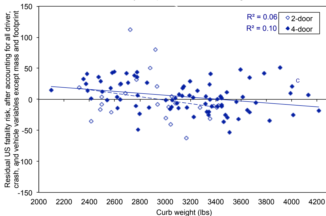
Figure 4.11. Residual US fatality risk per VMT after accounting for all driver, crash, and vehicle variables except mass and footprint vs. curb weight, car models
