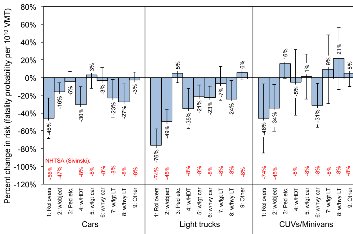
Figure 6.2. Estimated effect of ESC on fatality risk, by vehicle type and crash type
