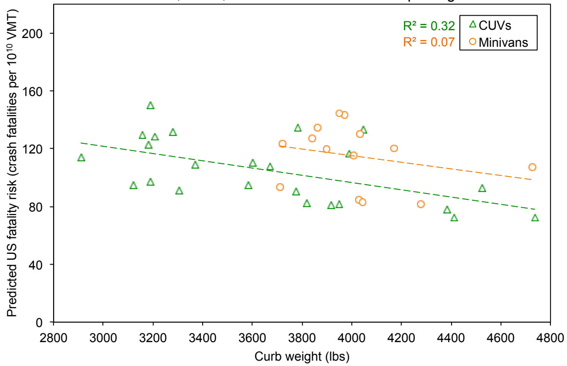
Figure 4.16. Predicted US fatality risk per VMT after accounting for all driver, crash and vehicle variables except mass and footprint vs. curb weight, CUV/Minivan models
