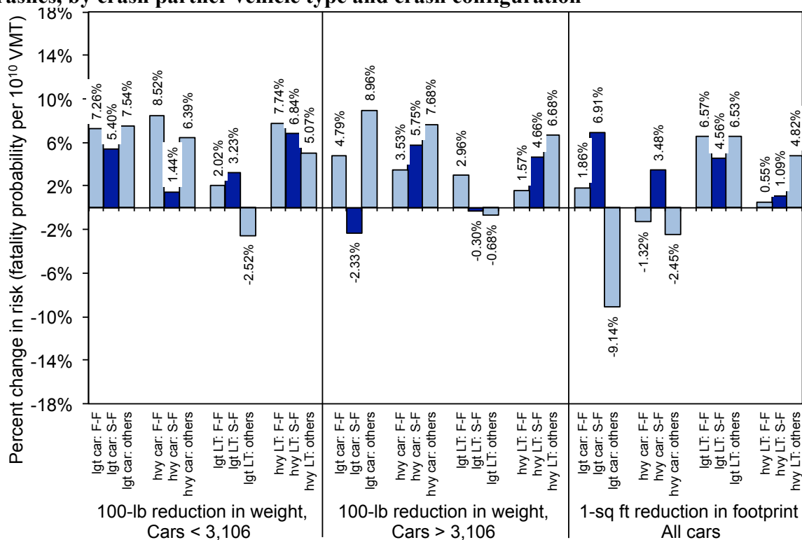
Figure 6.7. Estimated effect of mass reduction on risk to car occupants only in two-vehicle crashes, by crash partner vehicle type and crash configuration
