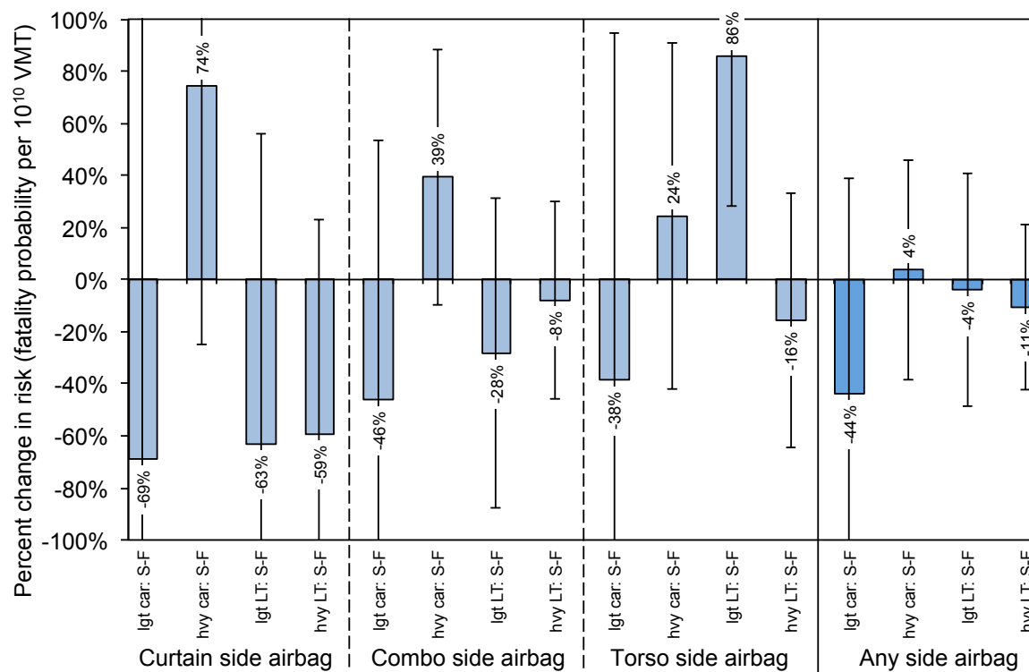
Figure 6.5. Estimated effect of side airbags on risk to CUV/minivan occupants only, when struck in the side by another light-duty vehicle, by crash partner vehicle type
