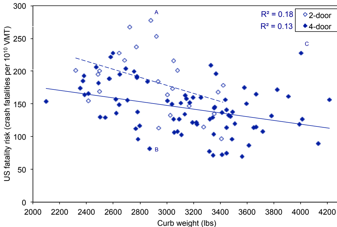
Figure 4.9. US fatality risk per VMT vs. curb weight, car models
