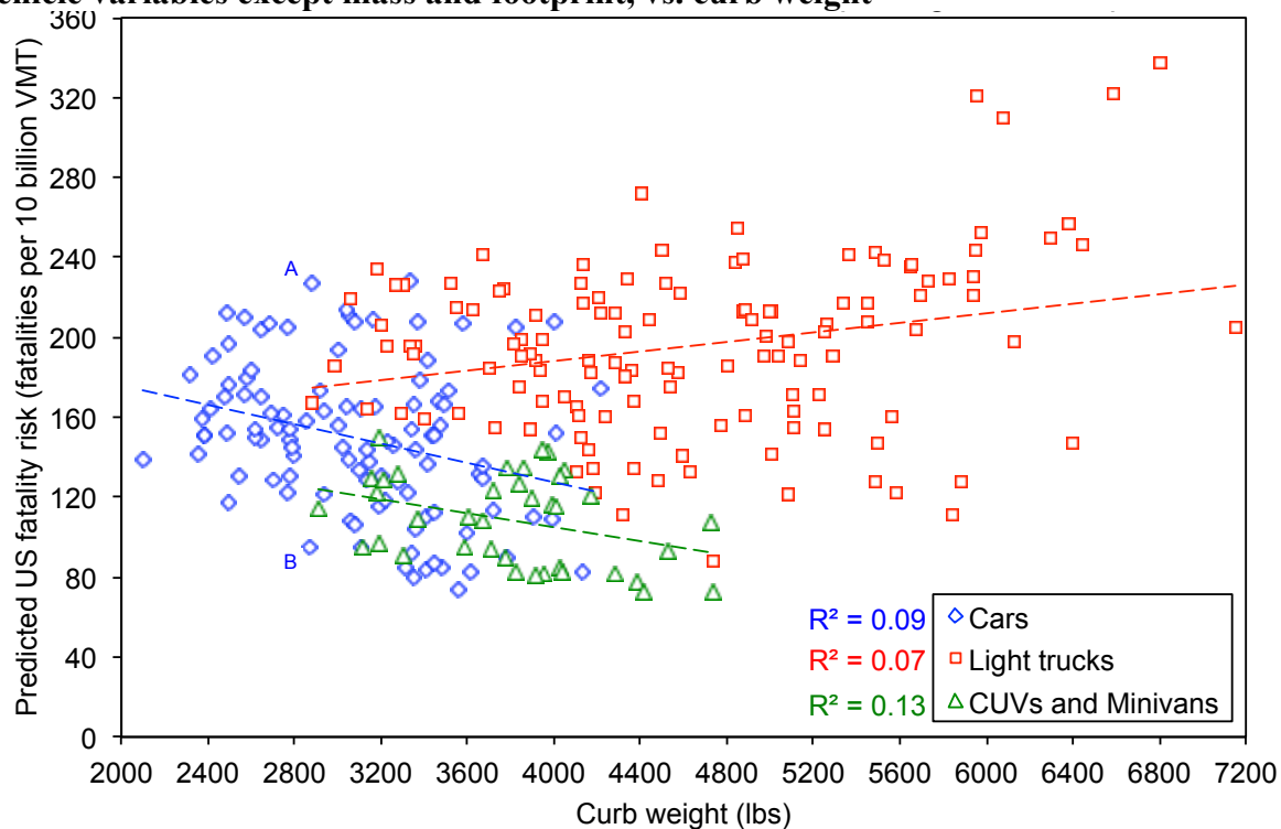
Figure 4.7. Predicted US fatality risk per VMT after accounting for all driver, crash, and vehicle variables except mass and footprint, vs. curb weight
