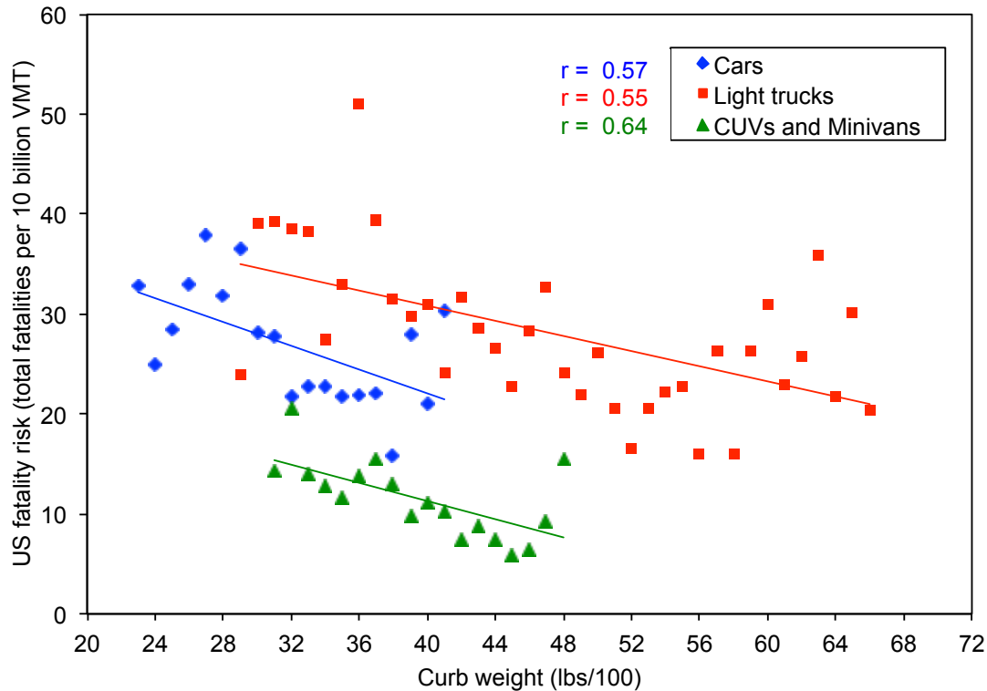
Figure 4.5. Relationship between US fatality risk in crashes with stationary objects and curb weight, by vehicle type
