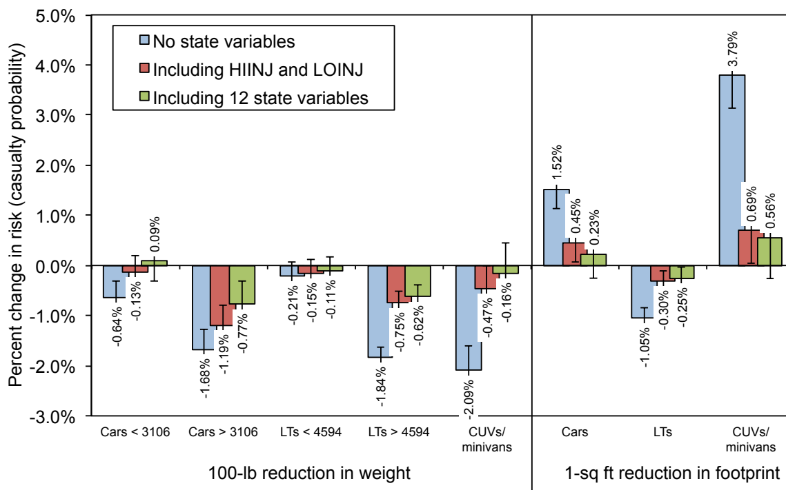
Figure 5.1. Estimated effect of mass or footprint reduction on 13-state casualty risk per crash by vehicle type, under two methods of controlling for the state in which the crash occurred
