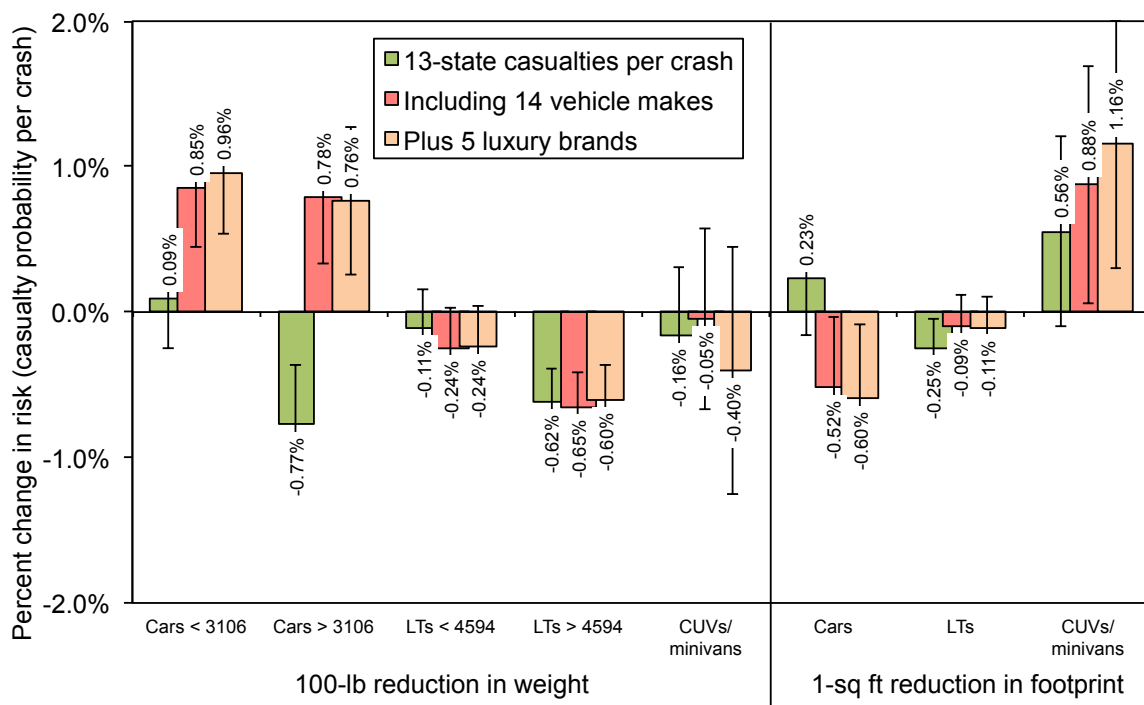
Figure 5.3. Estimated effect of mass or footprint reduction on 13-state casualty risk per crash by vehicle type, after controlling for vehicle manufacturer
