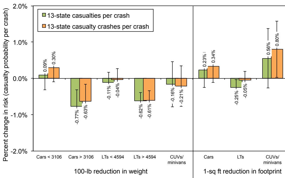
Figure 5.2. Estimated effect of mass or footprint reduction on 13-state casualties and casualty crashes per crash, by vehicle type
