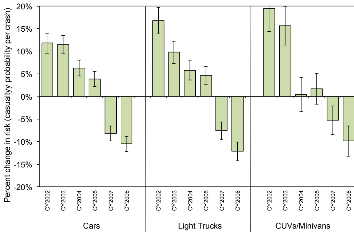
Figure 5.5. Estimated effect of calendar year variables on 13-state casualty risk per crash, by vehicle type
