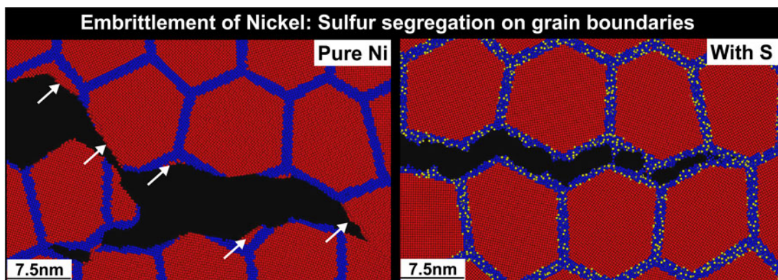
Figure 18. Close-ups of fracture simulations for nanocrystalline nickel without and with amorphous sulfide grain-boundary phases, obtained from a 48-million-atom ReaxFF-MD simulation. Red, blue, and yellow colors represent nickel atoms inside grains ( >0.5 nanometers from grain boundaries), nickel atoms within 0.5 nm from grain boundaries, and sulfur atoms, respectively. The figure shows a transition from ductile, transgranular tearing to brittle, intergranular cleavage. White arrows point to transgranular fracture surfaces. Image courtesy of Priya Vashishta (University of Southern California).
