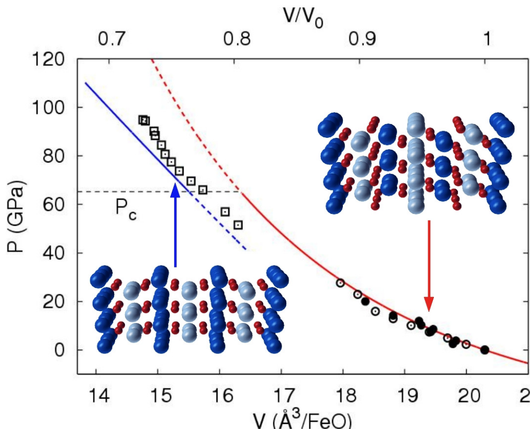
Figure 12. Equation of state (pressure versus volume) of FeO at low temperatures. The QMC results for the transition pressure, P_c = 65\text{--}70 GPa, is in close agreement with experimental measurements that vary between 70 and 100 GPa. The upper-right corner shows antiferromagnetic rocksalt equilibrium structure while the lower-left corner illustrates the high-pressure tetragonal structure. Image courtesy of Jindrich Kolorenč and Lubos Mitás (North Carolina State University). (Source: Kolorenč and Mitás 2008).
