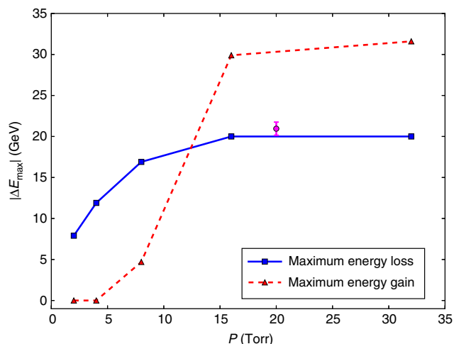
Figure 5 | Energy gain and loss in simulations. The red triangles (blue squares) represent the maximum energy gain (maximum energy loss) observed at the end of the beam-plasma interaction in QuickPIC simulations (see the Methods for details) for different argon pressures. The magenta circle and its error bar represent the experimental average maximum energy gain corresponding to the data of Fig. 2 and its s.e.m.
