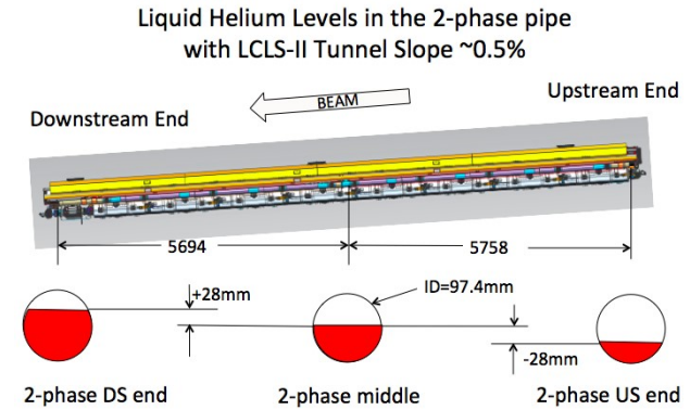
Figure 3: Liquid levels in the 2-phase pipe with 0.5% SLAC tunnel slope, with pipe sized to accommodate liquid levels both downstream and upstream (US) [2].
