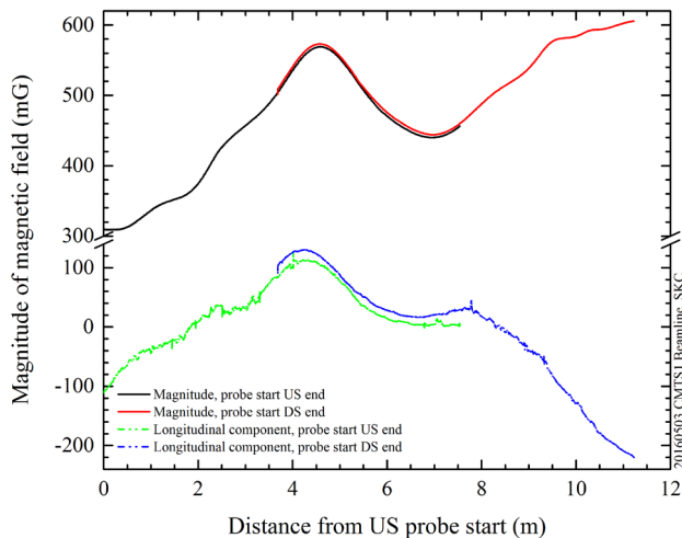
Figure 4: The measured magnetic field, magnitude (solid lines) and longitudinal component (dash-dot lines), along the beamline in CMTS-1.
