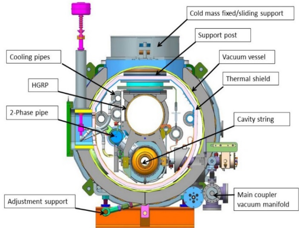
Figure 1: Cross-section of the cryomodule showing its major sub-assemblies [2].
